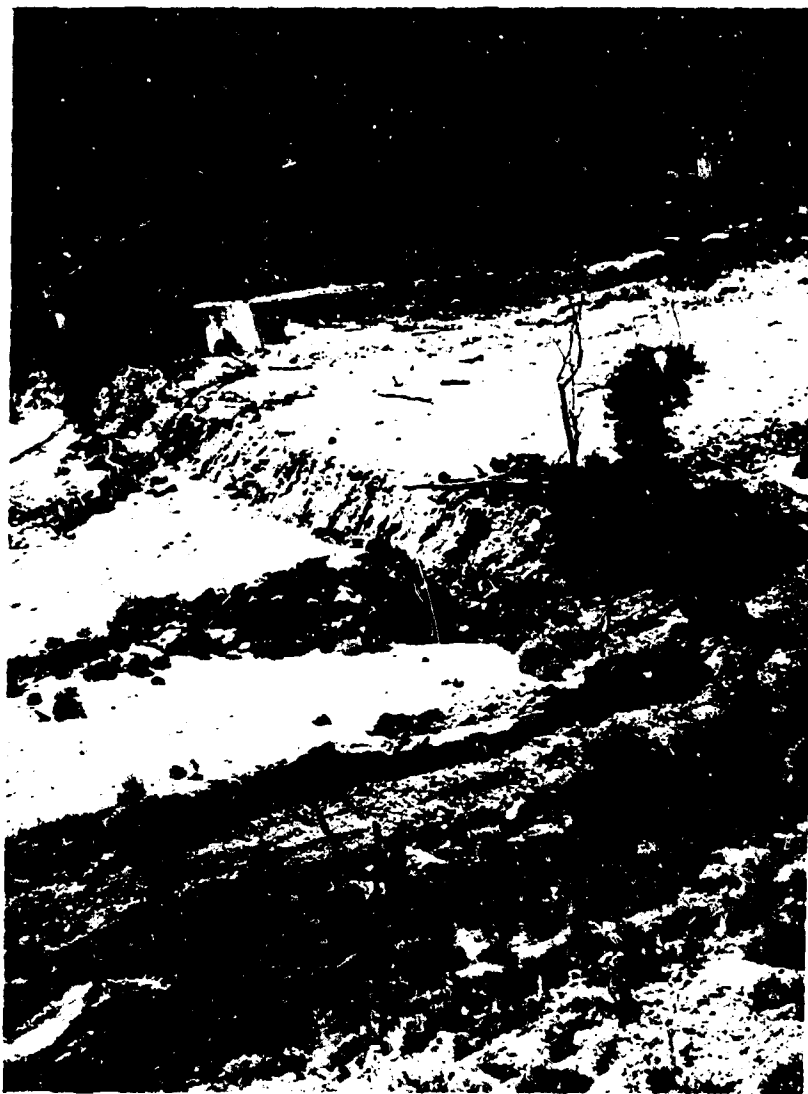
Figure 54. Pipeline intake reservoir in lower Leidy Creek Canyon filled and partly destroyed by flood of July 1967.
