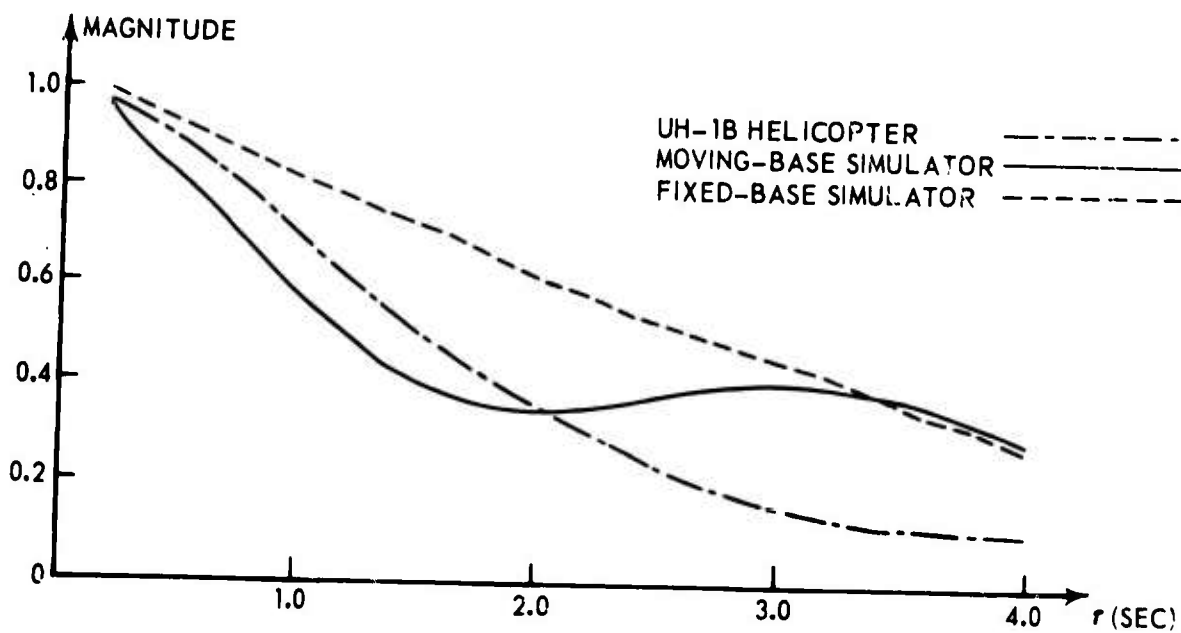
Figure 32. ACF of the Pitch Attitude for the 70-Knot Descent.
