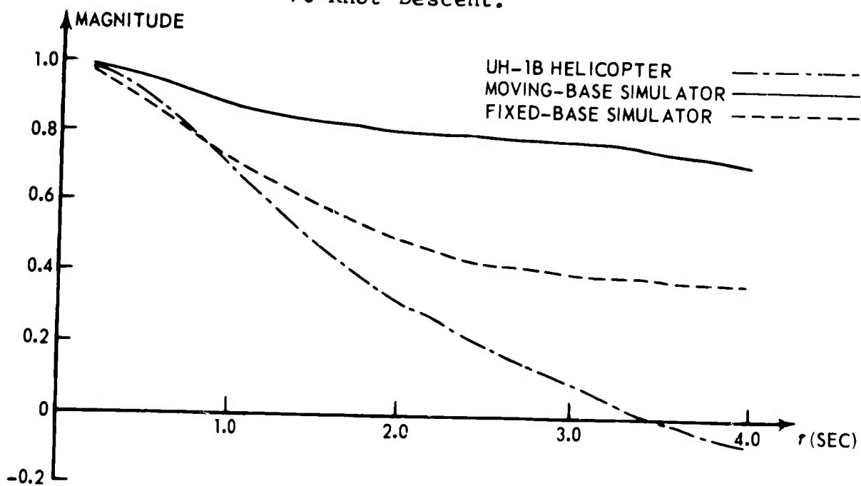
Figure 33. ACF of the Pitch Attitude for the Landing Approach.
