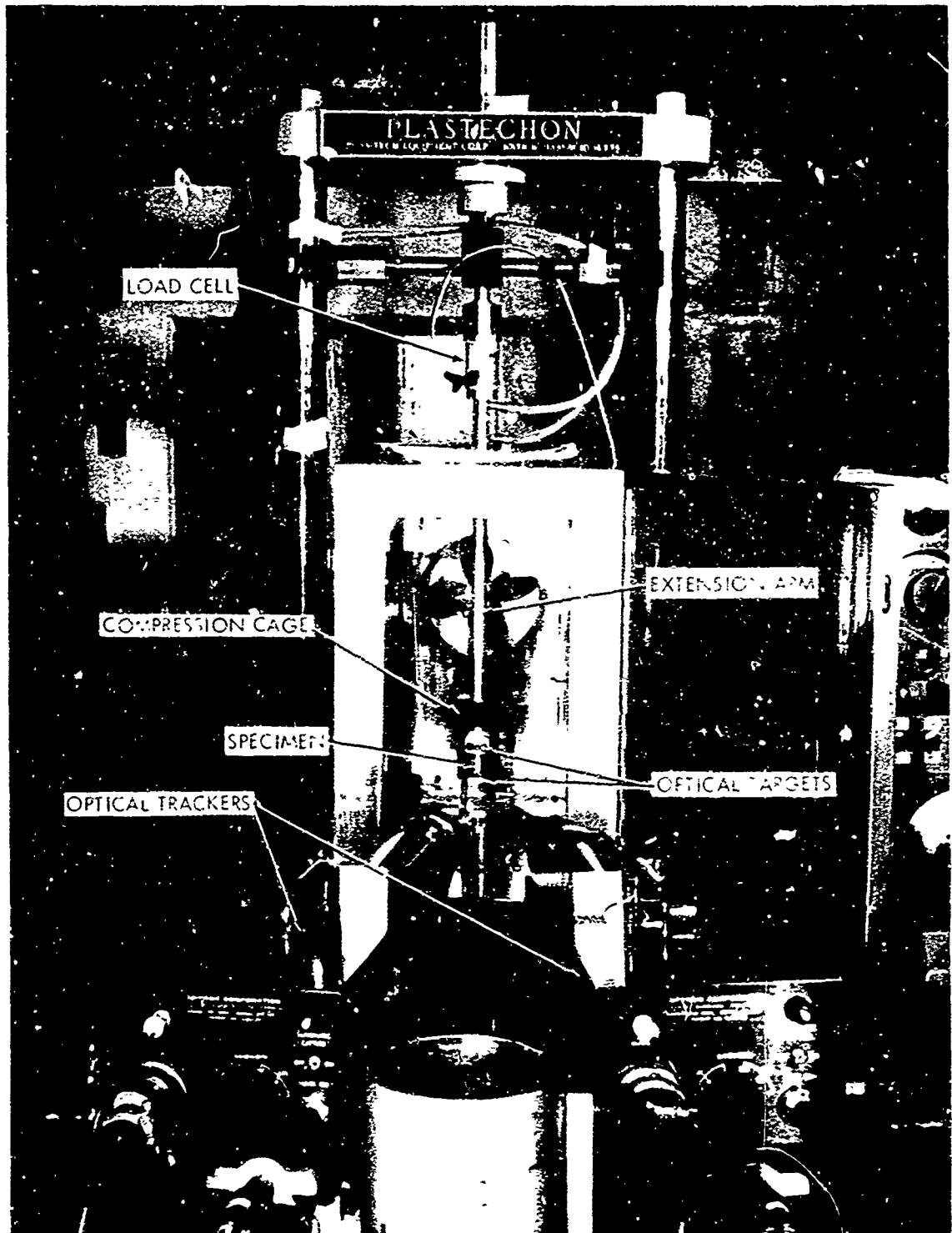
FIG. 13. MEDIUM RATE TESTING APPARATUS
