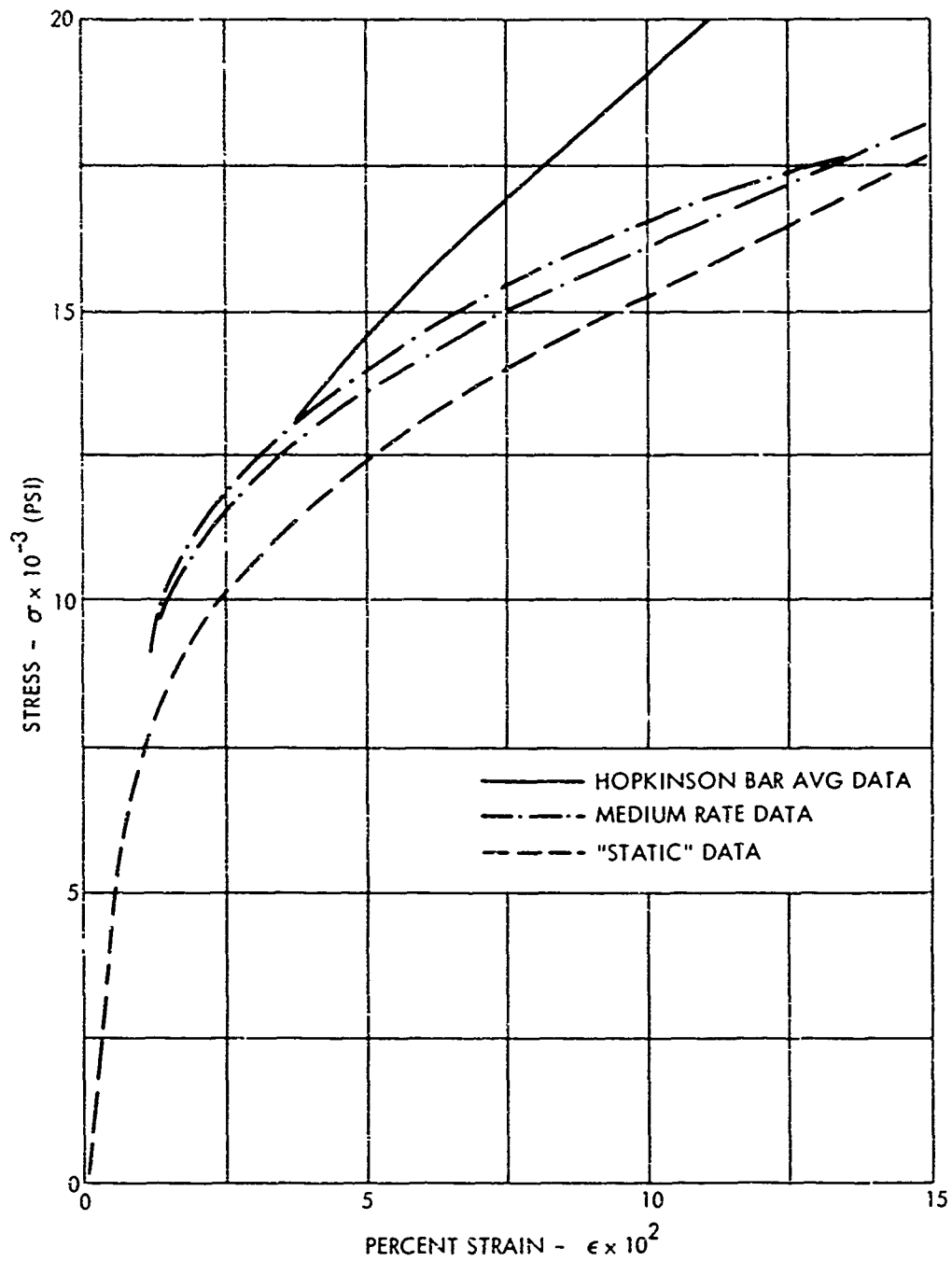
FIG. 20 VARIOUS OBSERVED BEHAVIOR OF COMMERCIALLY PURE ALUMINUM
