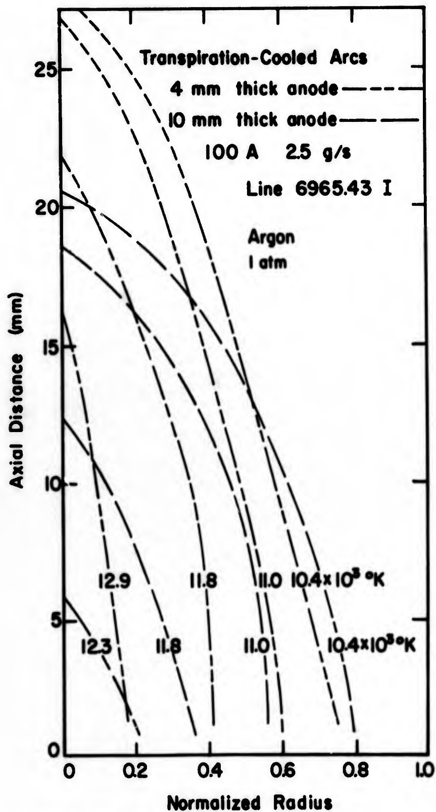
FIG. 35 Isotherms of Transpiration-Cooled Arcs
