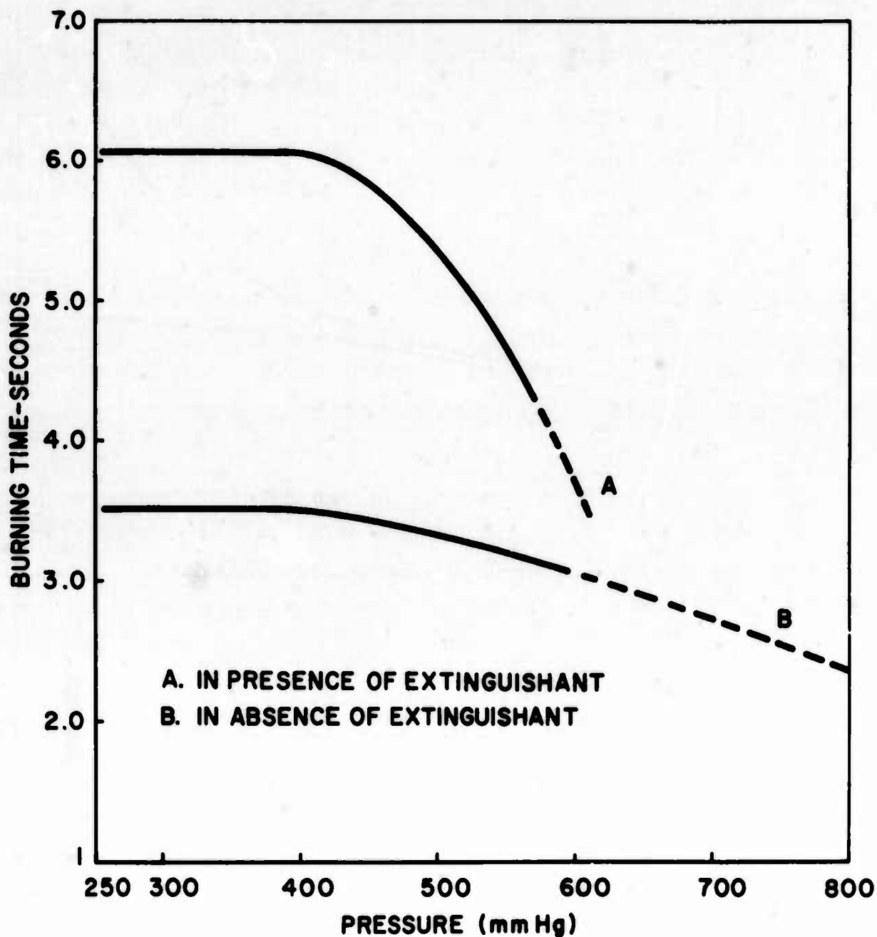
FIGURE 15. Combustion Behavior of Dacron Fabric in Initially 100% Oxygen Atmospheres at One Gravity:- Effect of \text{CF}_3\text{Br} Extinguishant.
