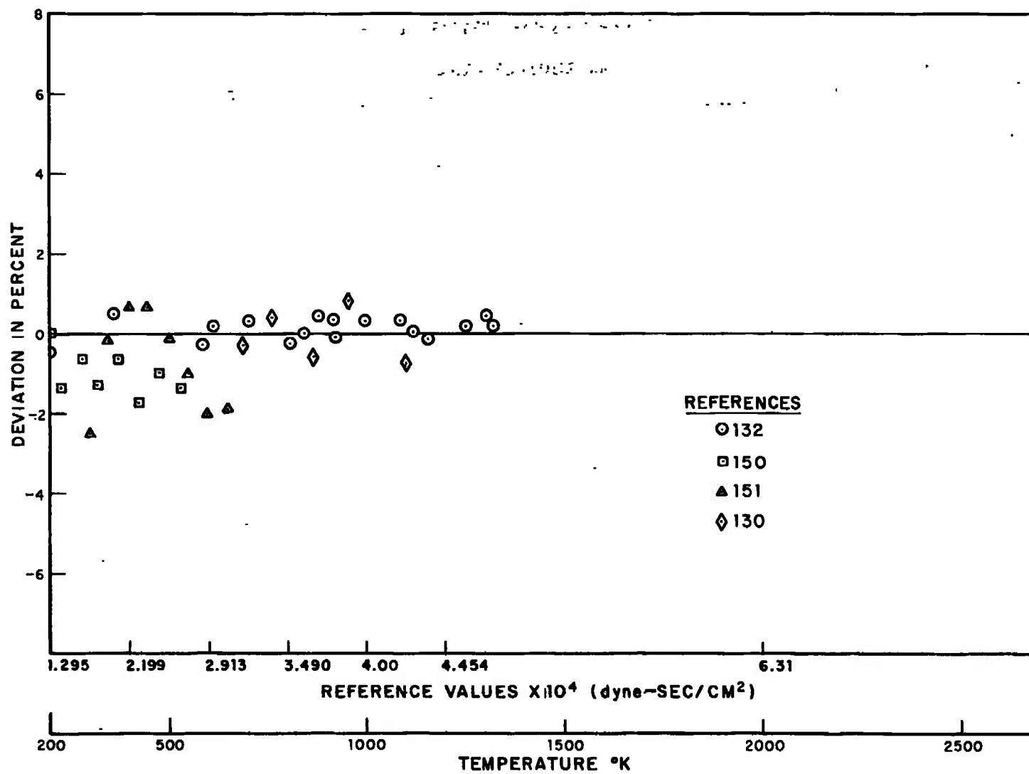
Fig. 14 Viscosity deviation chart for nitrogen
