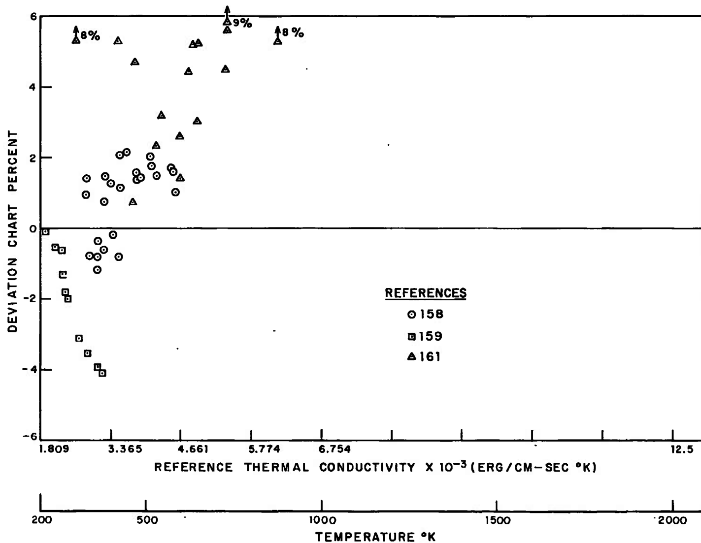
Fig. 21 Thermal conductivity deviation chart for air
