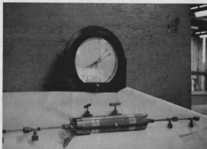
Fig. 32 Test chamber for high pressure sound speed measurements
