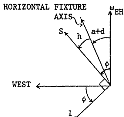
FIGURE 3 LABORATORY ORIENTATION OF THE GYROSCOPE
