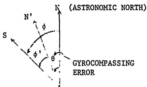
FIGURE 2 MINIMUM PRECESSION (General Case)
