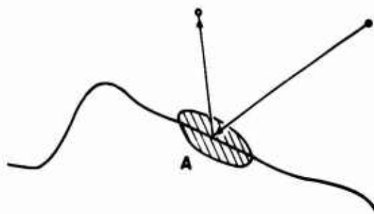
Fig. 8. Smooth bottom over A, the illuminated area.
