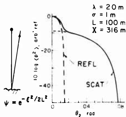
Fig. 17. Scattered and reflected sound. The surface spectrum is \Psi_1 .
