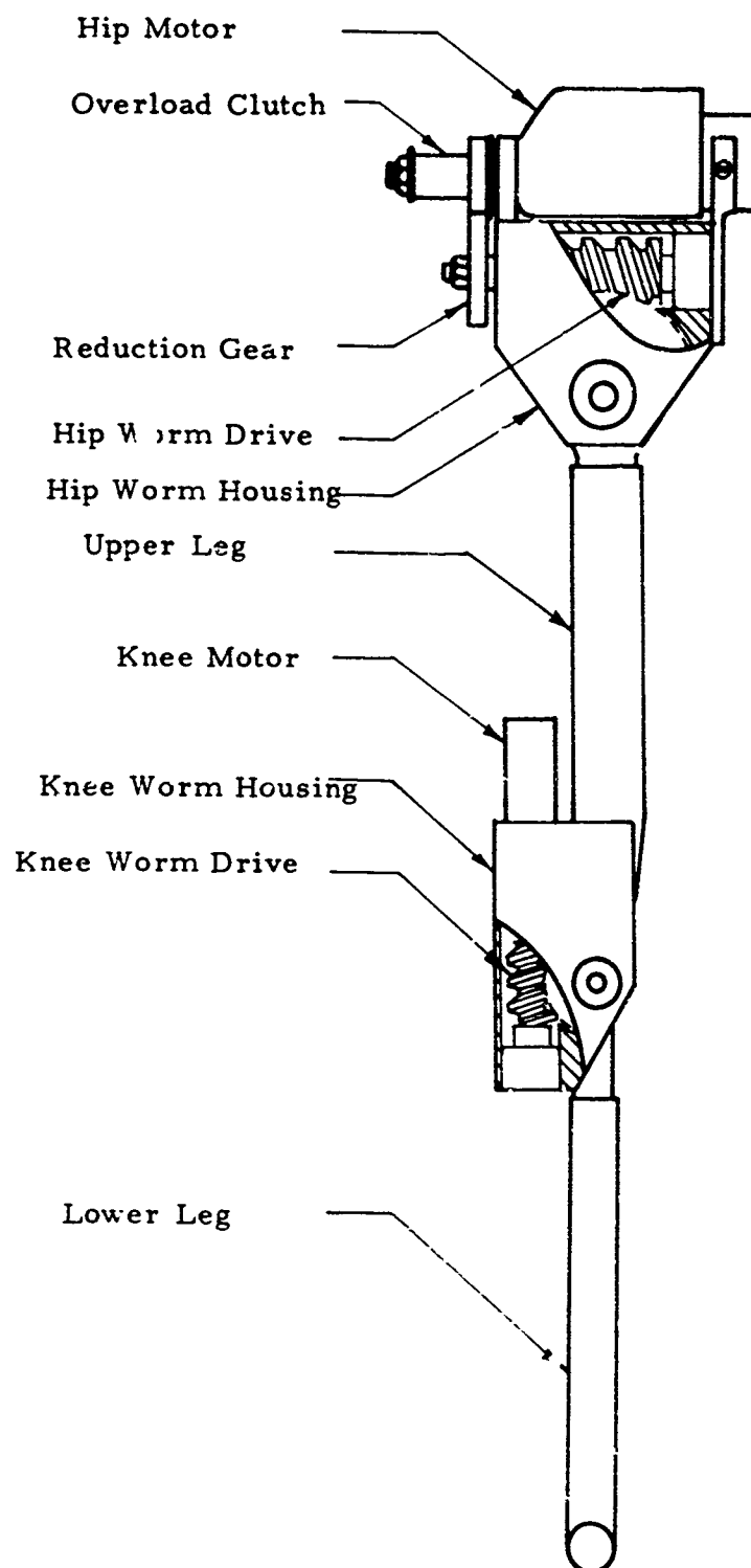
Leg Mechanism
