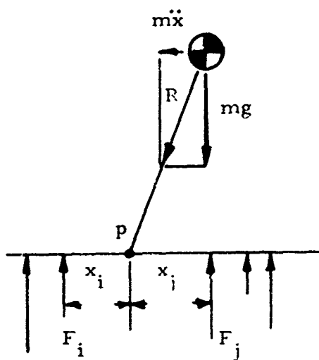
Moment plane normal to reaction force R
