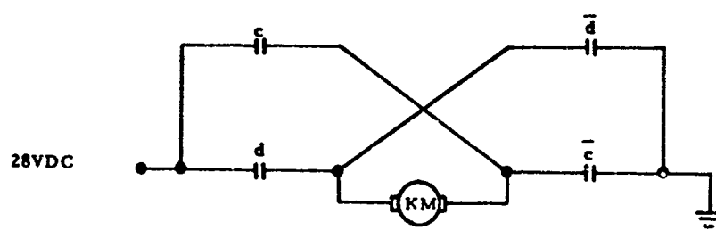
(b) Knee Motor Drive Circuit
