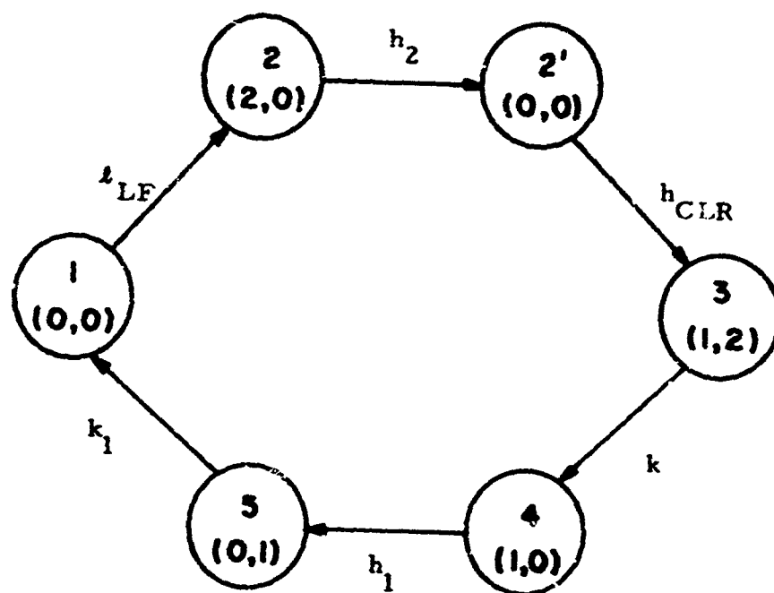
Trot Leg Control State Diagram
