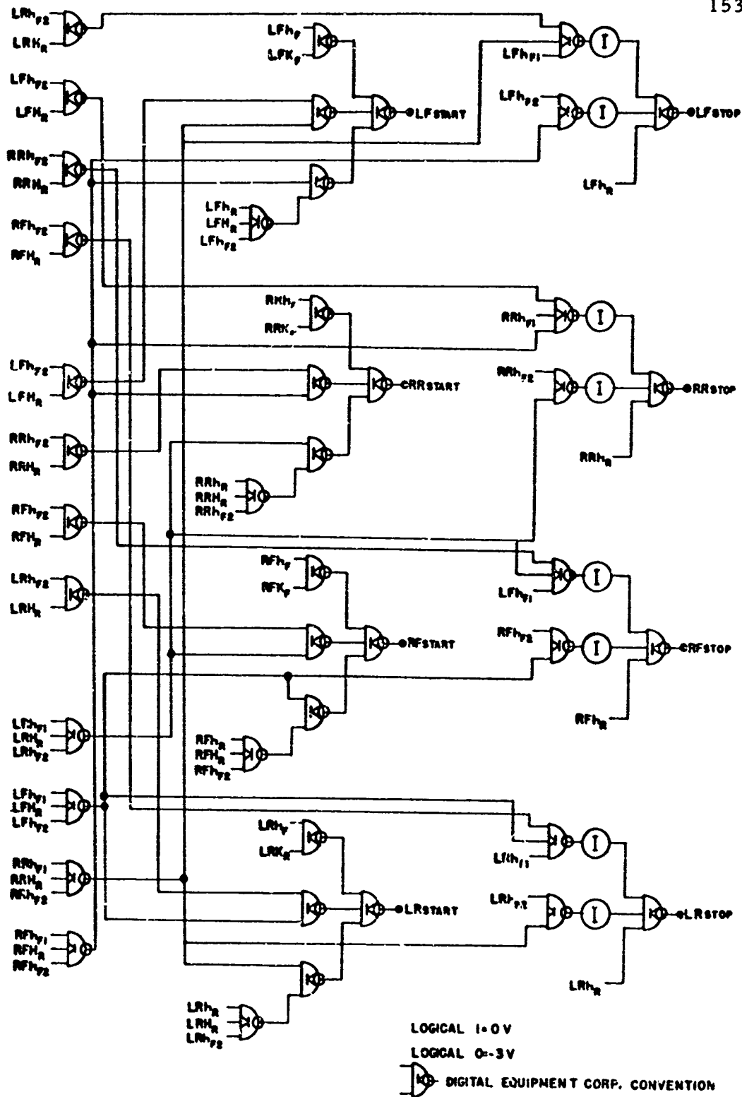
Start - Stop Logic Circuit Figure 6
