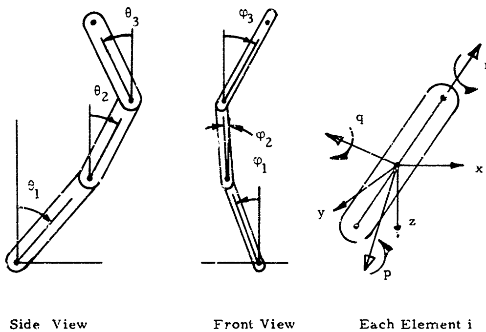
The Parameters of Leg Analysis Figure 3.2
