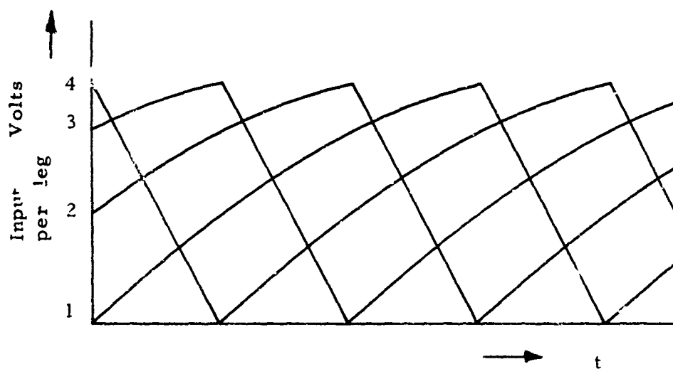
Coordinated Leg Commands
