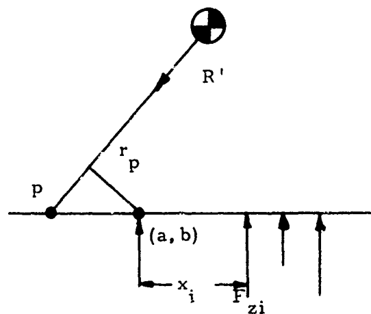
The Projection of R Into A Plane Normal To Line (a, b)
