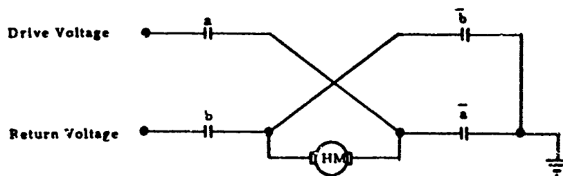
(a) Hip Motor Drive Circuit
