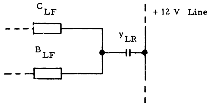
(a) Leg Return Interrupt Circuit
