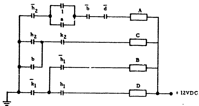
(c) Relay Monostable Leg Logic
