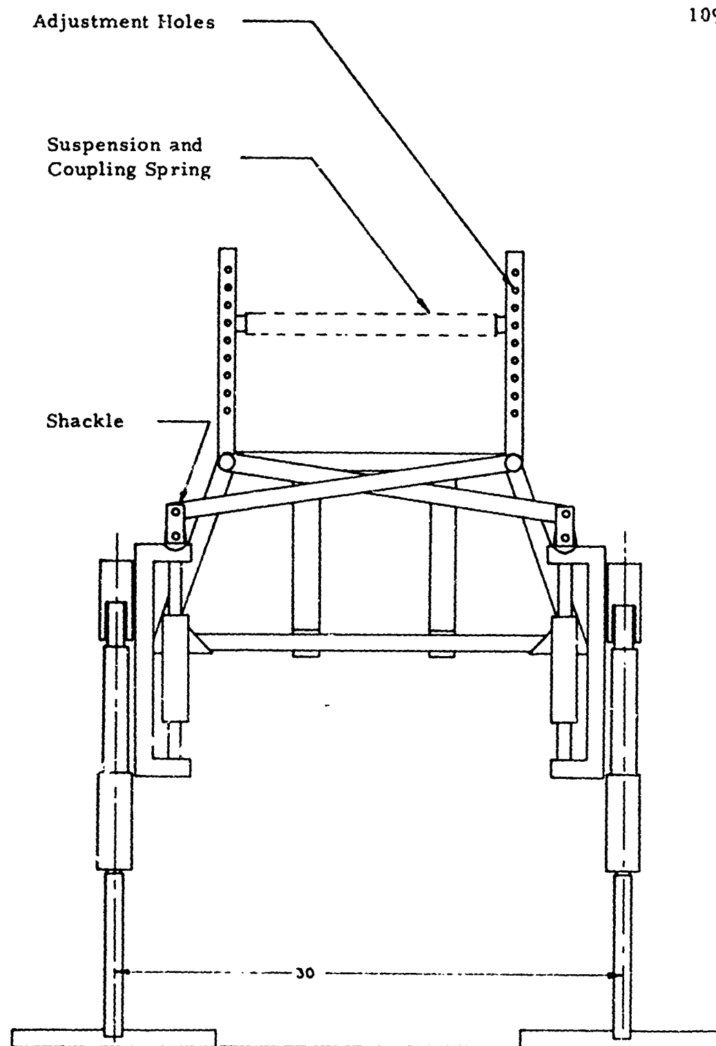
Leg-Pelvic Arrangement for the Designed Quadruped Figure 4.2
