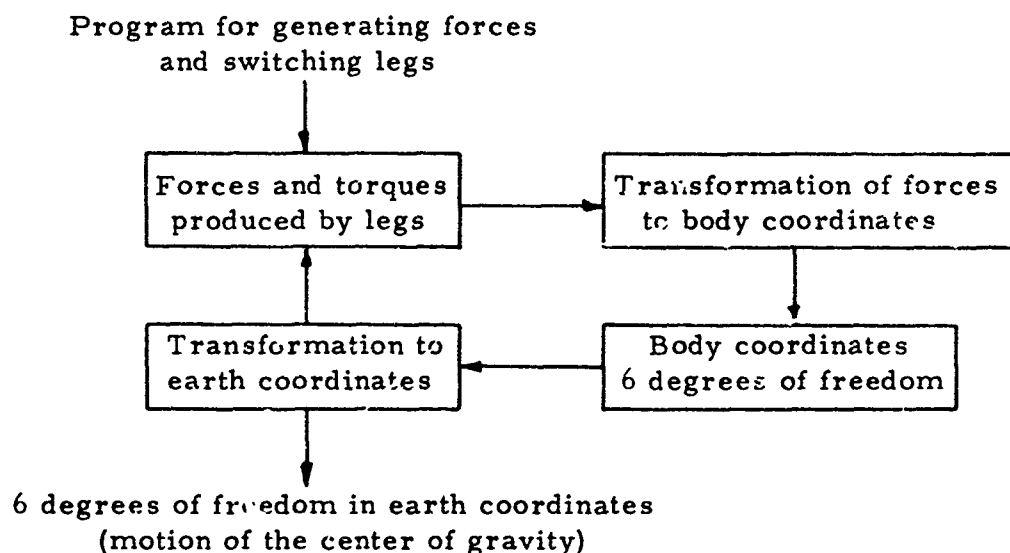
Block Diagram for Computation of Legged Machine Motions Figure 3.5
