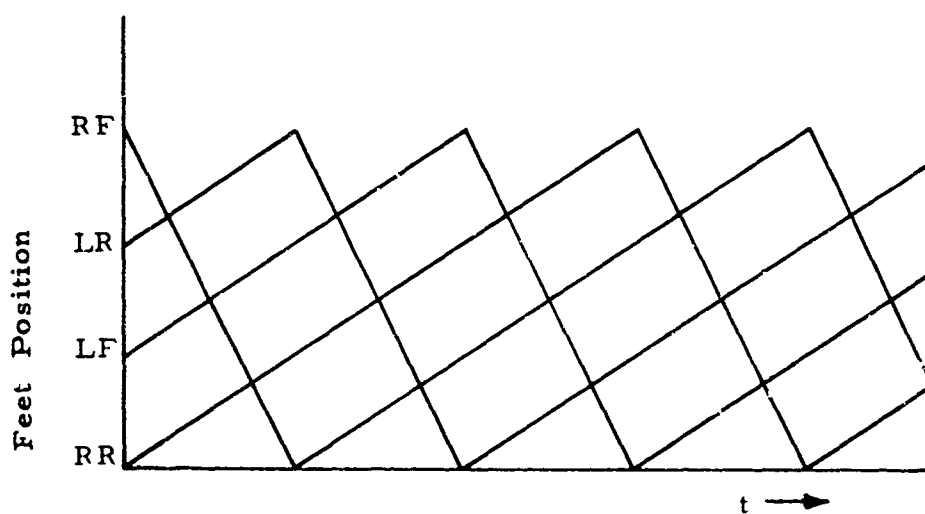
Ideal Feet Position - Time Trajectory For A Quadruped
