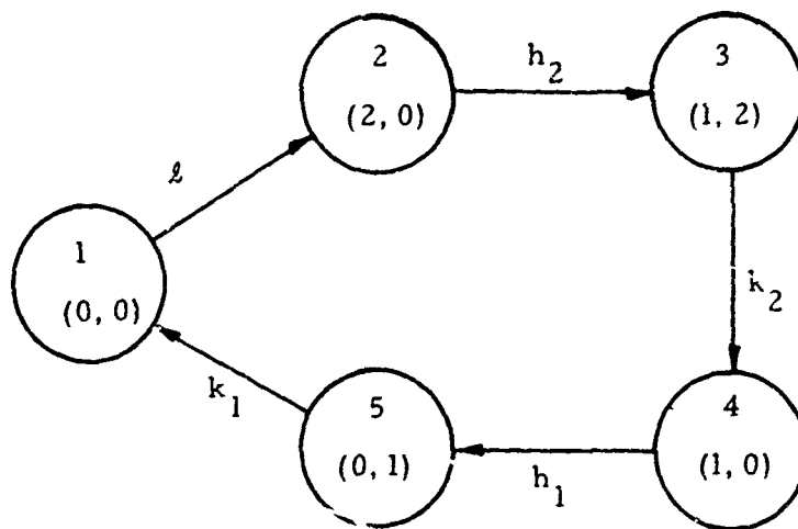
(a) State Diagram For Monostable Leg Sequence
