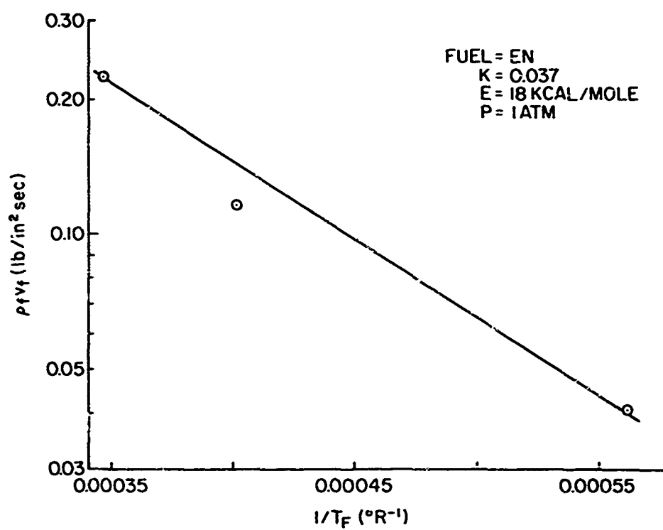
Figure 4.10 Activation Energy for EN
