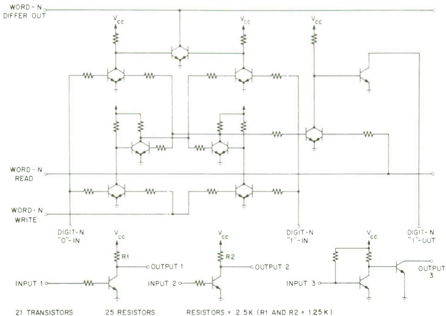
Figure 13. Schematic diagram of 1-Bit, 1-Word Associative Memory Cell (including drive circuitry).
