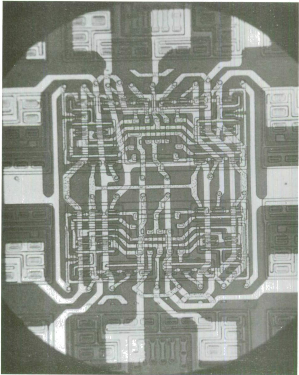
Figure 4. Photomicrograph of 3-Bit Parity Array.
