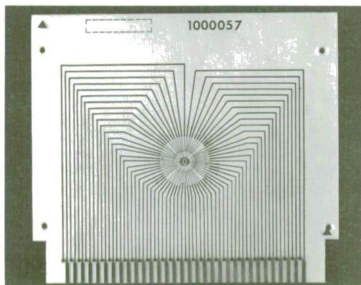
Figure 17. Fifty-nine pin micro test probe.
