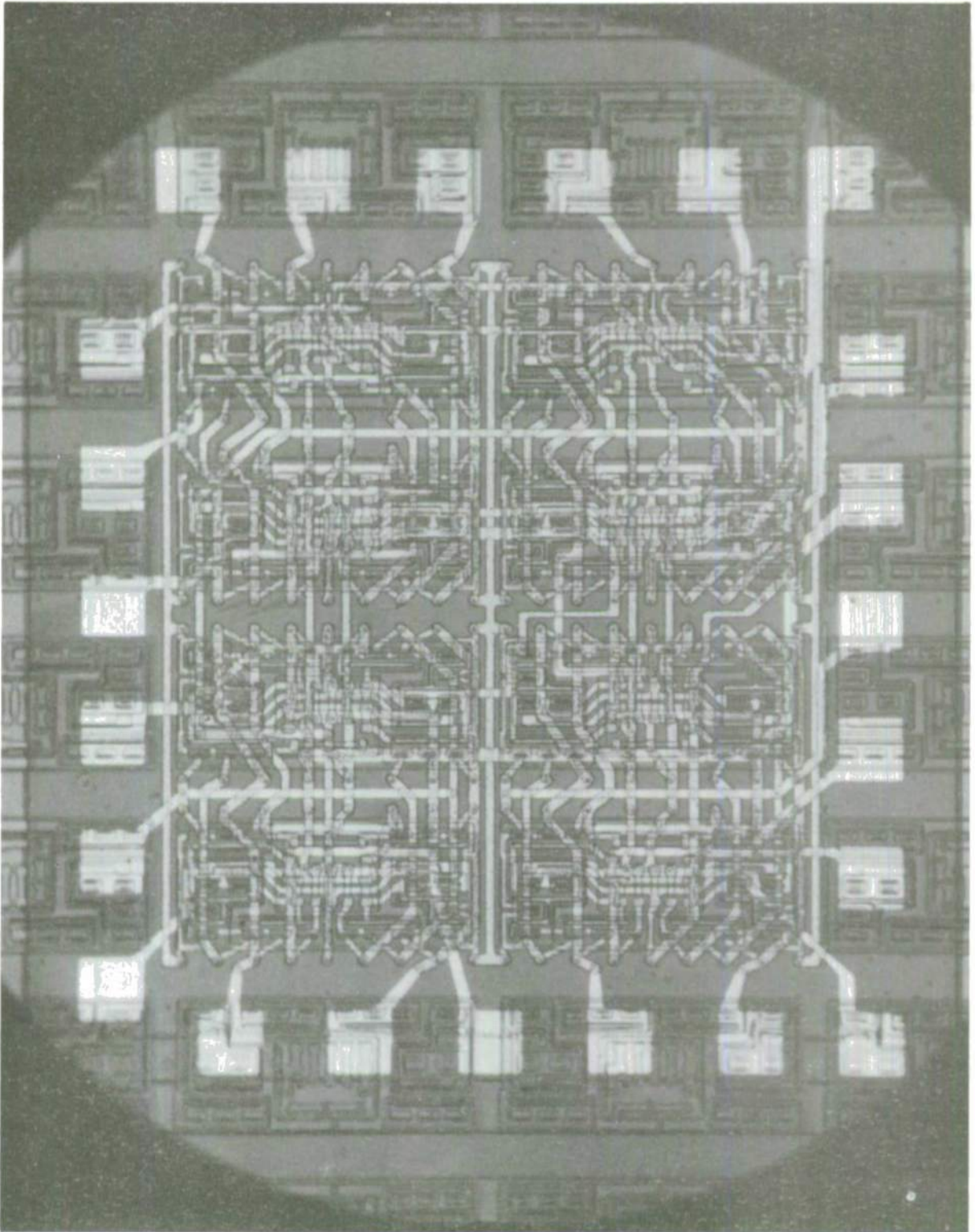
Figure 8. Photomicrograph of 9-Bit Parity Array.
