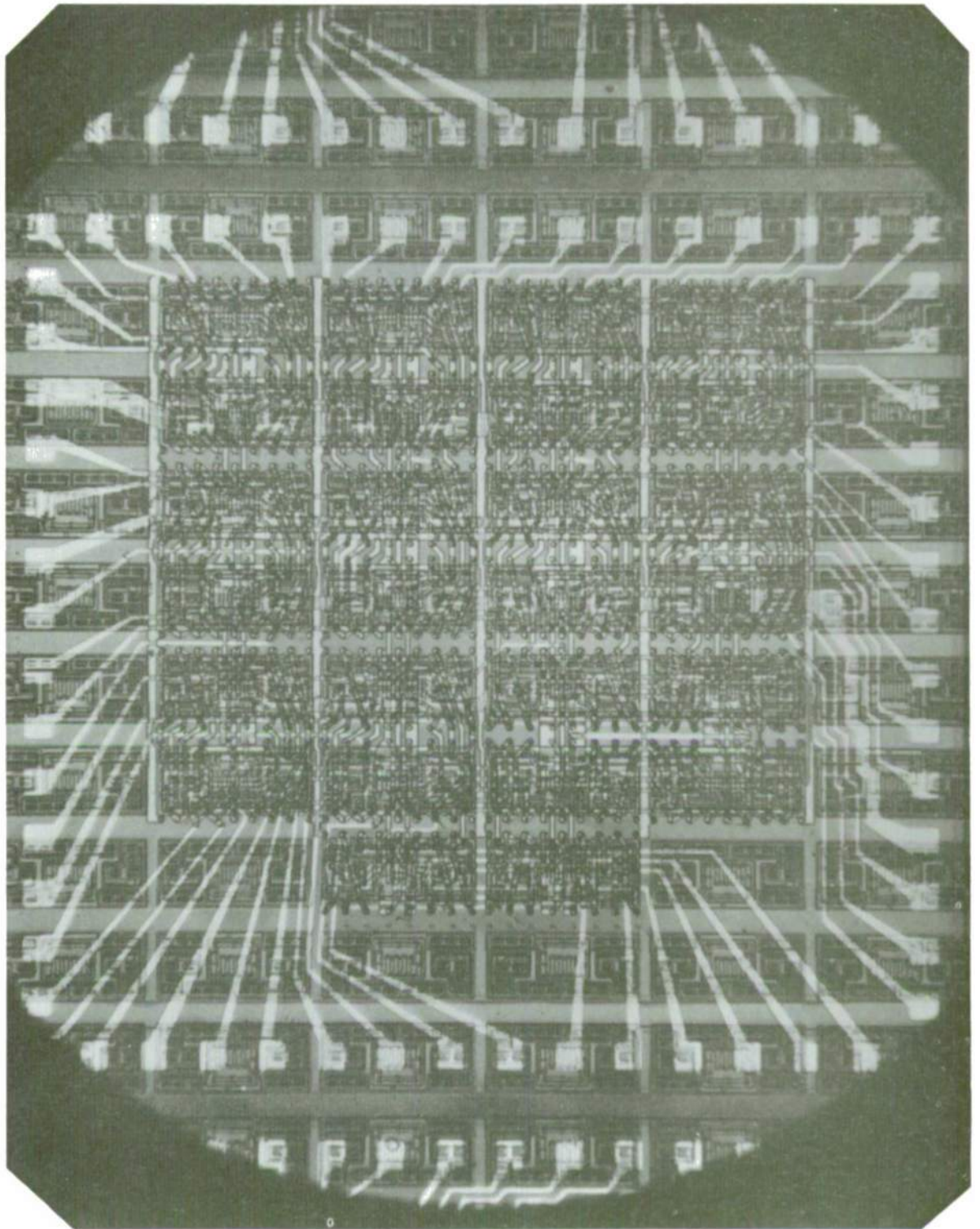
Figure 9. Photomicrograph of 27-Bit Parity Array.
