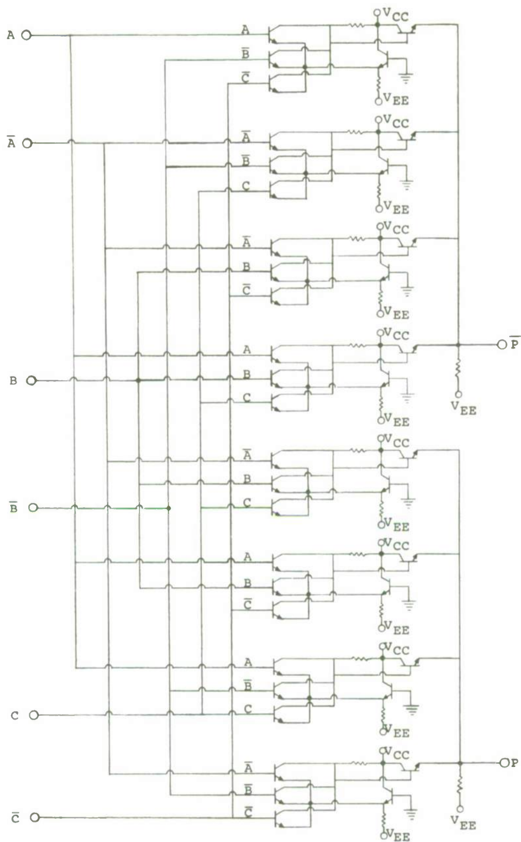
Figure 5. Schematic diagram of 3-Bit Parity Array.
