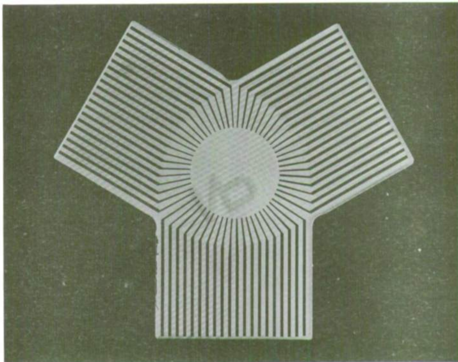
Figure 15. Experimental printed circuit test board for 60-lead package shown in Figure 14.
