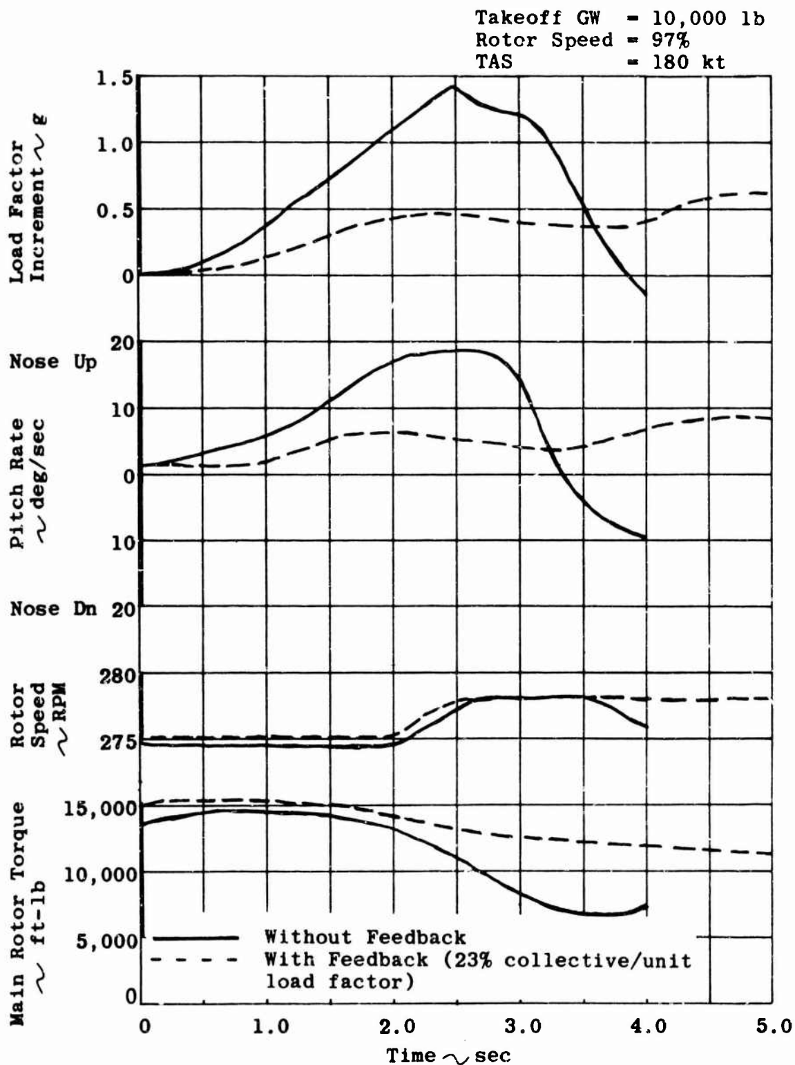
Figure 10. Influence of Feedback on Aircraft Maneuver Stability.
