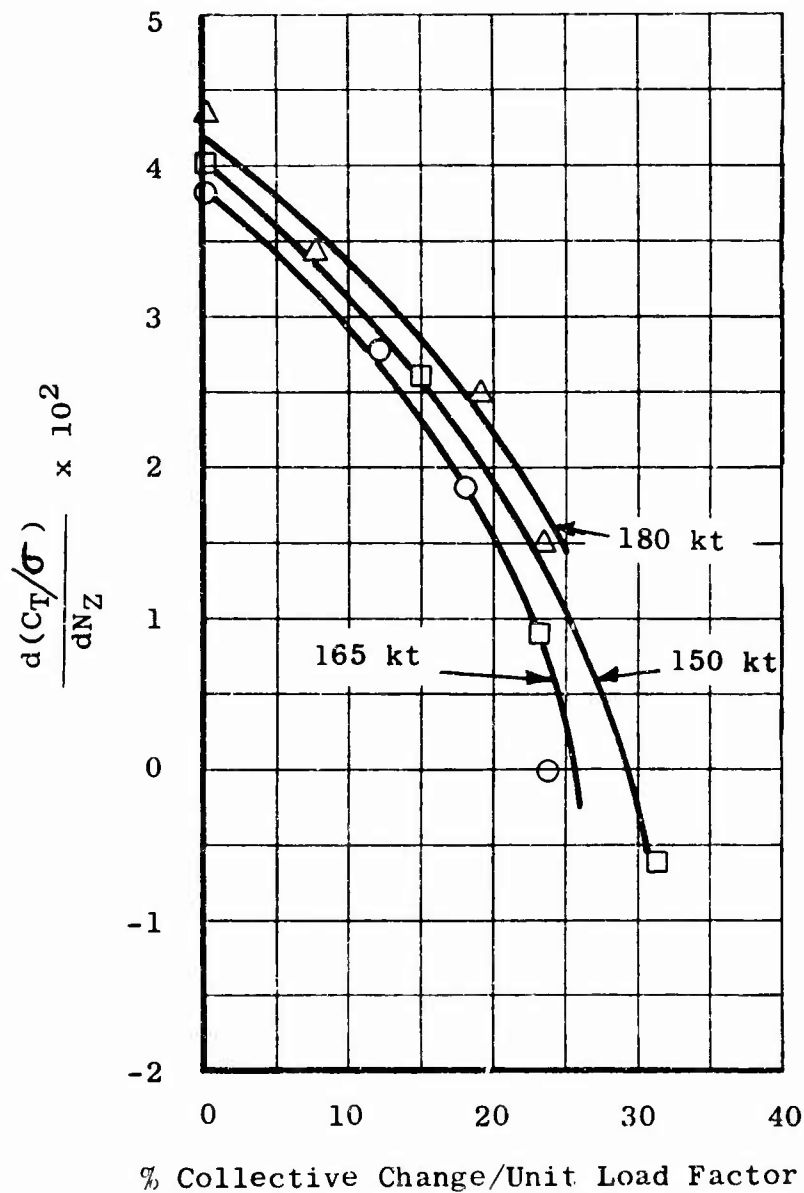
Figure 5. Effect of Collective Pitch Reduction on Rotor Blade Loading Change With Normal Load Factor.
