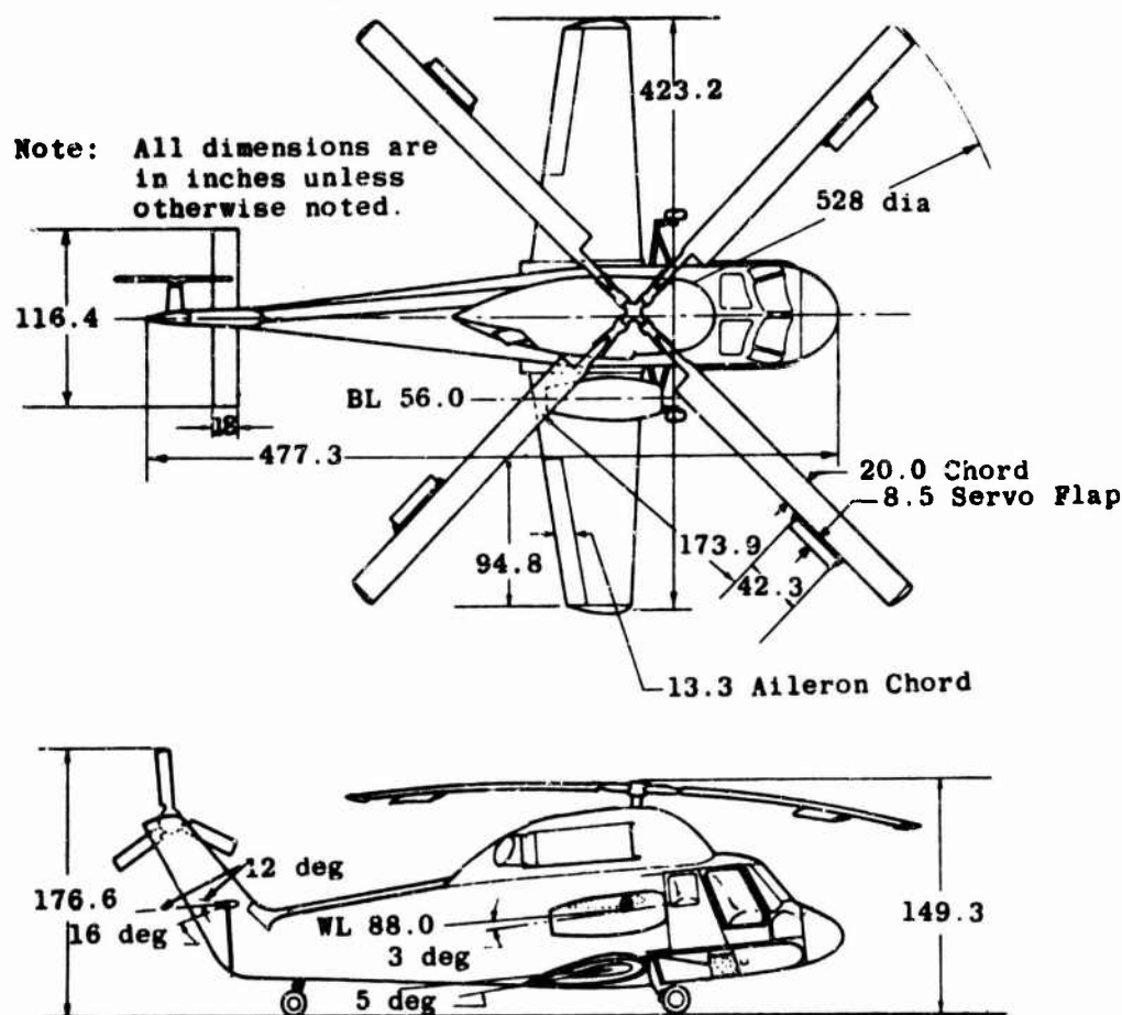
Figure 2. General Arrangement - UH-2 Compound Helicopter.
