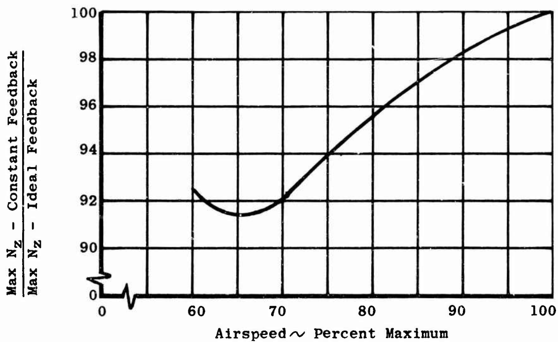
Figure 9. Penalty Imposed by Constant Collective Feedback.
