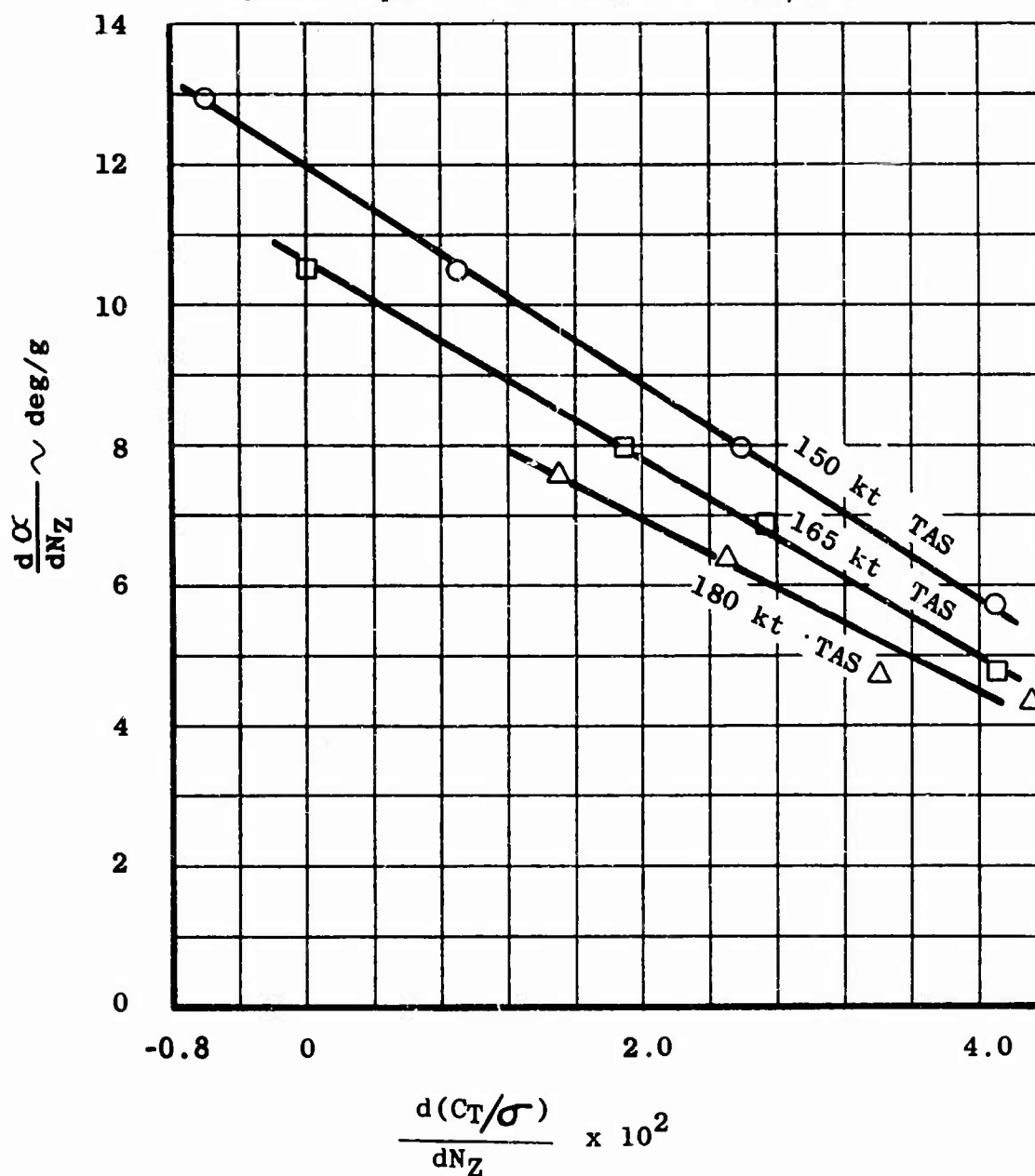
Figure 8. Effect of Rotor Blade Loading Change on Wing Angle of Attack in Accelerated Maneuvers.
