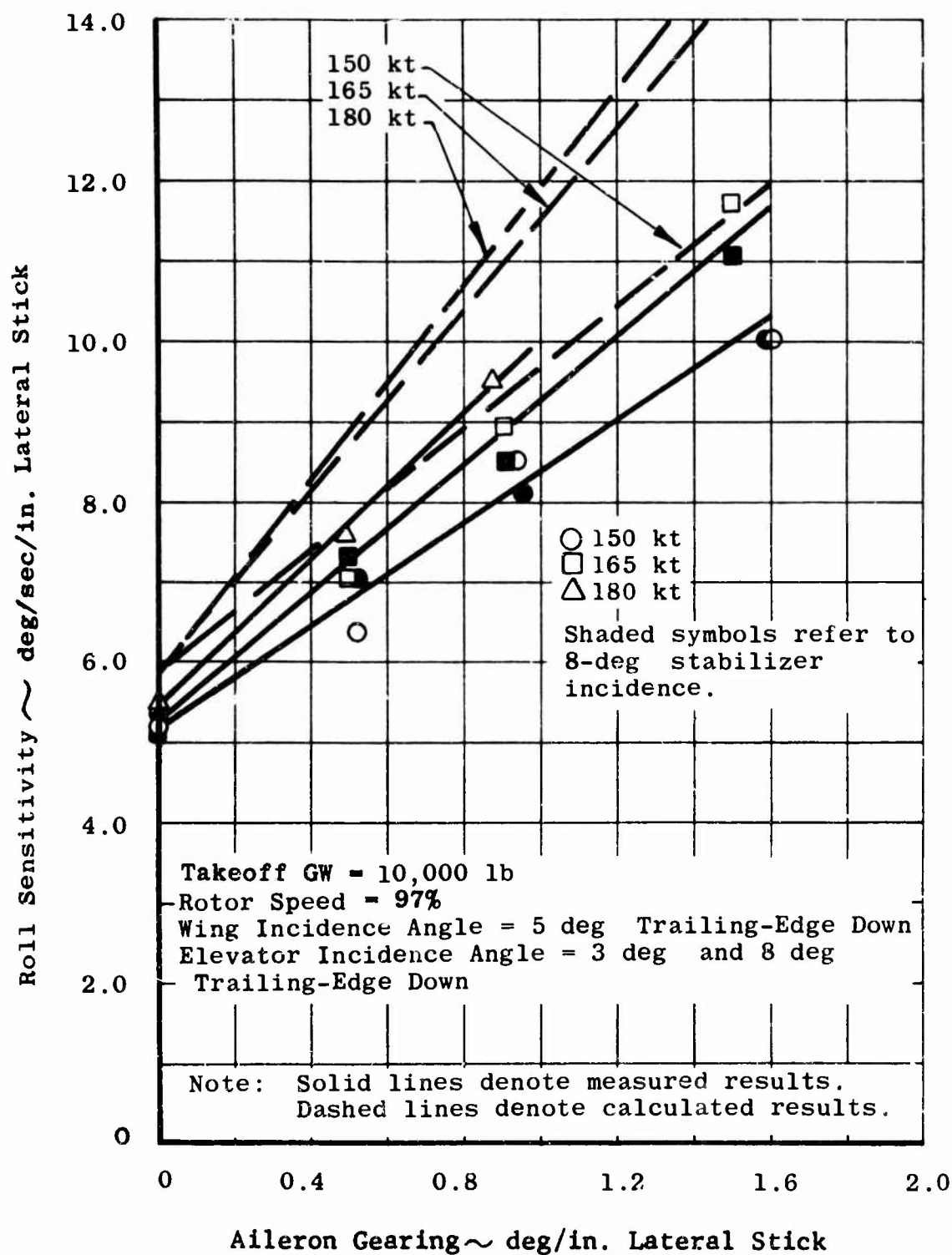
Figure 6. Variation of Roll Rate Sensitivity with Roll Control Augmentation.
