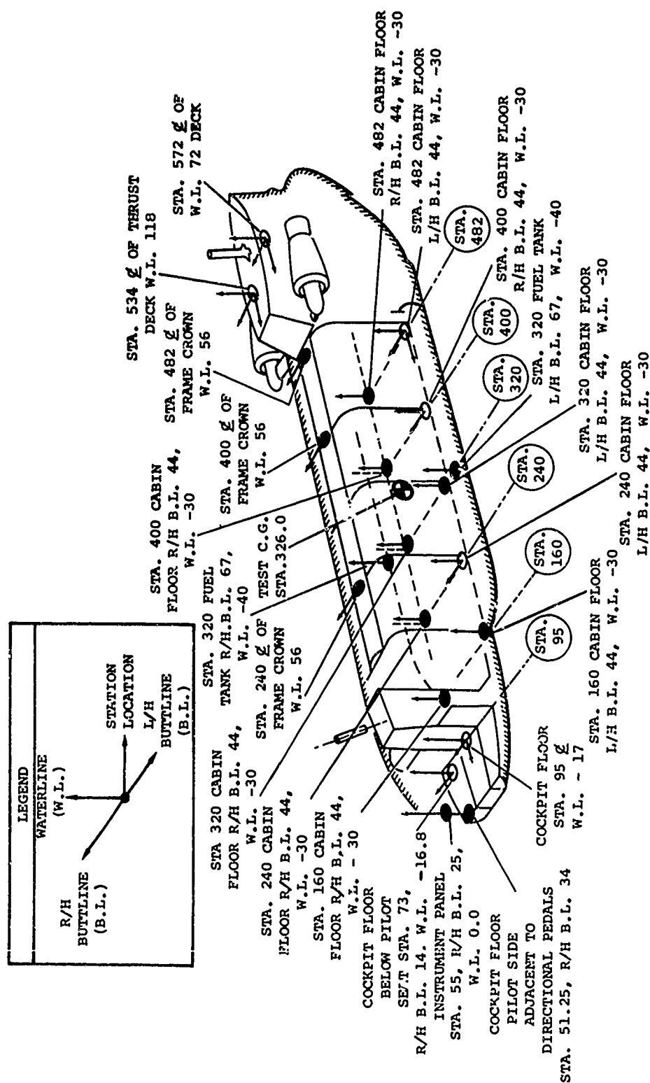
Figure 23. Location and Orientation of Fuselage Response Accelerometers.
