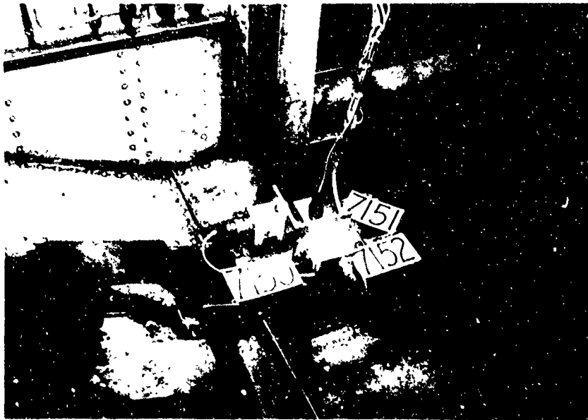
Figure 24. Typical Fuselage Accelerometer Installation.
