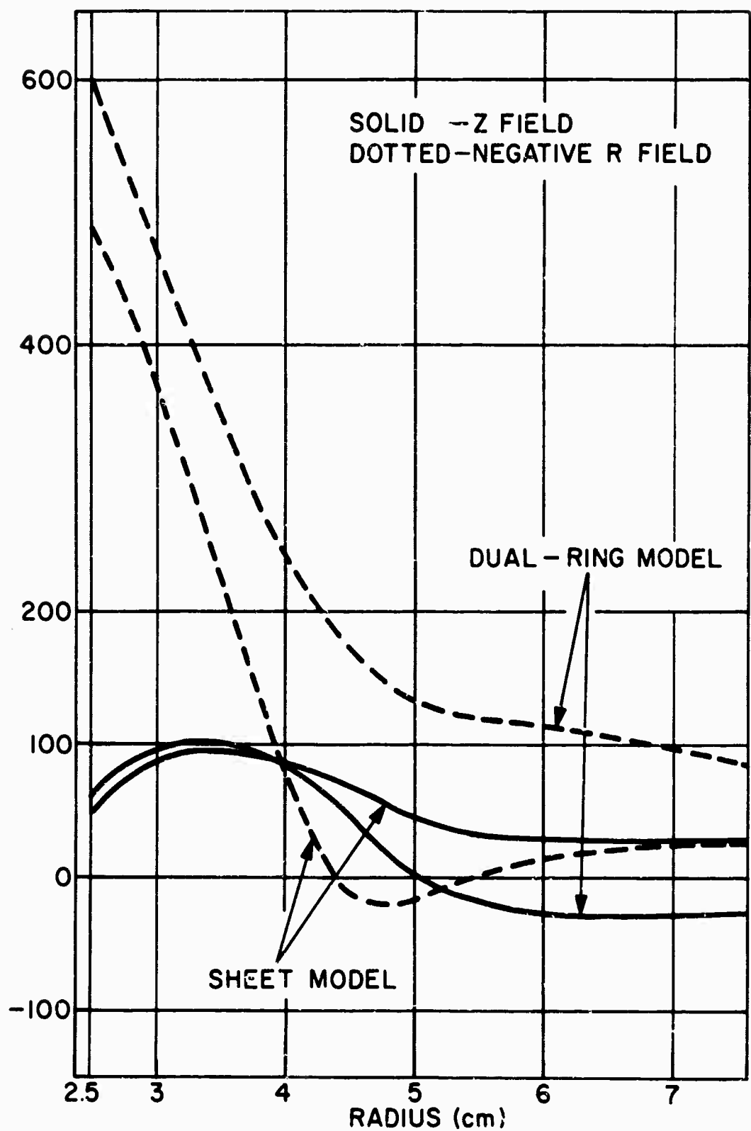
Model Fields (Side Wall)
