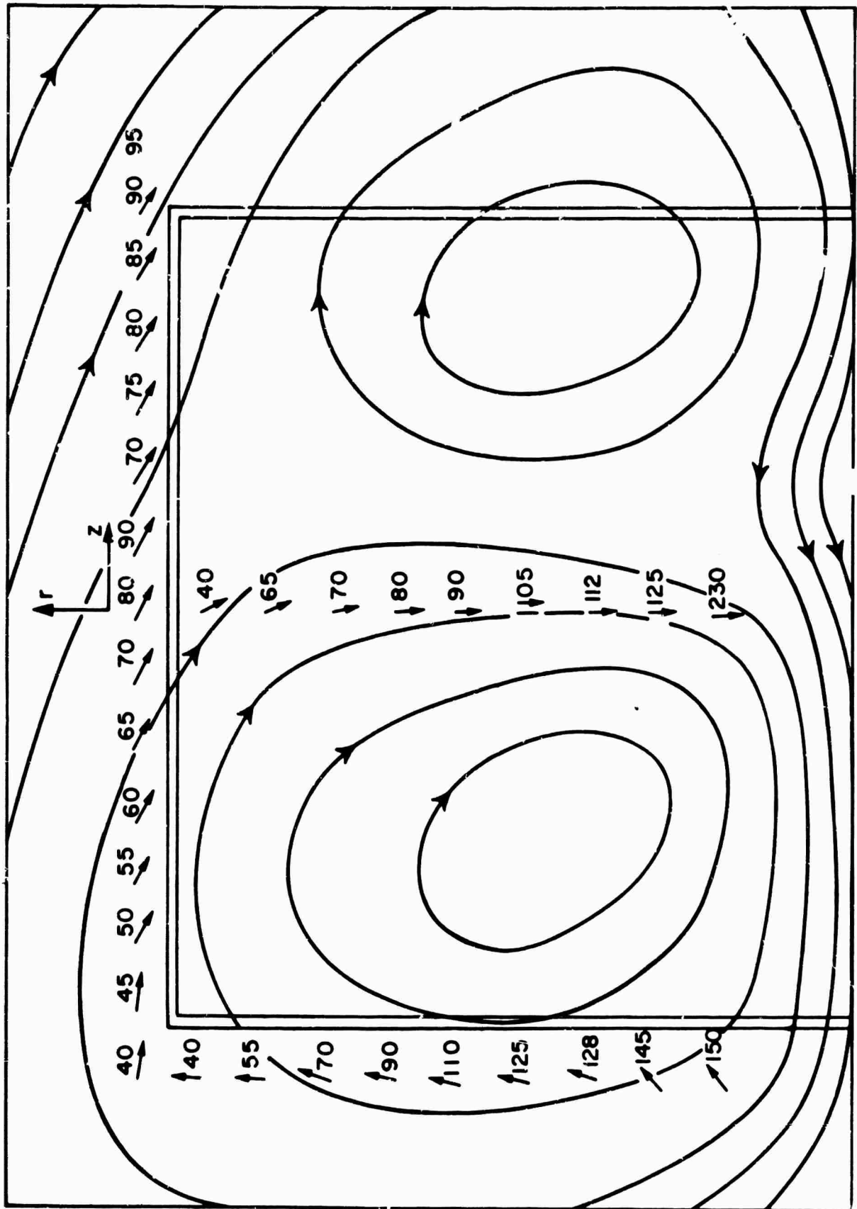
Magnetic Flux Plot - Time Four Microseconds
