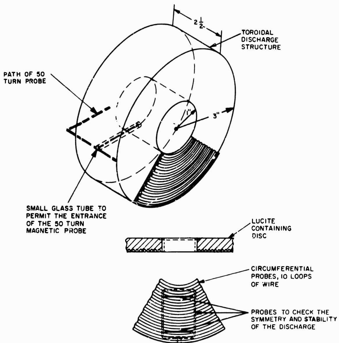
Stationary Magnetic Probes
