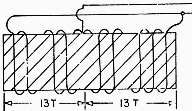
WINDING FOR THREE PLASMA RINGS
