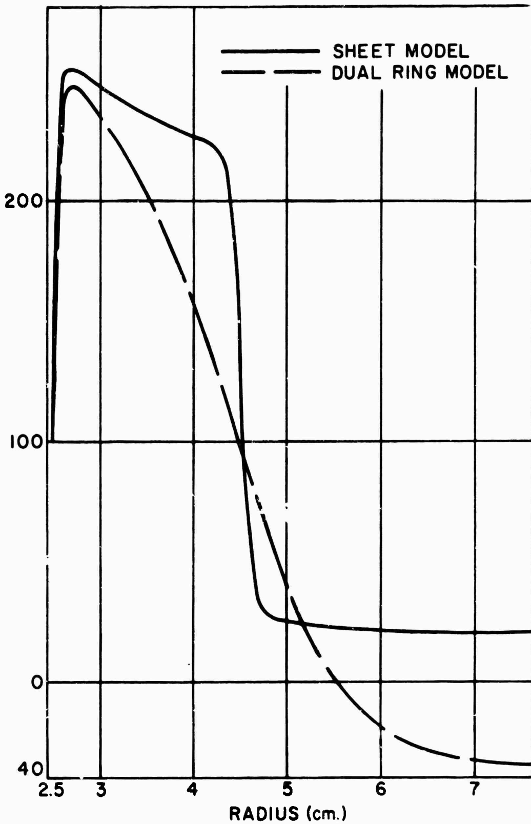
Model Fields for B_z (Center of Discharge) Figure V-11
