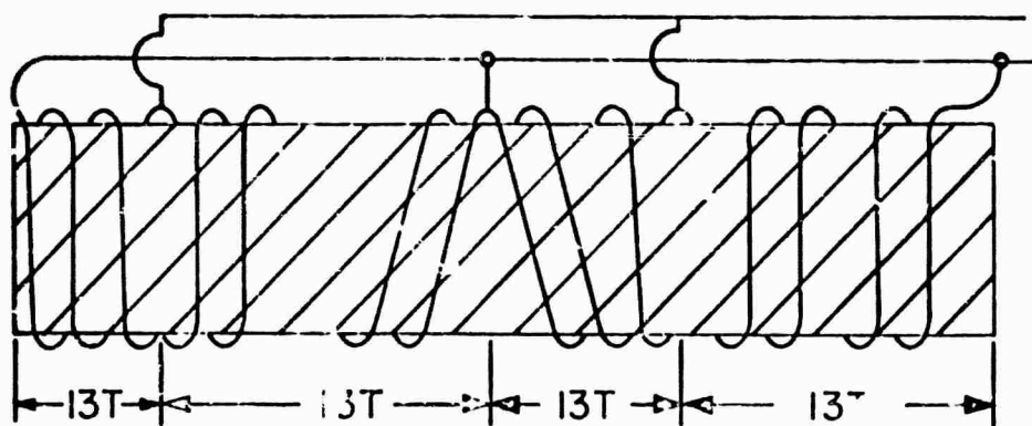
WINDING FOR FIVE PLASMA RINGS
