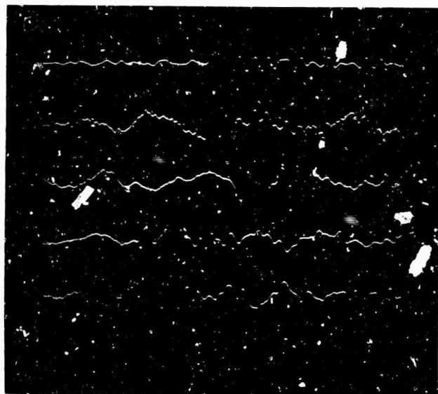
Fig. 7b. Top trace is Butterworth filtered. Second trace; raw data.
