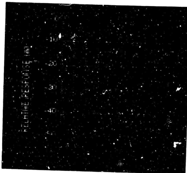
Fig. 8b. Periodogram of the bottom trace of Fig. 8a.
