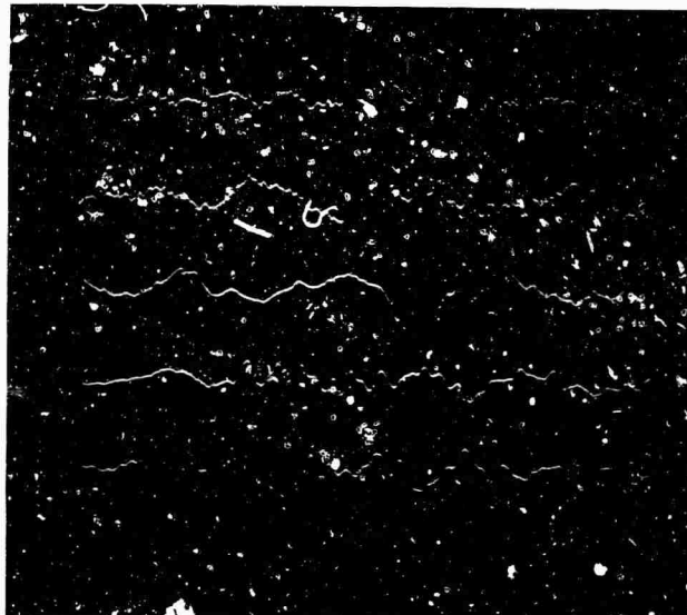
Fig. 7a. Top trace is notch filtered. Second trace; raw data.
