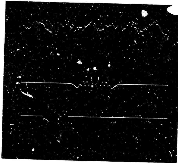
Fig. 8a. Top trace is input data. At the bottom, a certain portion is selected with the light pen. The middle trace is the autocorrelation function of the bottom trace.
