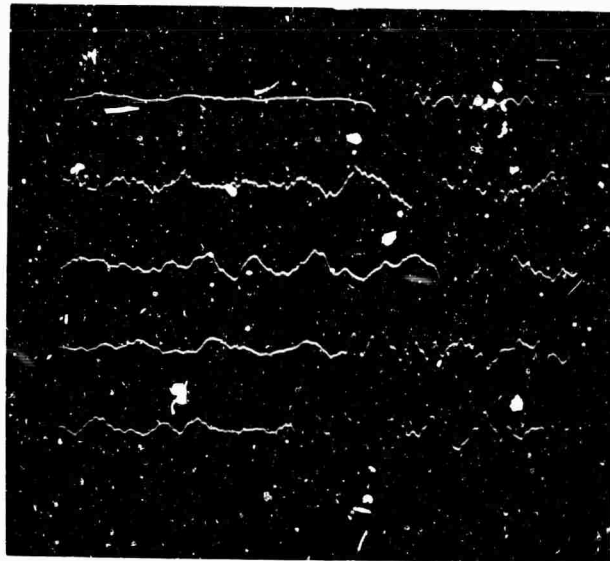
Fig. 5. Beam formed from all 21 seismograms at top. Notice improved S/N.
