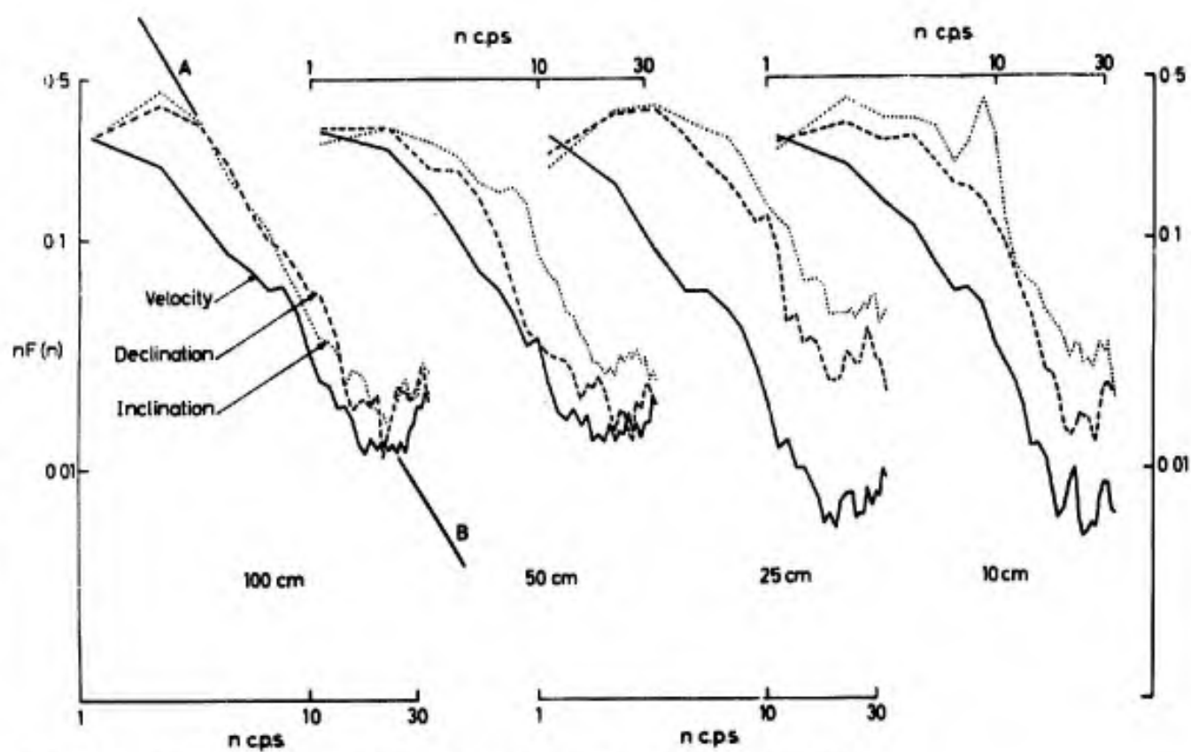
Fig.2.25. Mean energy spectra from 3 samples taken during hours 1945-2200
