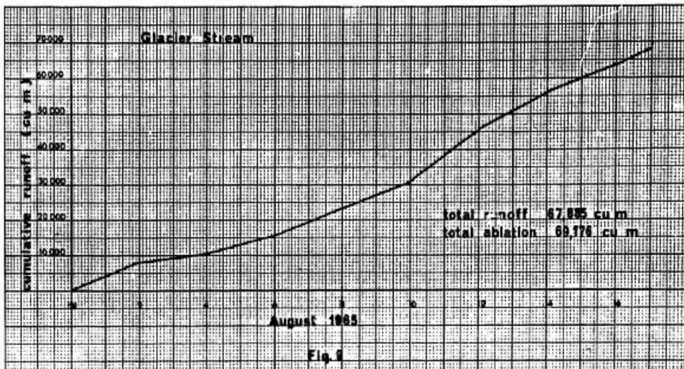
Fig.3.6. Cumulative discharge from Mir Samir West Glacier during August 1965.
