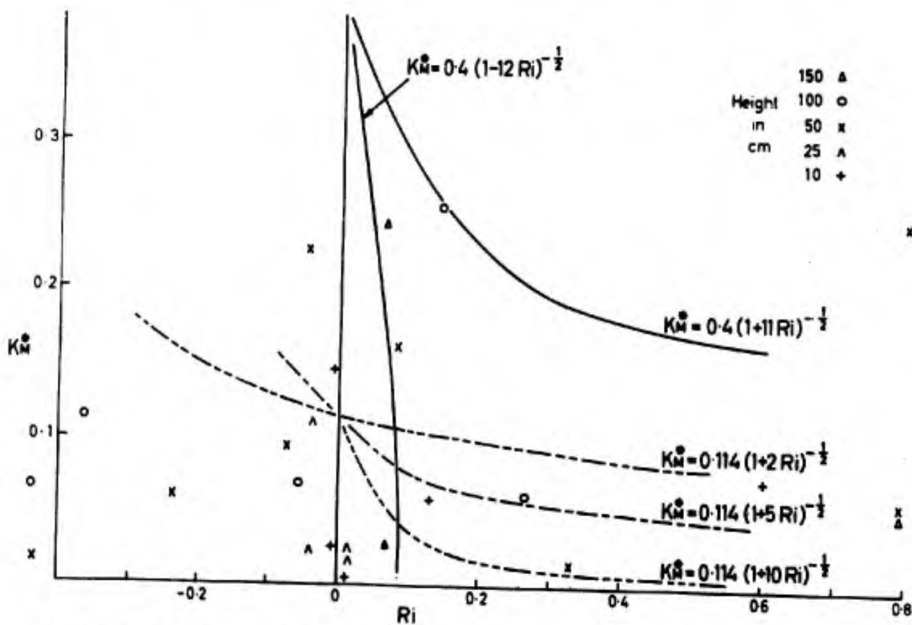
Fig.2.21. Eddy viscosity with stability
