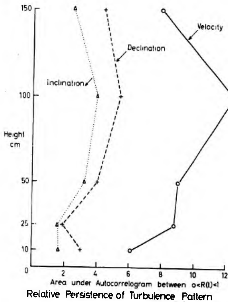
Fig.2.15. Persistence of turbulence pattern with height
