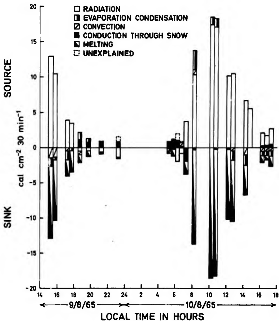
Fig.1.11. Heat balance Mir Samir West Glacier.
