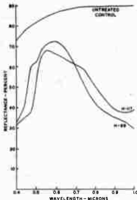
Figure 2: Reflectance of Cloth, Cotton, Sateen, 9 oz./yard, undyed, treated with two infrared absorbers, and of an untreated control.
