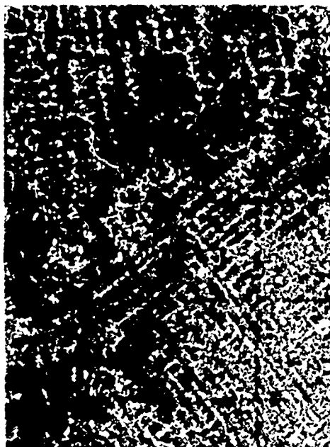
Fig. 5 - Further magnification of the same area as in Fig. 4. Note the parallel rows of bright antimony particles which show the positions of the channels between the primary dendrites; note also that voids (dark) align with these parallel rows of antimony particles. The original magnification was 400X. The superimposed line spacing represents 60 microns between lines.
