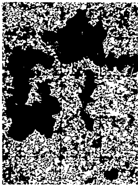
Fig. 12 - Another example of large voids, suggesting channels in the metal but bearing little relation to the surrounding microstructure. The original magnification was 400X.
