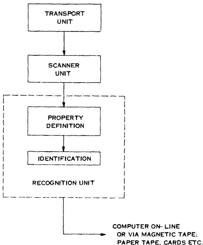
Figure 1. Block Diagram of Pattern Character Recognizer Reader
