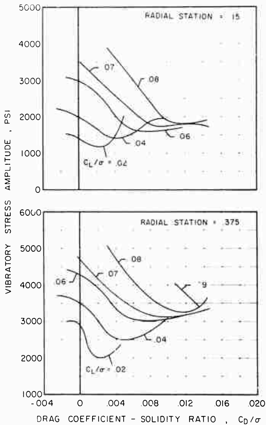
(a) Flapwise
