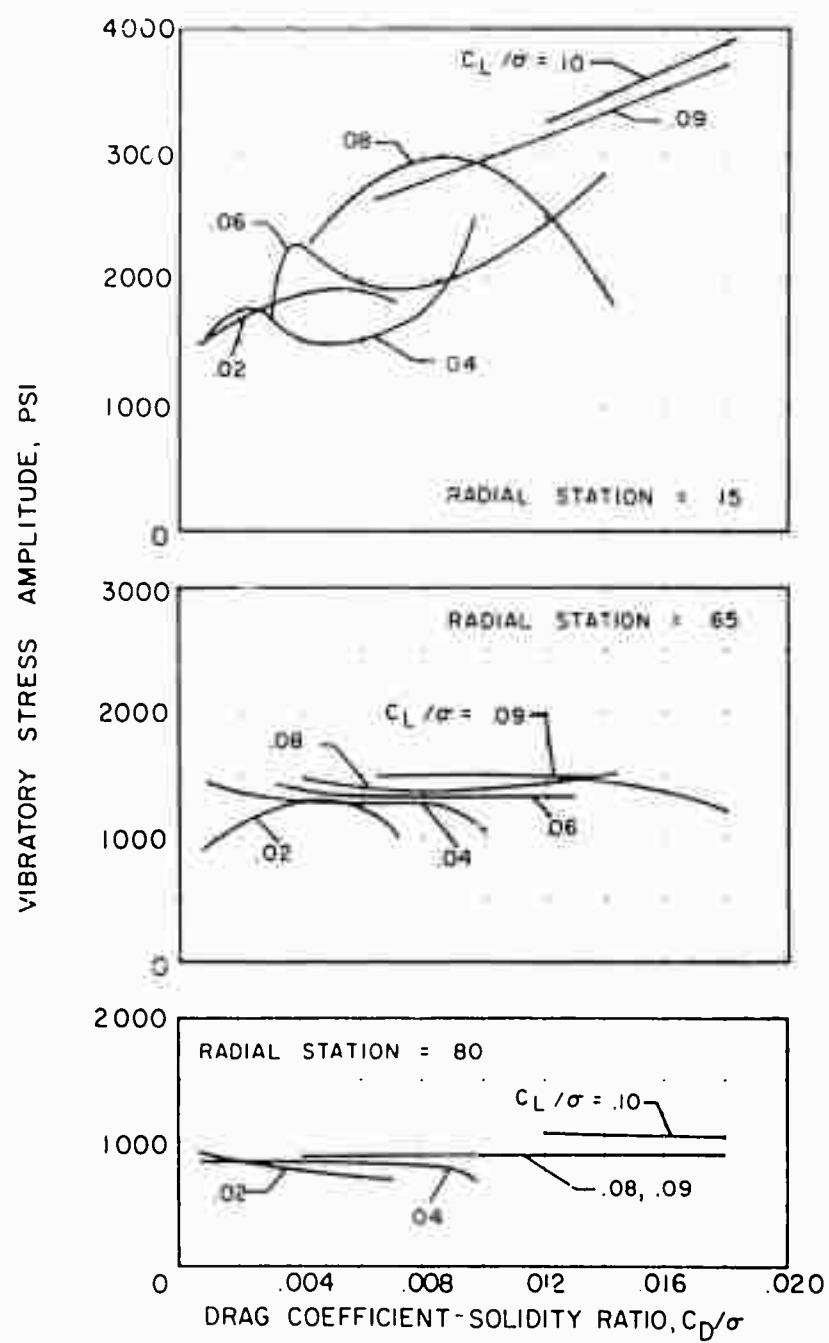
(b) Chordwise
