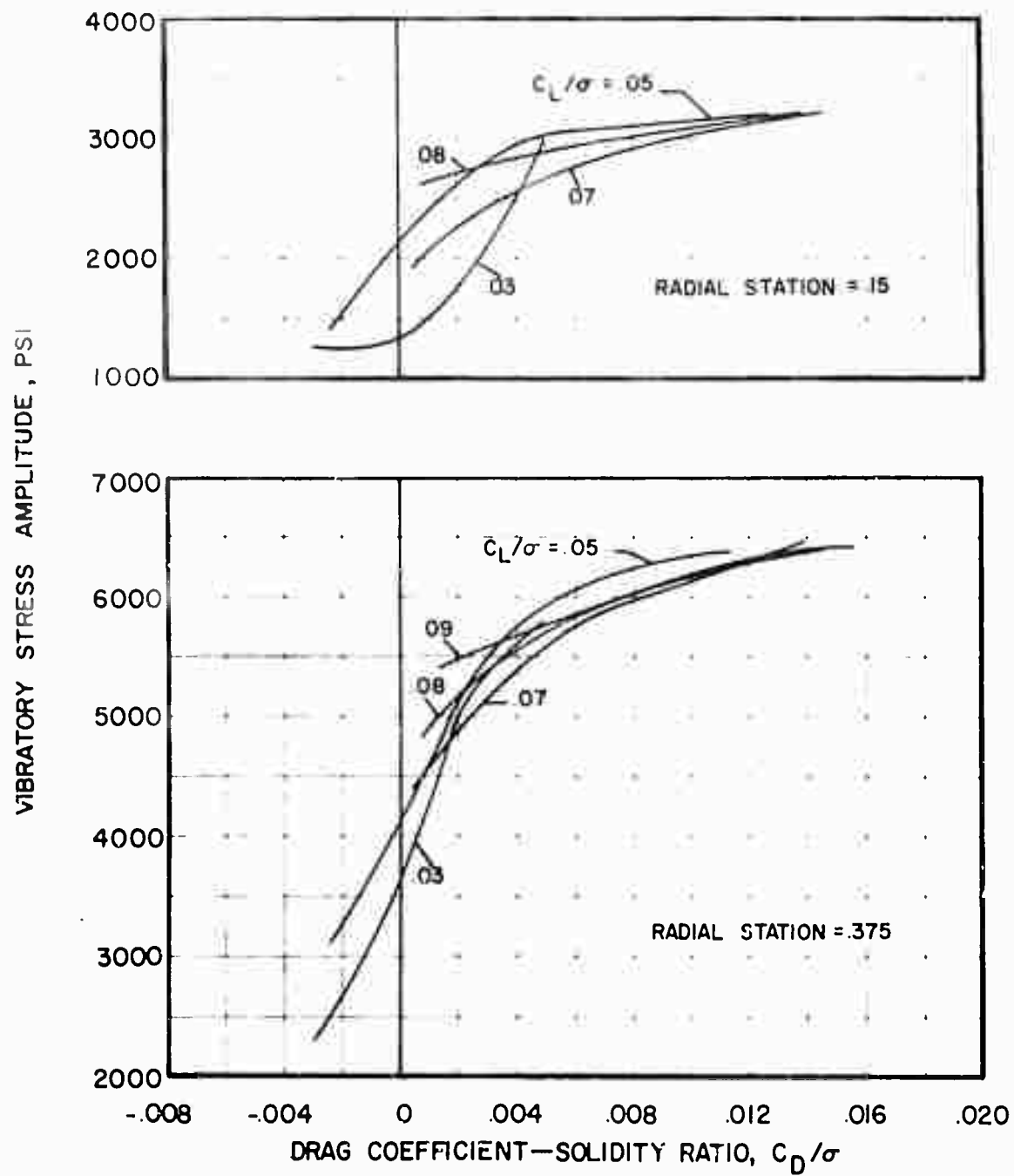
(a) Flapwise
