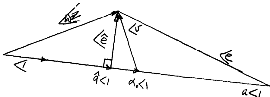
Fig. (1) Vector in k-Space
