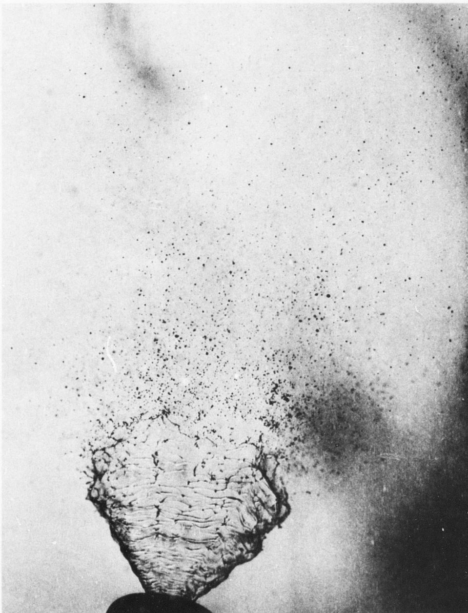
Figure 30. Neat JP-4 Passing Through Dual Orifice Nozzle (Actual Nozzle Size 0.400 in.).
