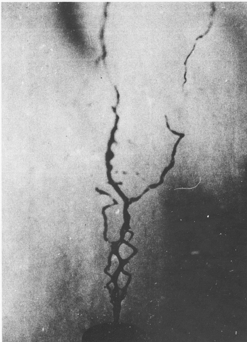
Figure 34. Emulsified JP-4 (2400 dynes/cm 2 ) Passing Through Dual Orifice Nozzle (Intermittent Behavior) (Actual Nozzle Size 0.400 in.).
