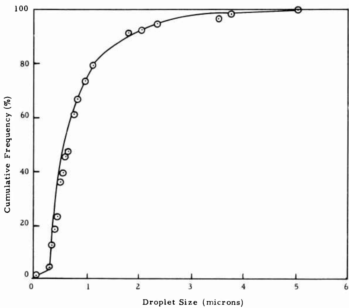
Figure 15. Droplet Size Distribution - Altered Emulsified JP-4 Fuel - 5 Minutes' Mixing Time.
