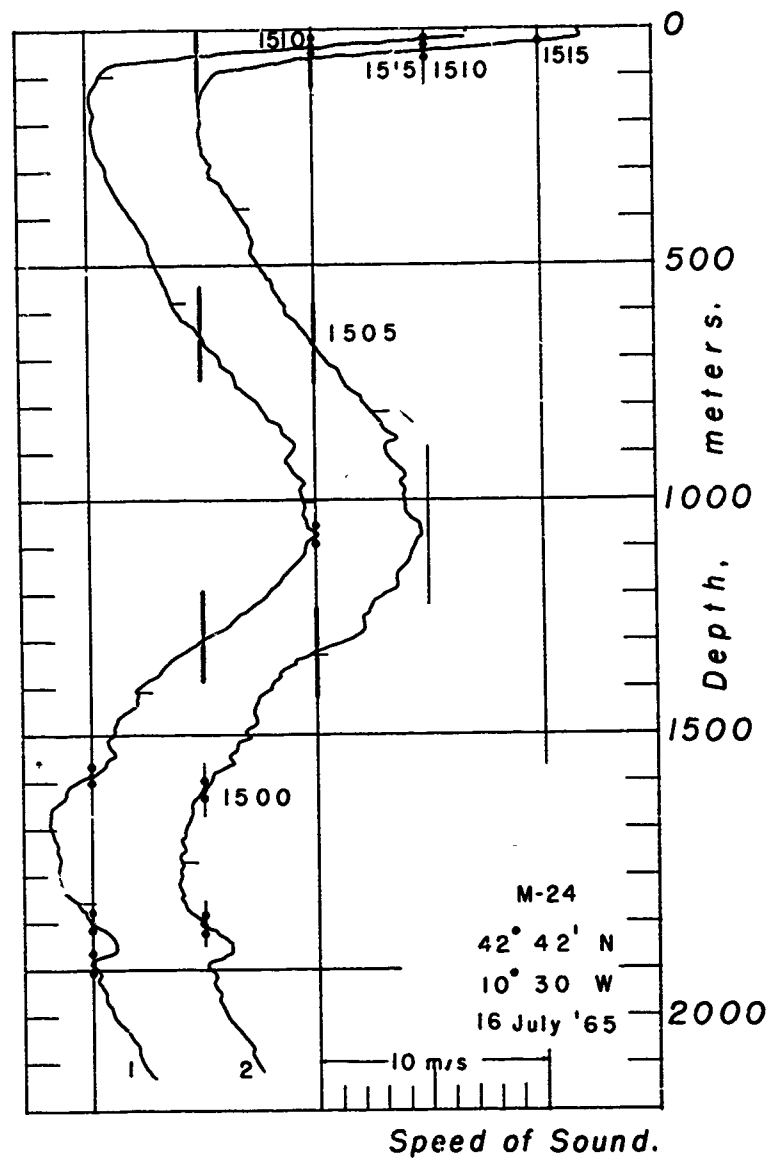
Fig. 47 Sound Speeds - Station M-24
