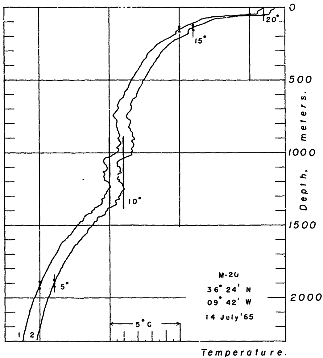
Fig. 40 Temperatures - Station M - 20
