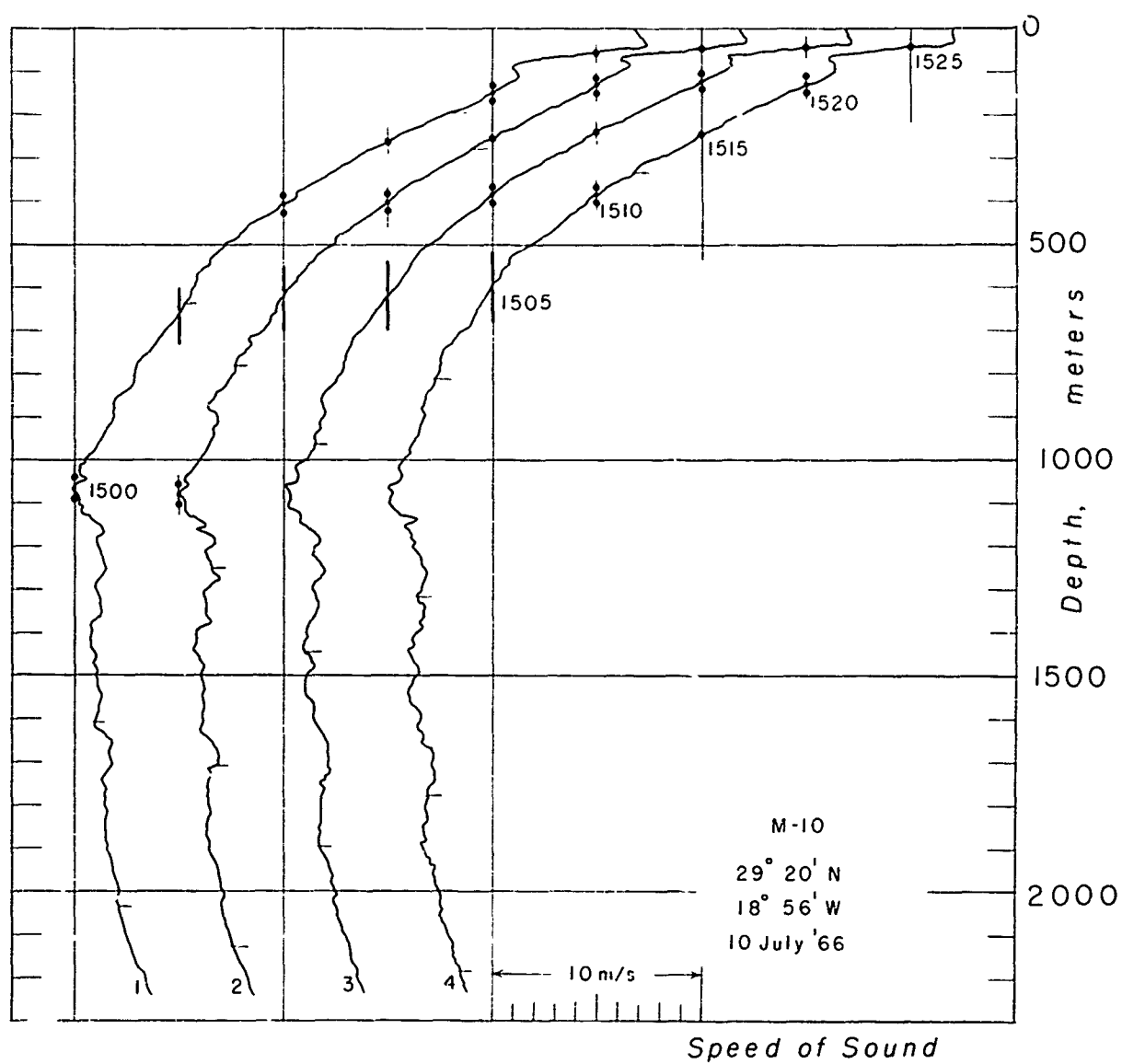
Fig. 19 Sound Speeds - Station M-10
