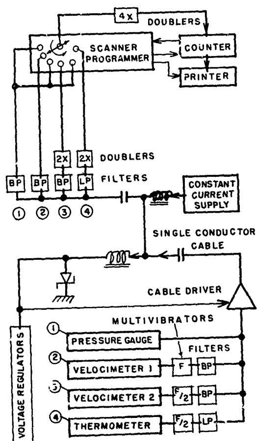
Fig. 2 Block diagram of Instrumentation
