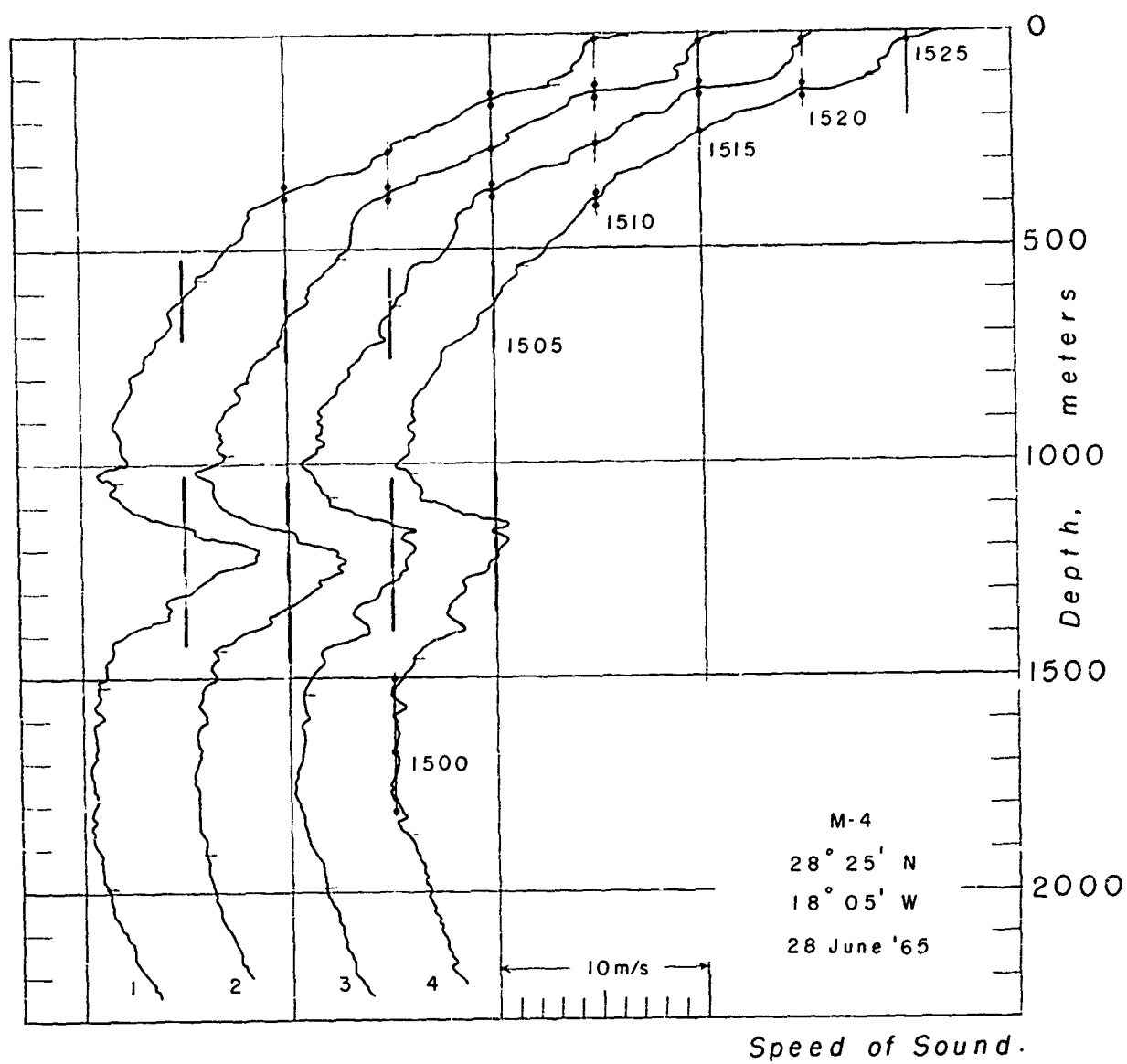
Fig. 7 Sound Speeds - Station M-4
