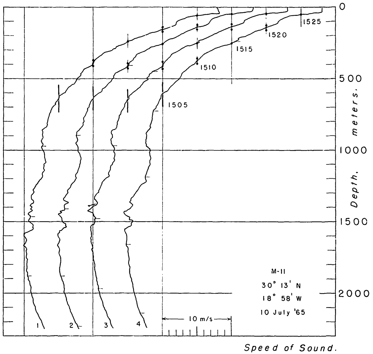
Fig. 21 Sound Speeds - Station M-II
