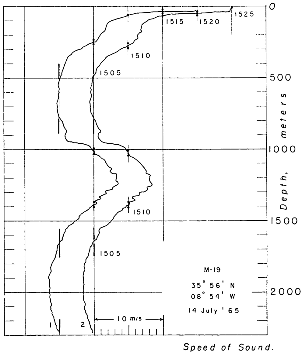
Fig. 37 Sound Speeds - Station M-19
