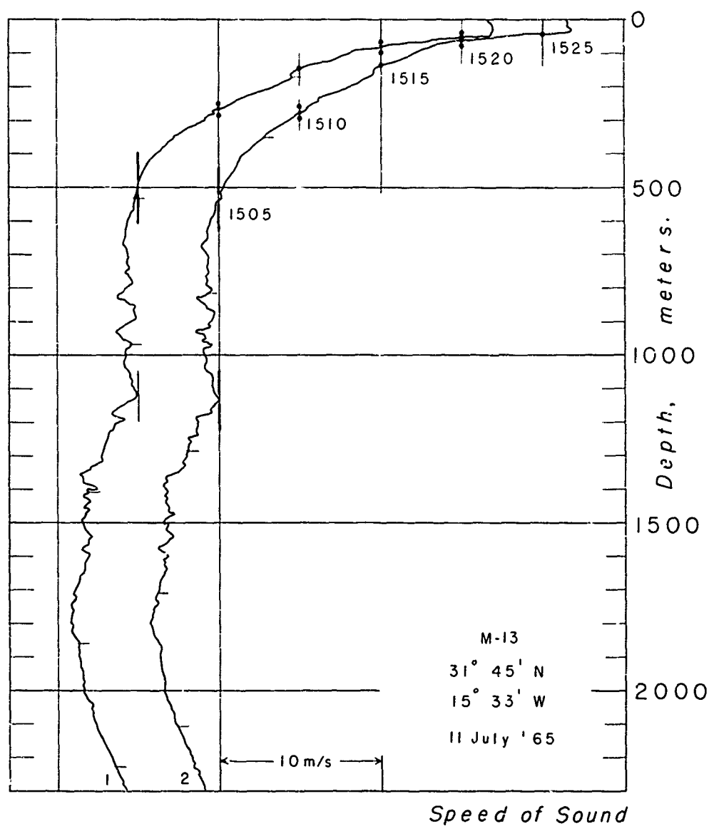
Fig. 25 Sound Speeds - Station M-13
