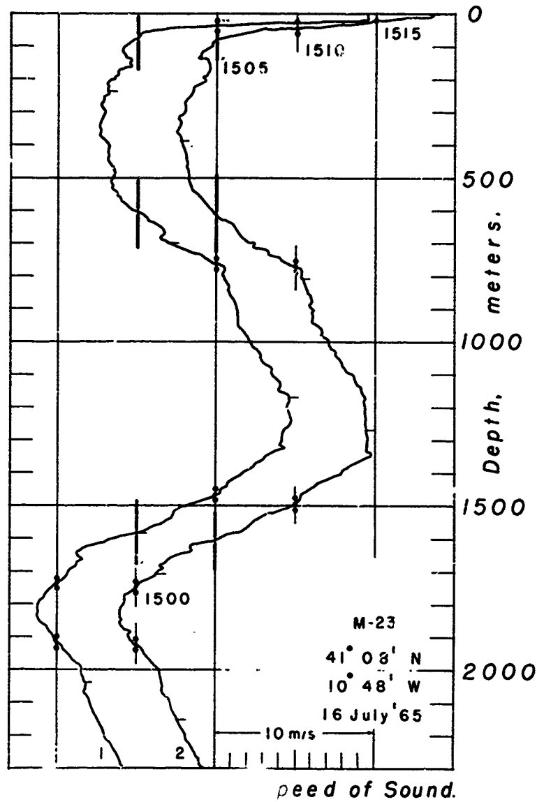
Fig. 45 Sound Speeds - Station M-23
