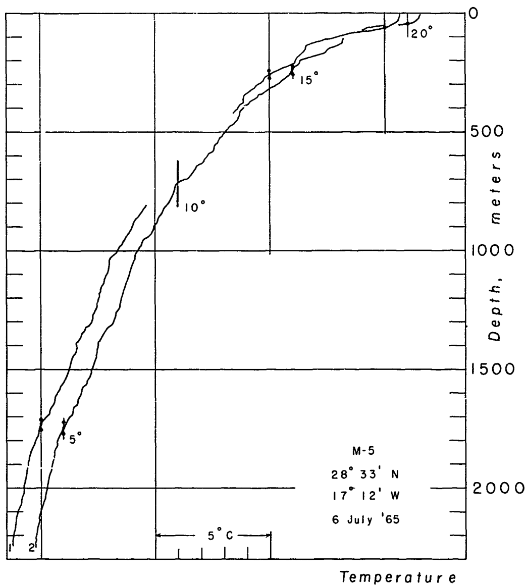
Fig. 10 Temperatures - Station M-5
