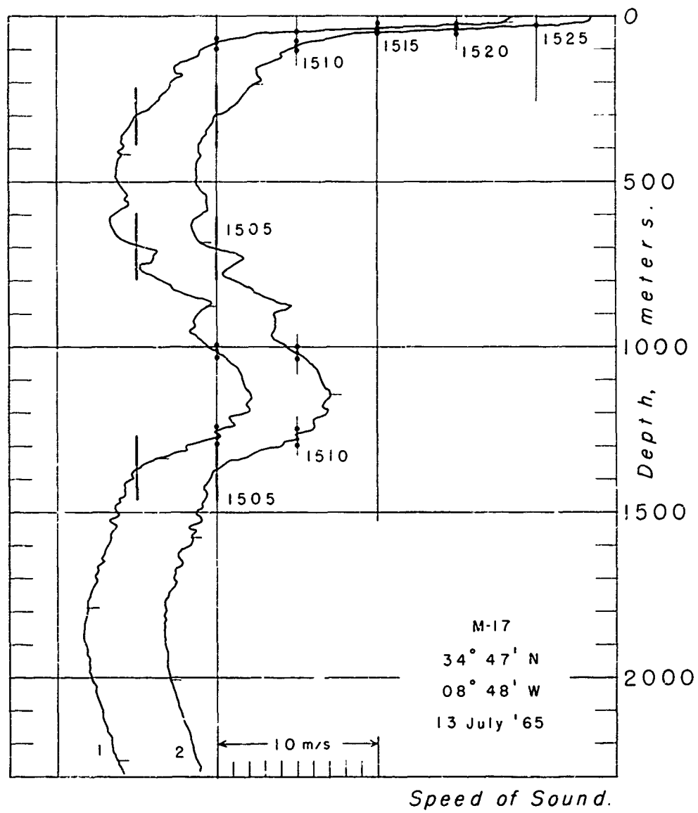
Fig. 33 Sound Speeds - Station M - 17
