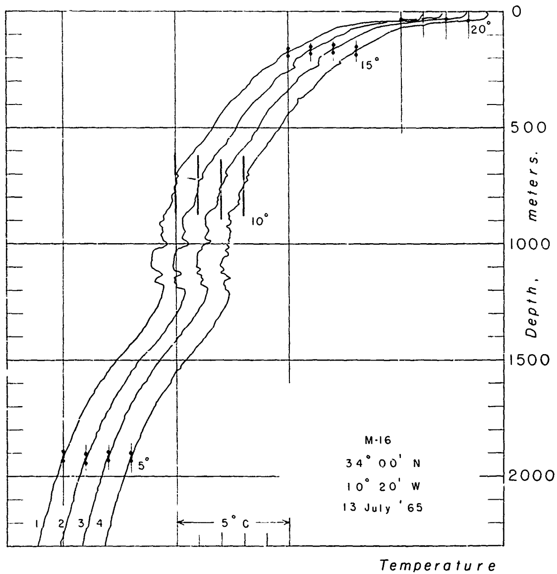
Fig. 32 Temperatures - Station M -16
