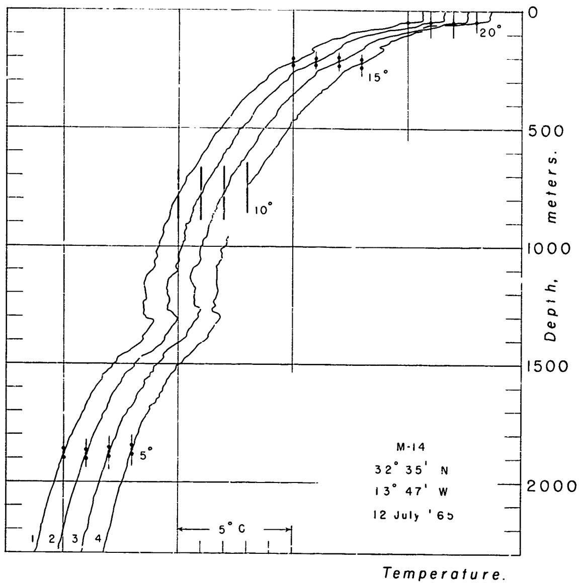
Fig. 28 Temperatures - Station M -14
