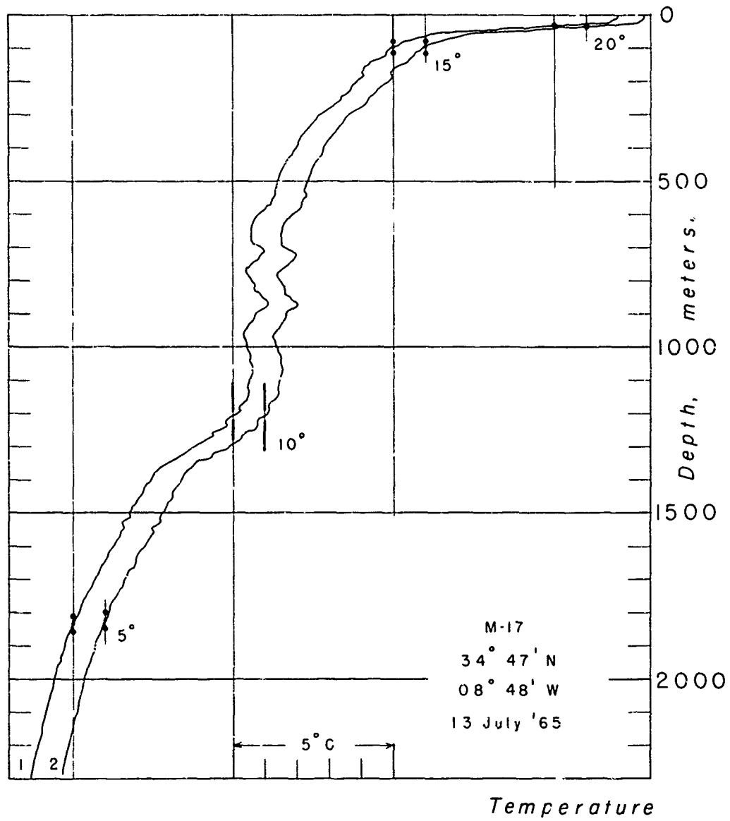
Fig. 34 Temperatures - Station M-17
