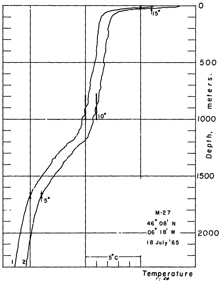
Fig. 54 Temperatures - Station M - 27
