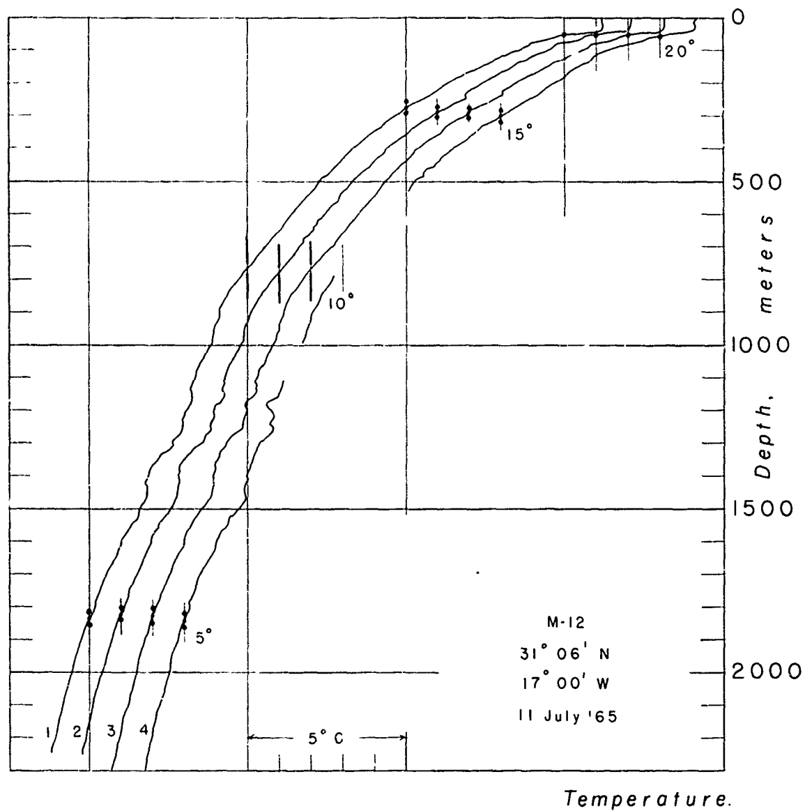
Fig. 24 Temperatures - Station M-12
