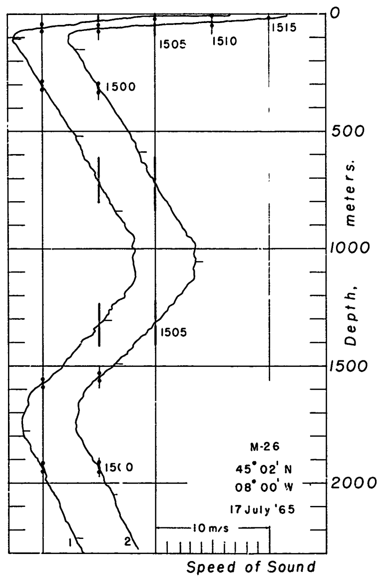
Fig. 51 Sound Speeds - Station M - 26
