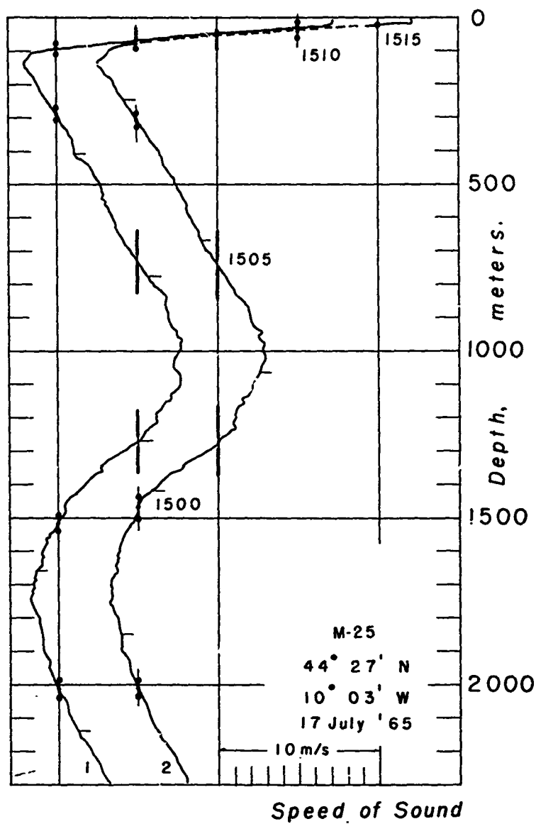
Fig. 49 Sound Speeds - Station M-25
