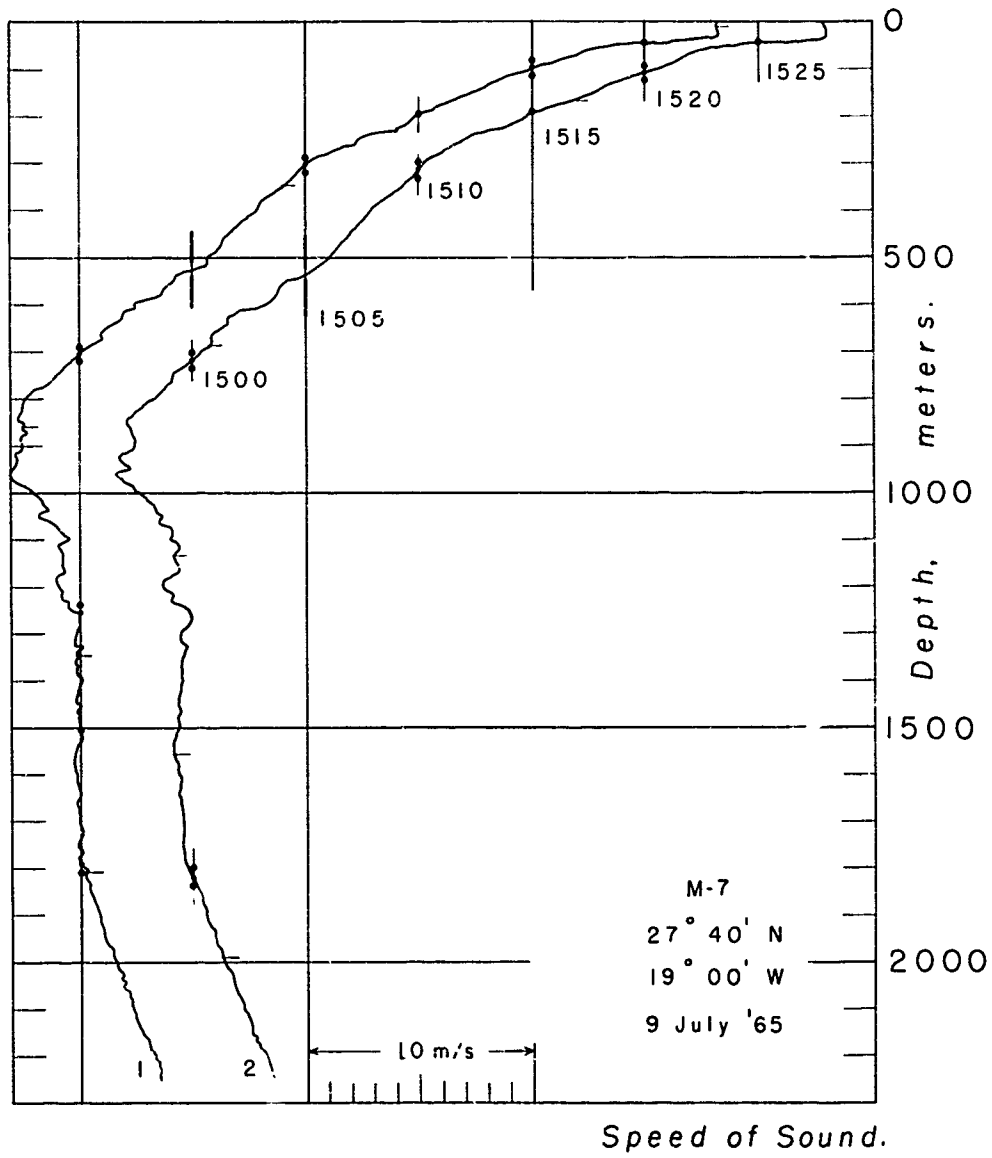
Fig.13 Sound Speeds - Station M - 7
