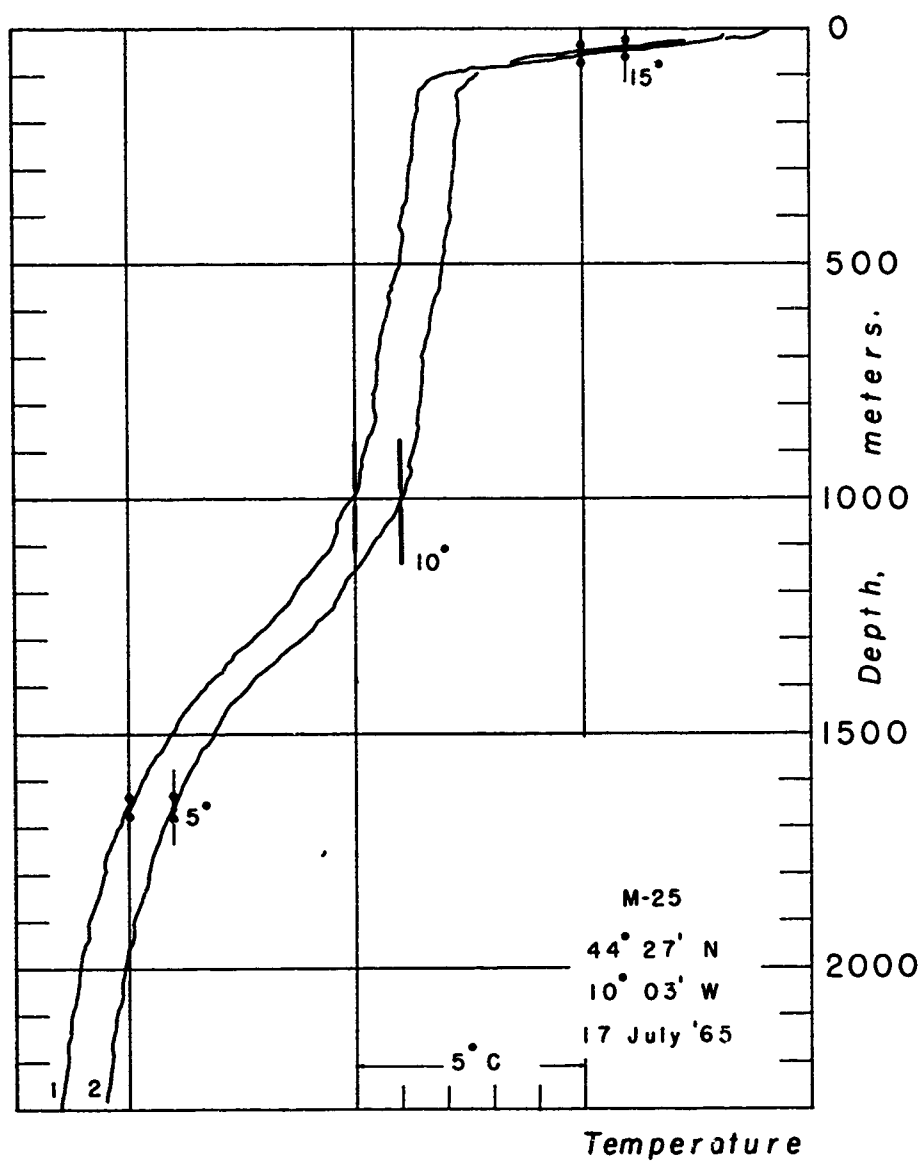
Fig. 50 Temperatures - Station M - 25
