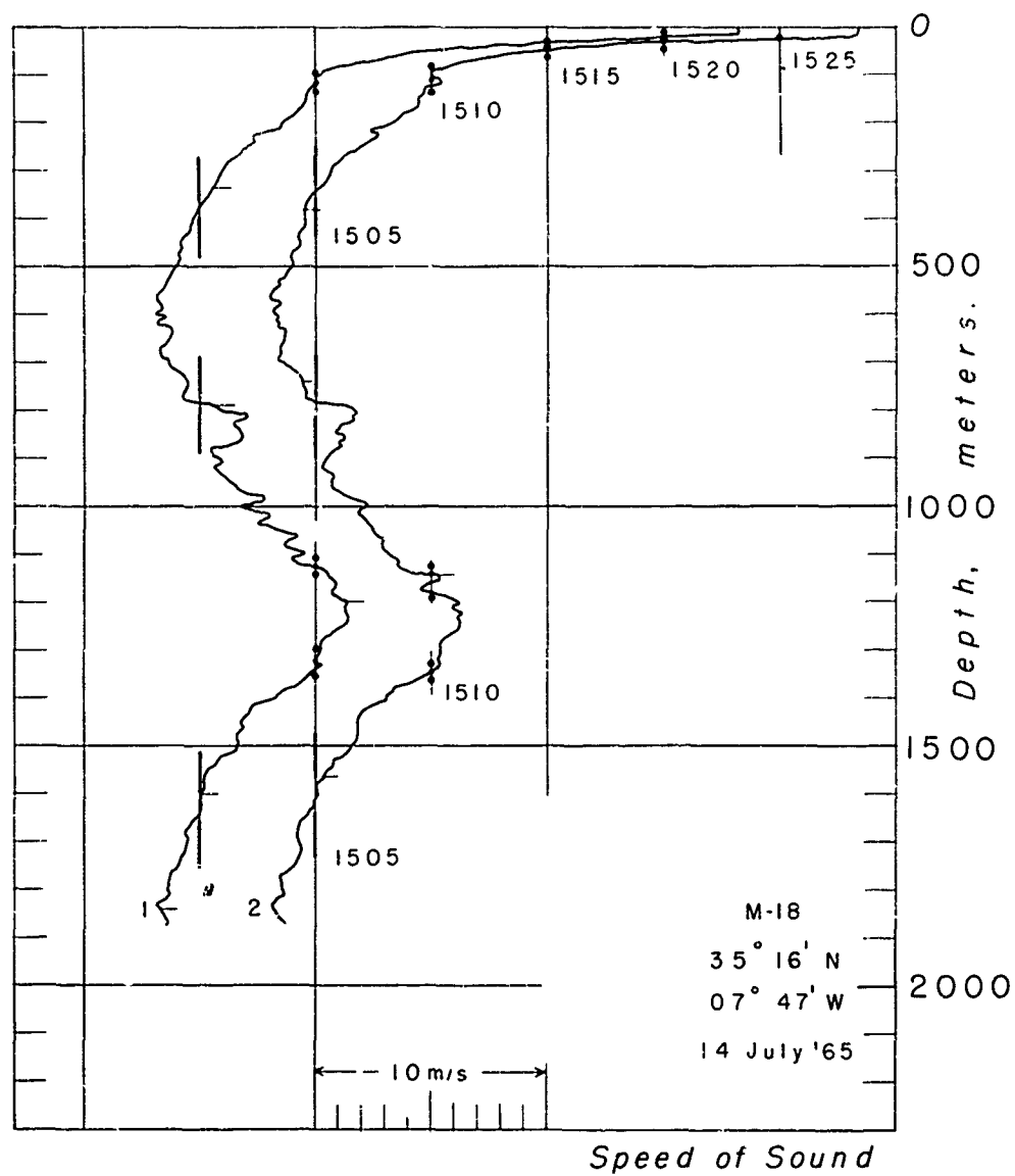
Fig. 35 Sound Speeds - Station M-18
