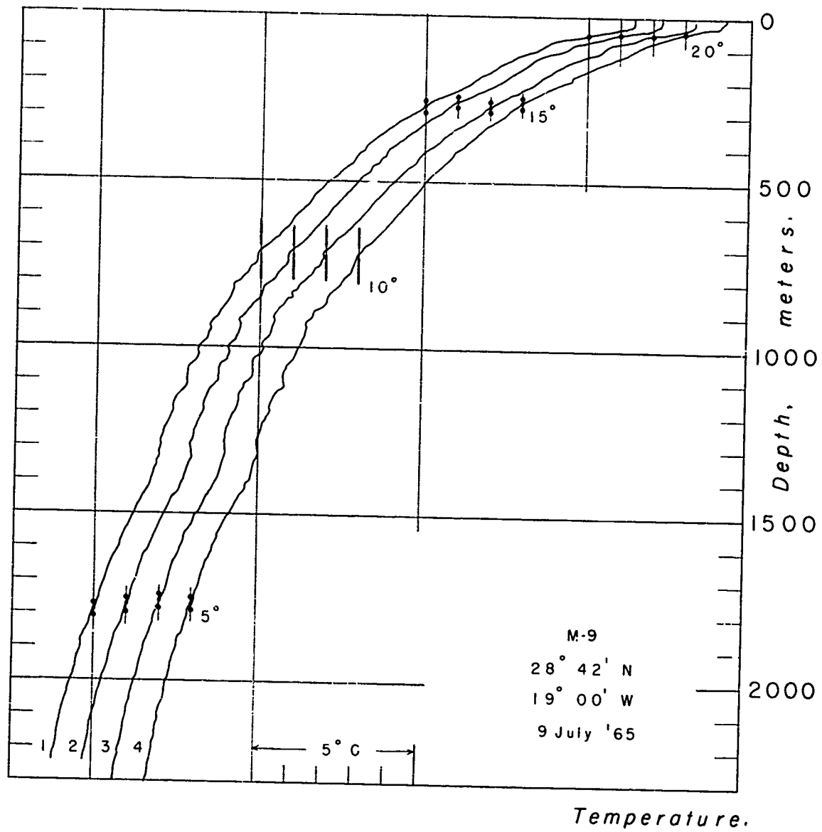
Fig. 18 Temperatures - Station M-9
