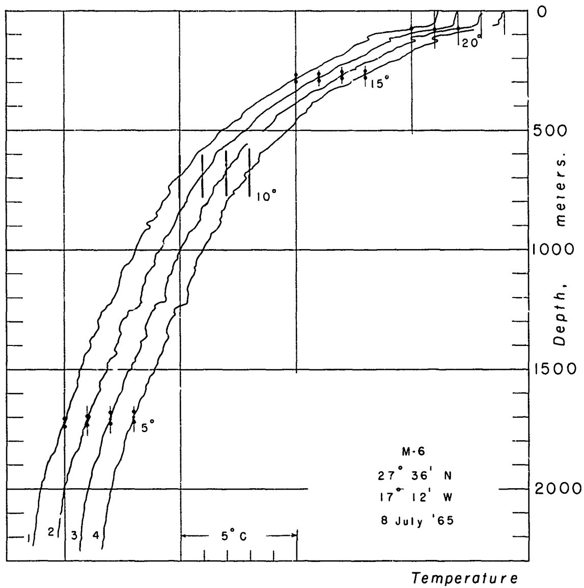
Fig. 12 Temperatures - Station M-6
