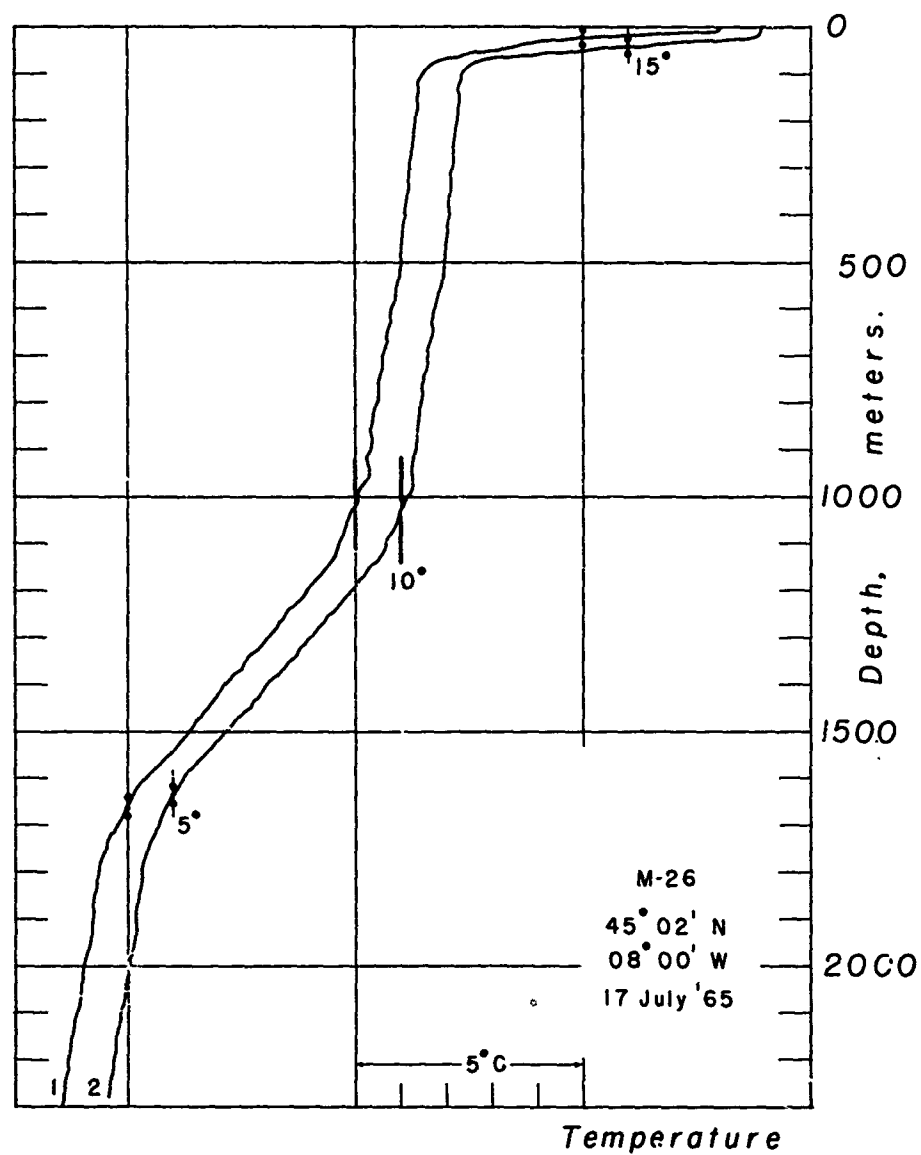
Fig. 52 Temperatures - Station M - 26
