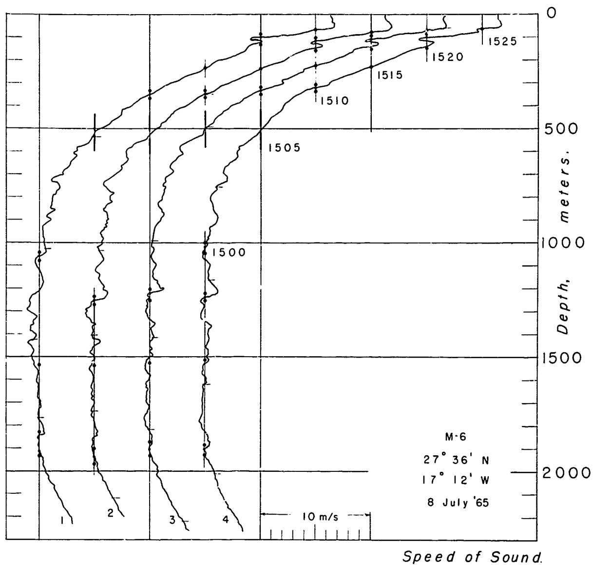
Fig. II Sound Speeds - Station M - 6
