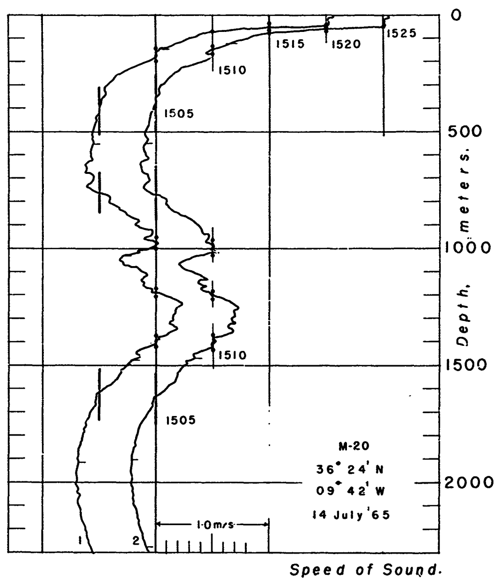
Fig. 39 Sound Speeds - Station M-20
