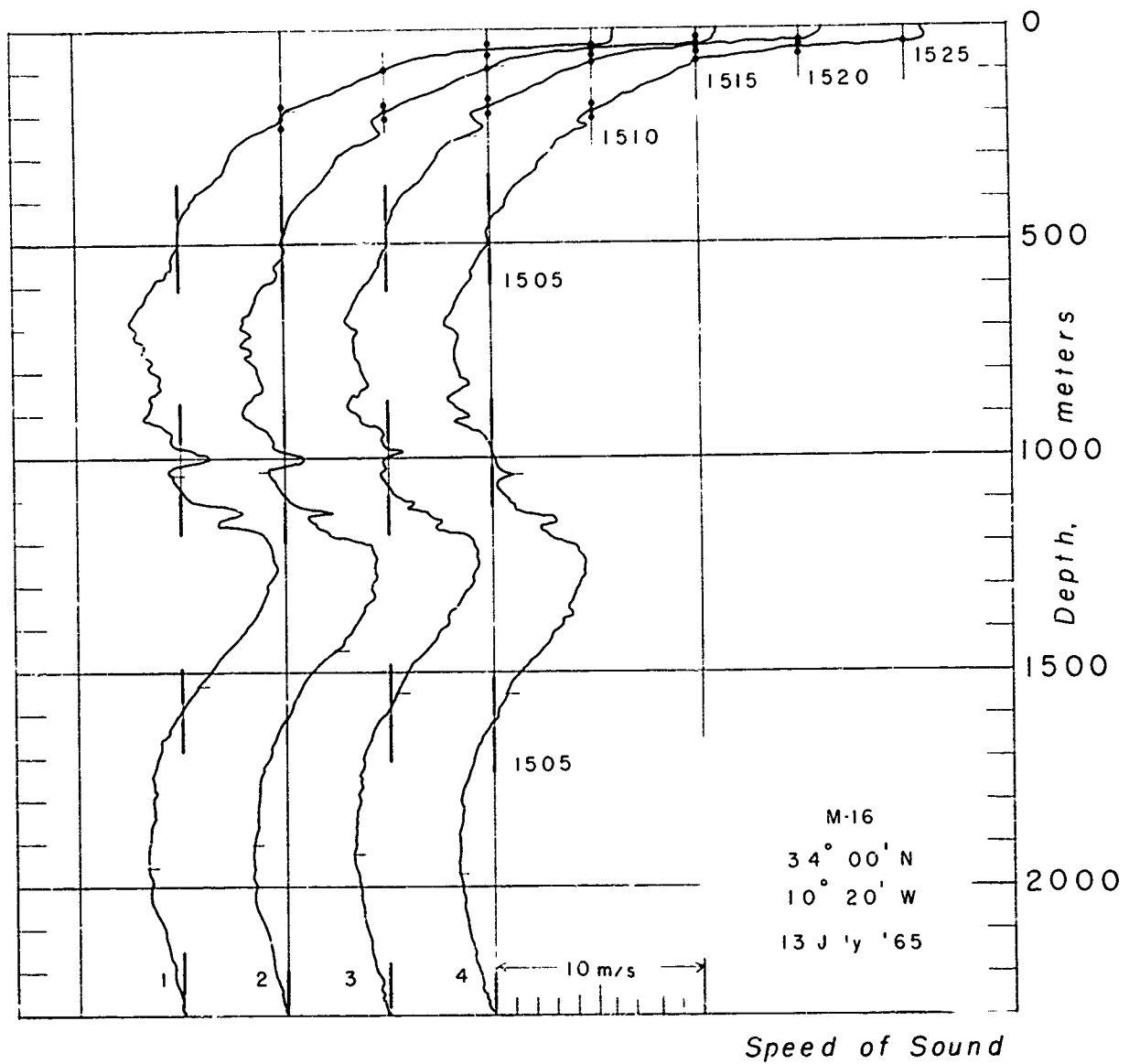
Fig. 31 Sound Speeds - Station M-16
