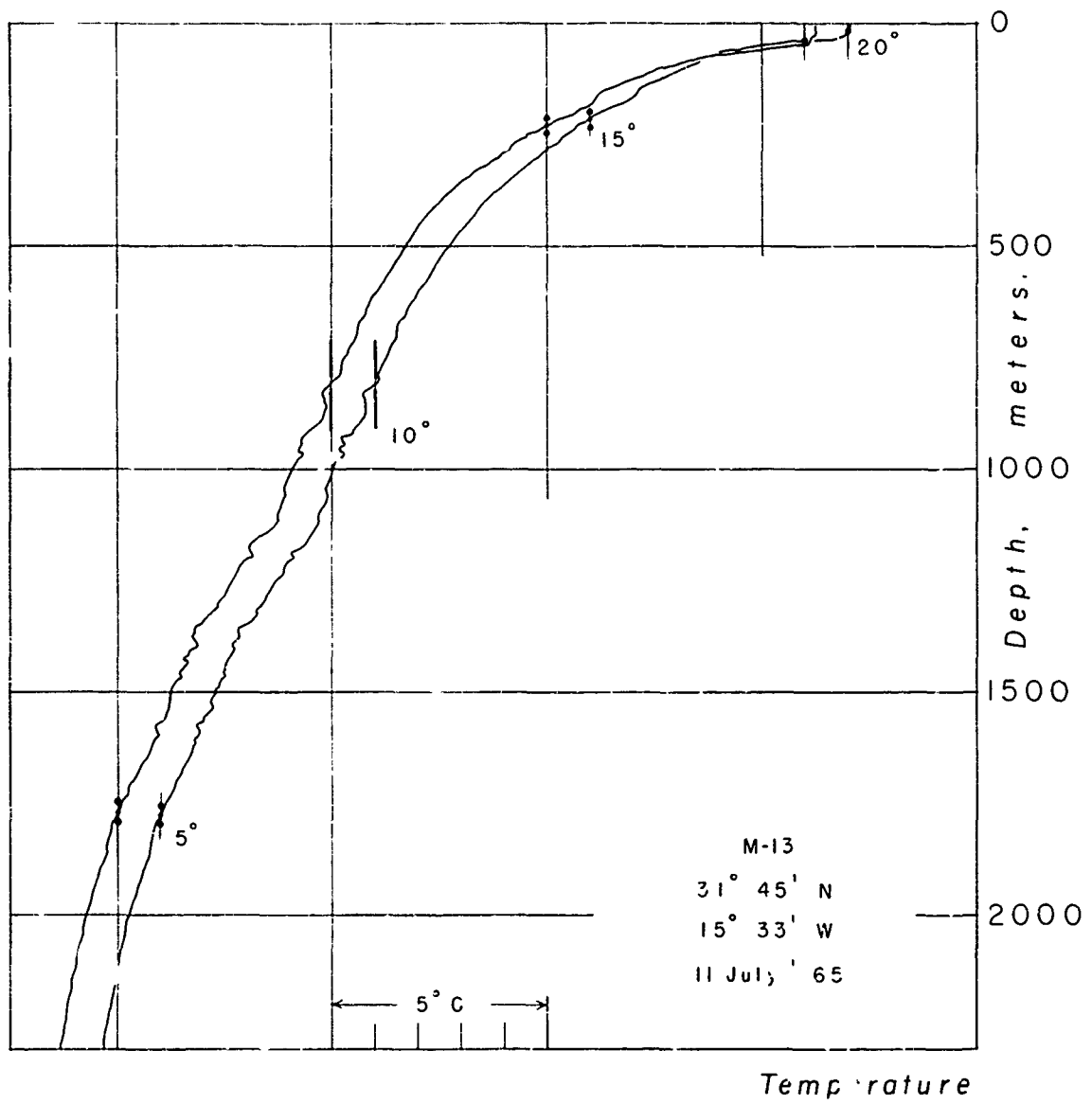
Fig. 26 Temperatures - Station M-13
