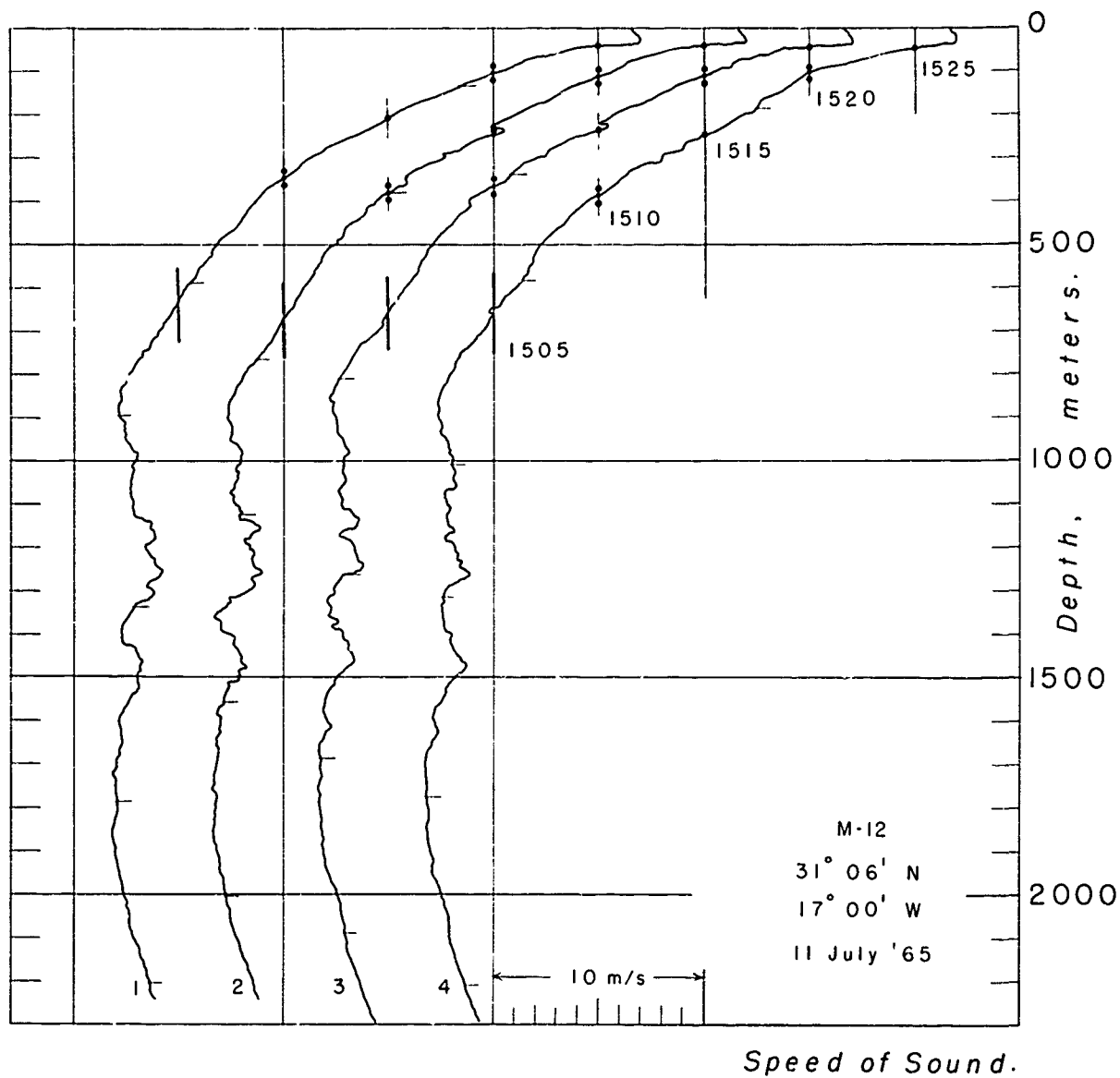
Fig. 23 Sound Speeds - Station M-12
