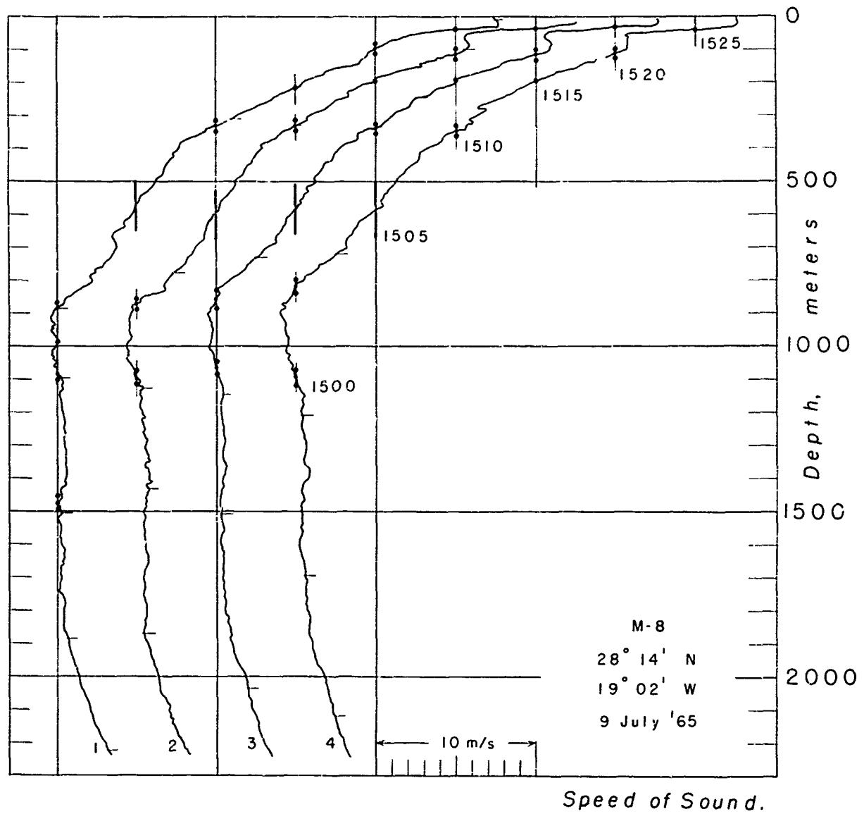
Fig.15 Sound Speeds - Station M - 8
