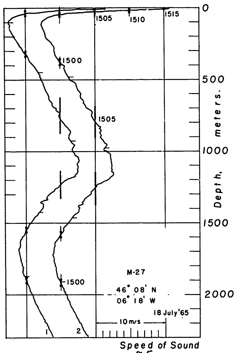
Fig. 53 Sound Speeds - Station M - 27
