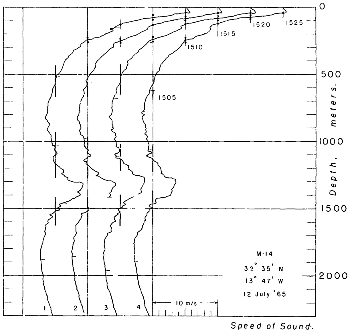
Fig. 27 Sound Speeds - Station M-14
