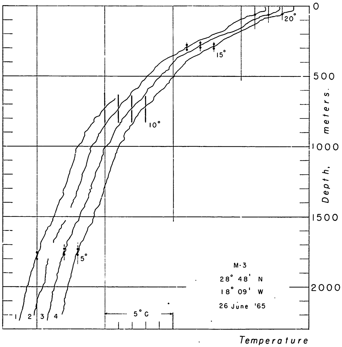
Fig. 6 Temperatures - Station M-3
