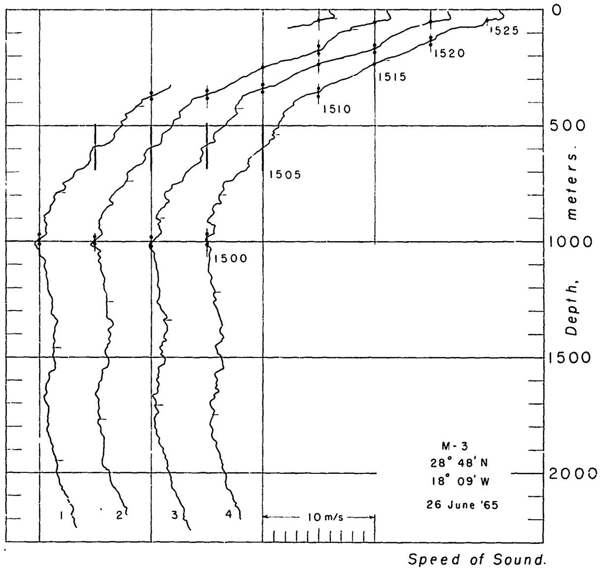
Fig. 5 Sound Speeds - Station M-3
