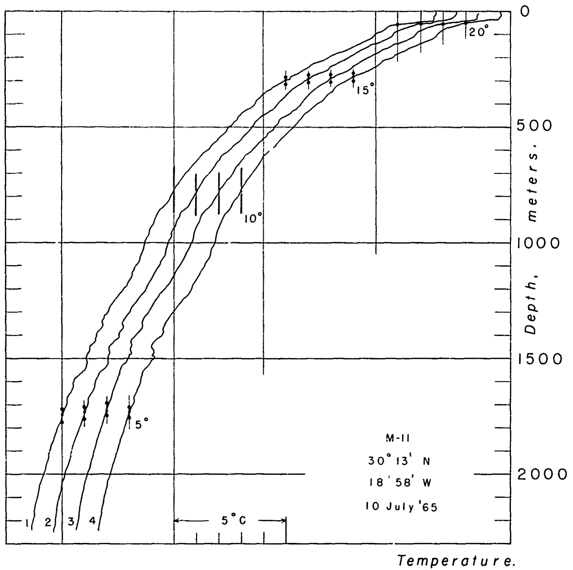
Fig. 22 Temperatures - Station M-II
