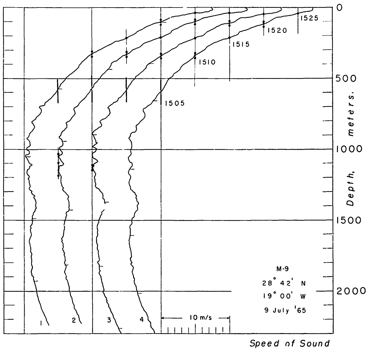
Fig. 17 Sound Speeds - Station M-9
