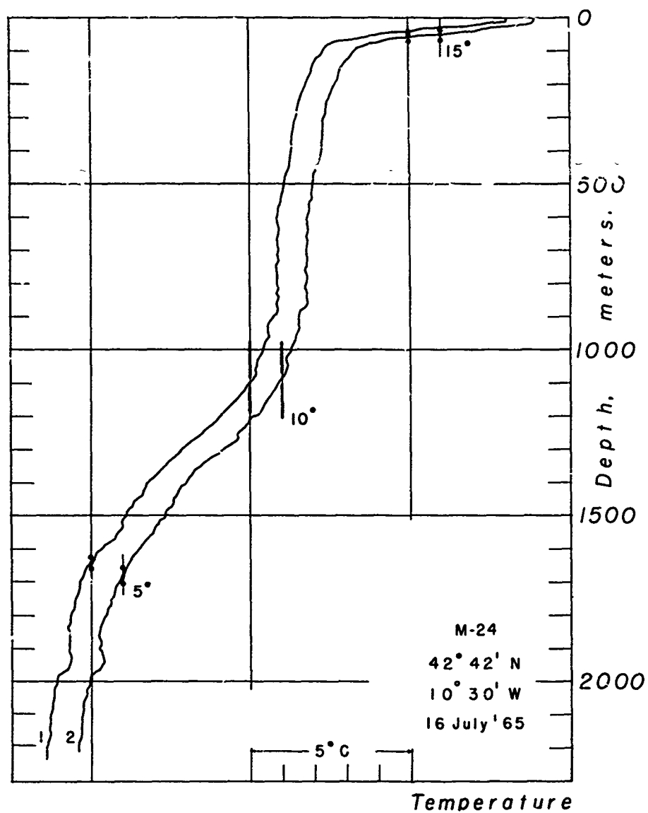
Fig. 48 Temperatures - Station M - 24
