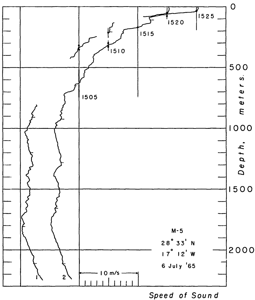
Fig. 9 Sound Speeds - Station M-5
