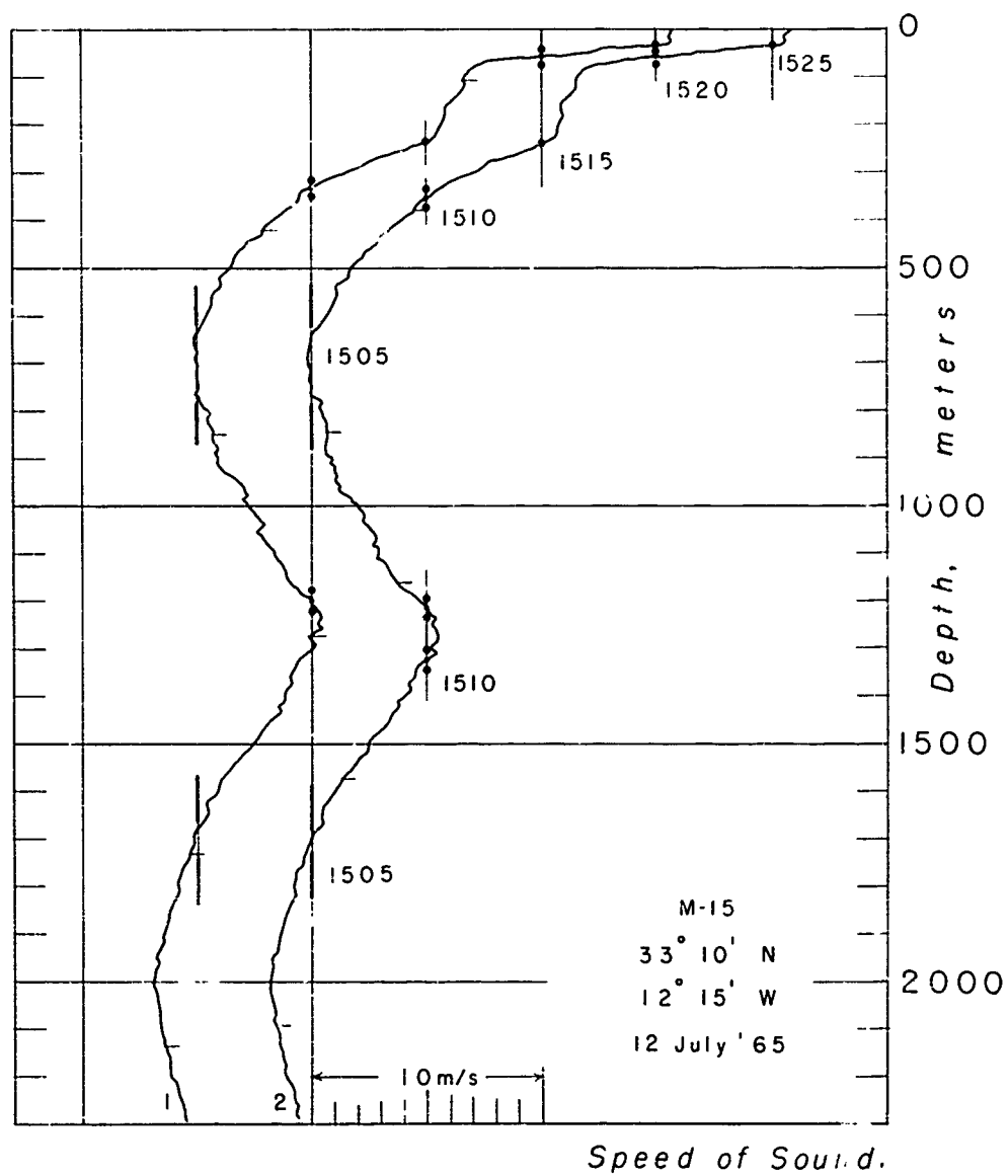
Fig. 29 Sound Speeds - Station M-15
