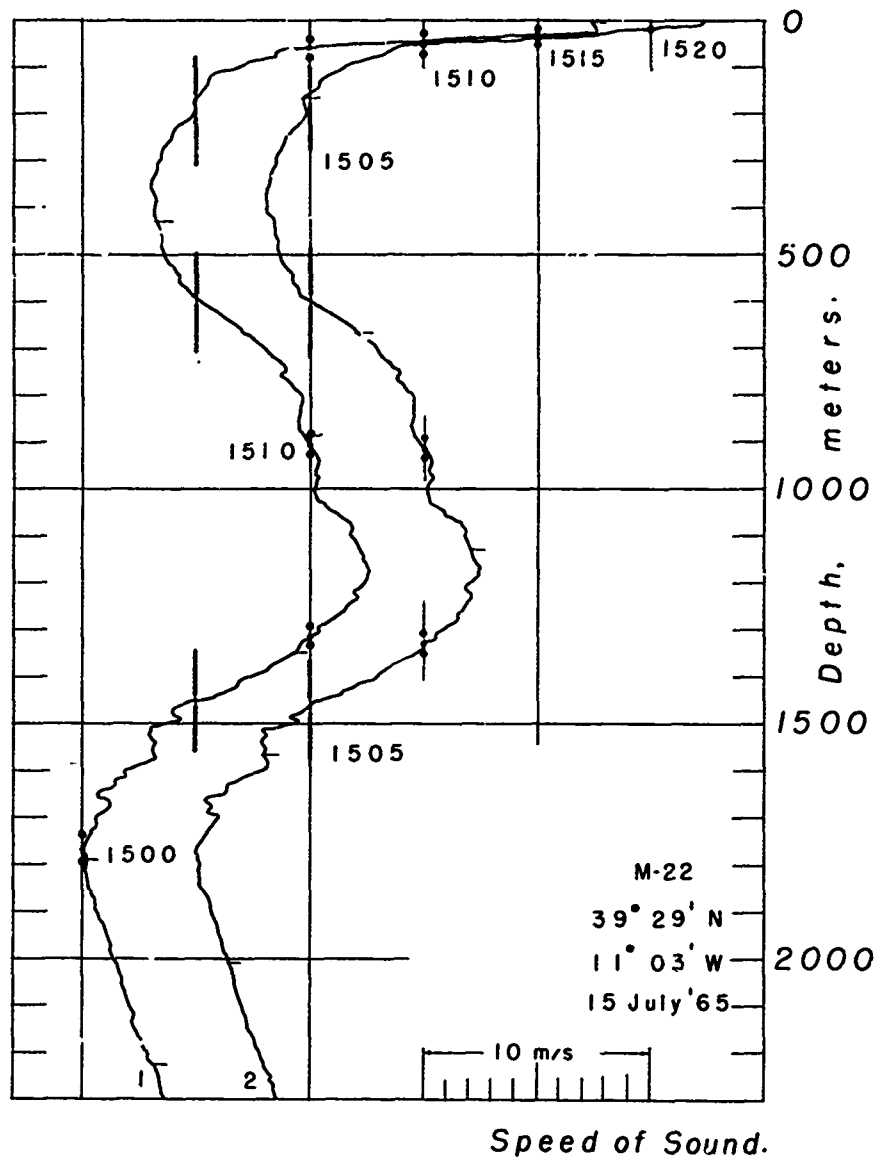
Fig. 43 Sound Speeds - Station M-22
