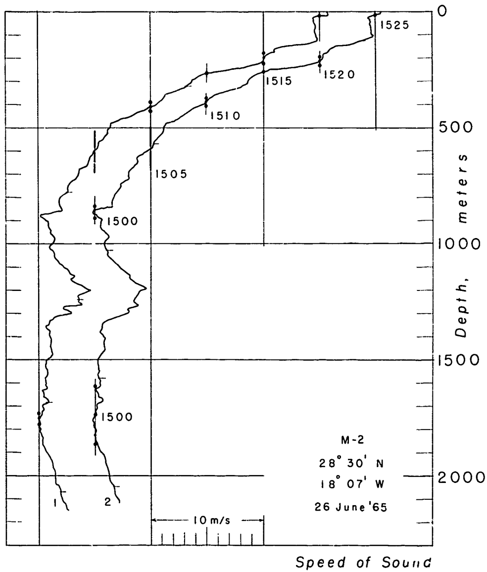
Fig. 3 Sound Speeds - Station M-2
