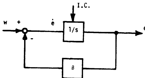
Fig. 13 Stochastic process with exponentially correlated output.
