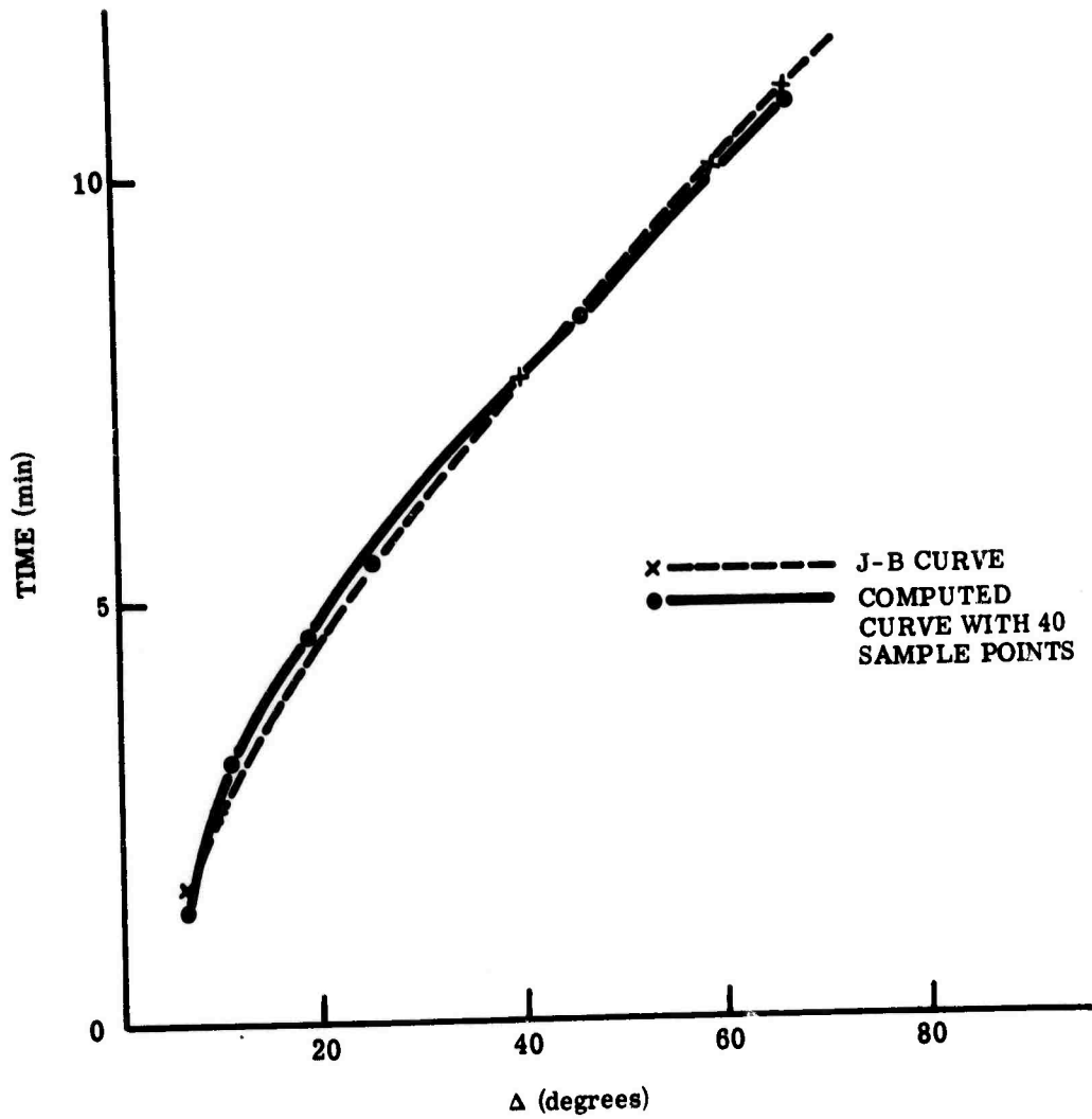
FIGURE 45. TRAVEL-TIME CURVE PLOTTED WITH SAMPLED JEFFREY-BOLLEN RADIAL P-WAVE VELOCITY PROFILE
