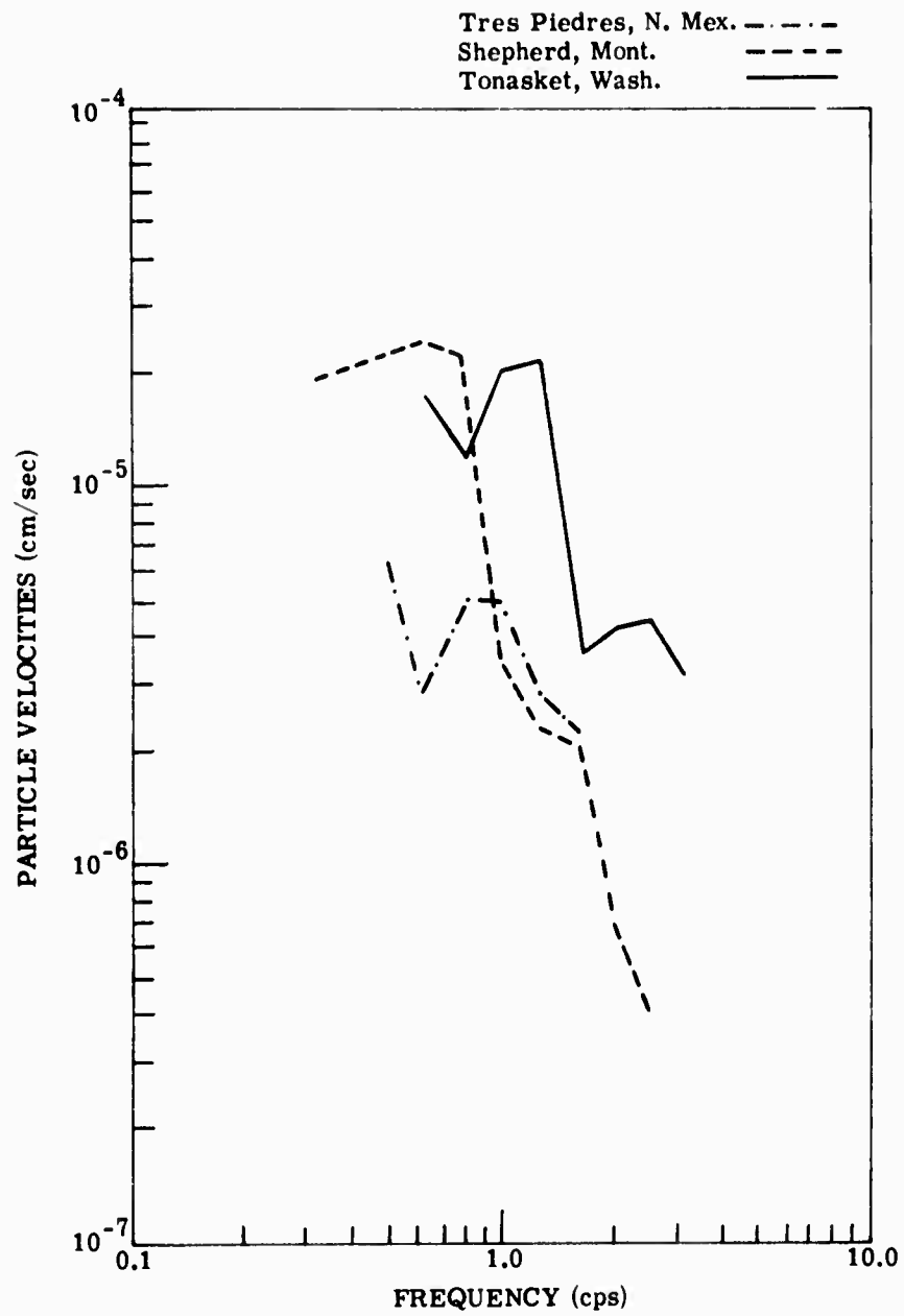
FIGURE 32. SHOAL P n PARTICLE VELOCITIES AT 1100-km SITES
