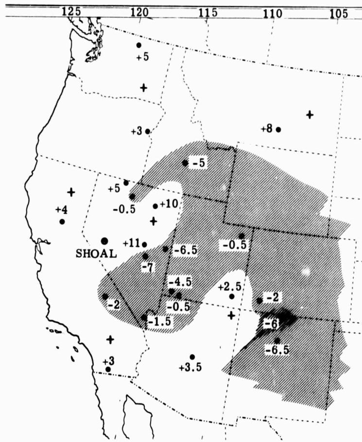
FIGURE 29. SHOAL P. AMPLITUDE RESIDUALS IN DECIBELS RELATED TO MEAN INVERSE CUBE
