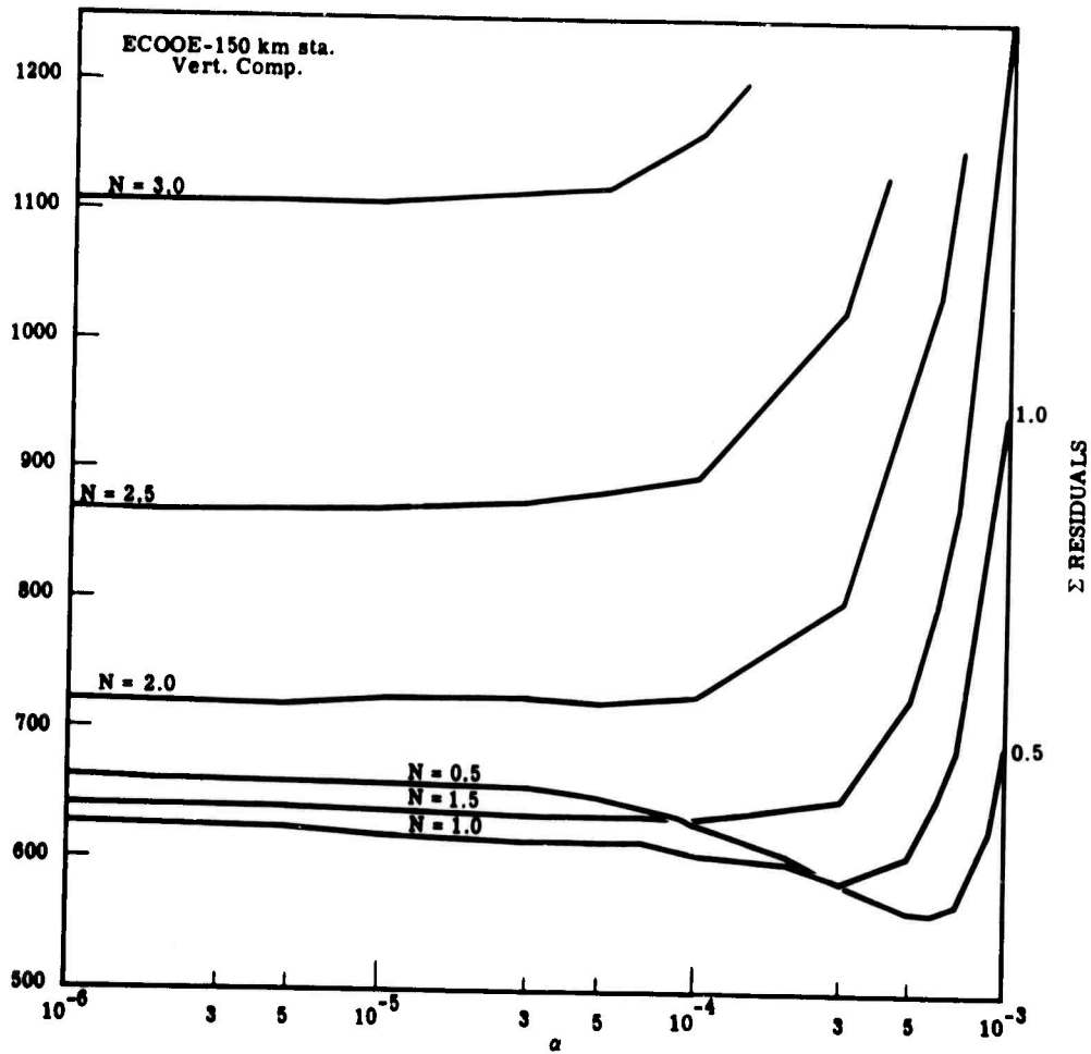
FIGURE 17. SUMMATION OF RESIDUALS VS. \alpha FOR ECOQE SOUTHERN PROFILE 150-KM SITE
