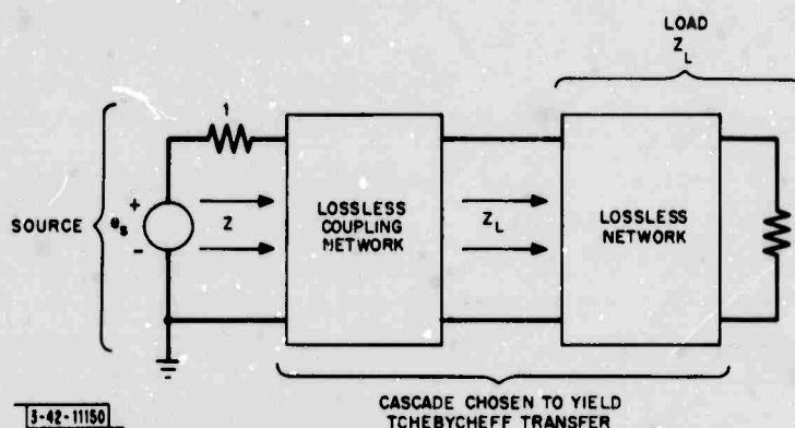
Fig. 1-4. Darlington realization of Tchebycheff transfer.
