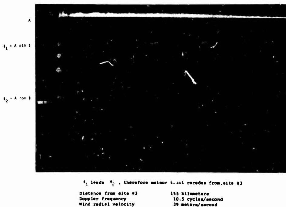
Figure 5. Sample of One-dimensional Wind Measurement (meteor trail receding from site No. 3)
