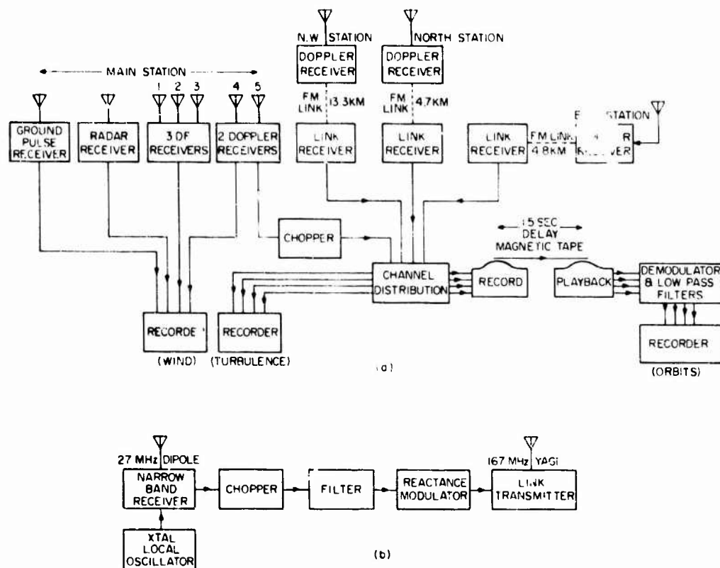
Figure 5. Block Diagrams of (a) the Equipment at the Main Receiving Station, (b) the Outstation Equipment
