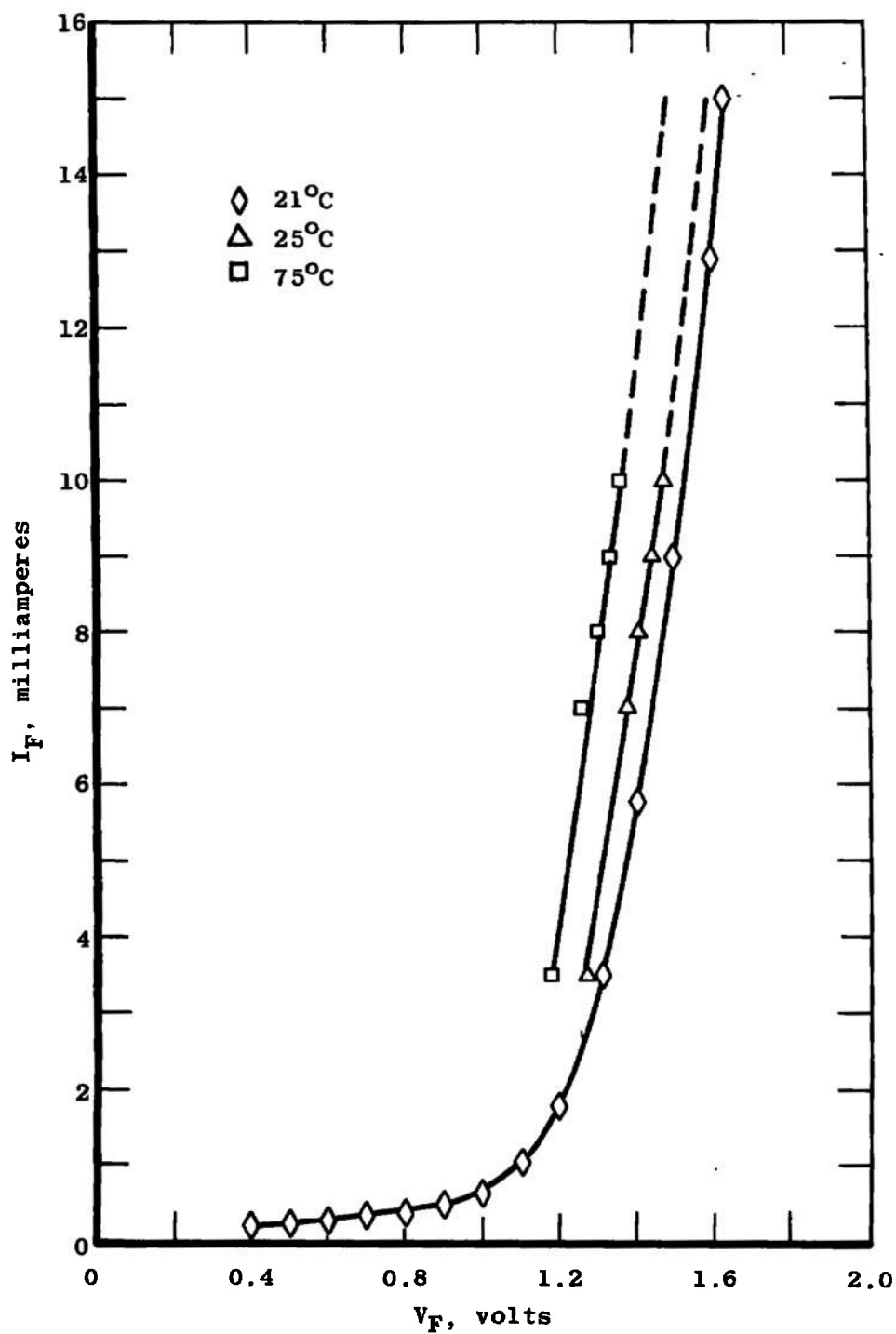
Figure 13. 1N661 forward current versus forward voltage for varying temperature.
