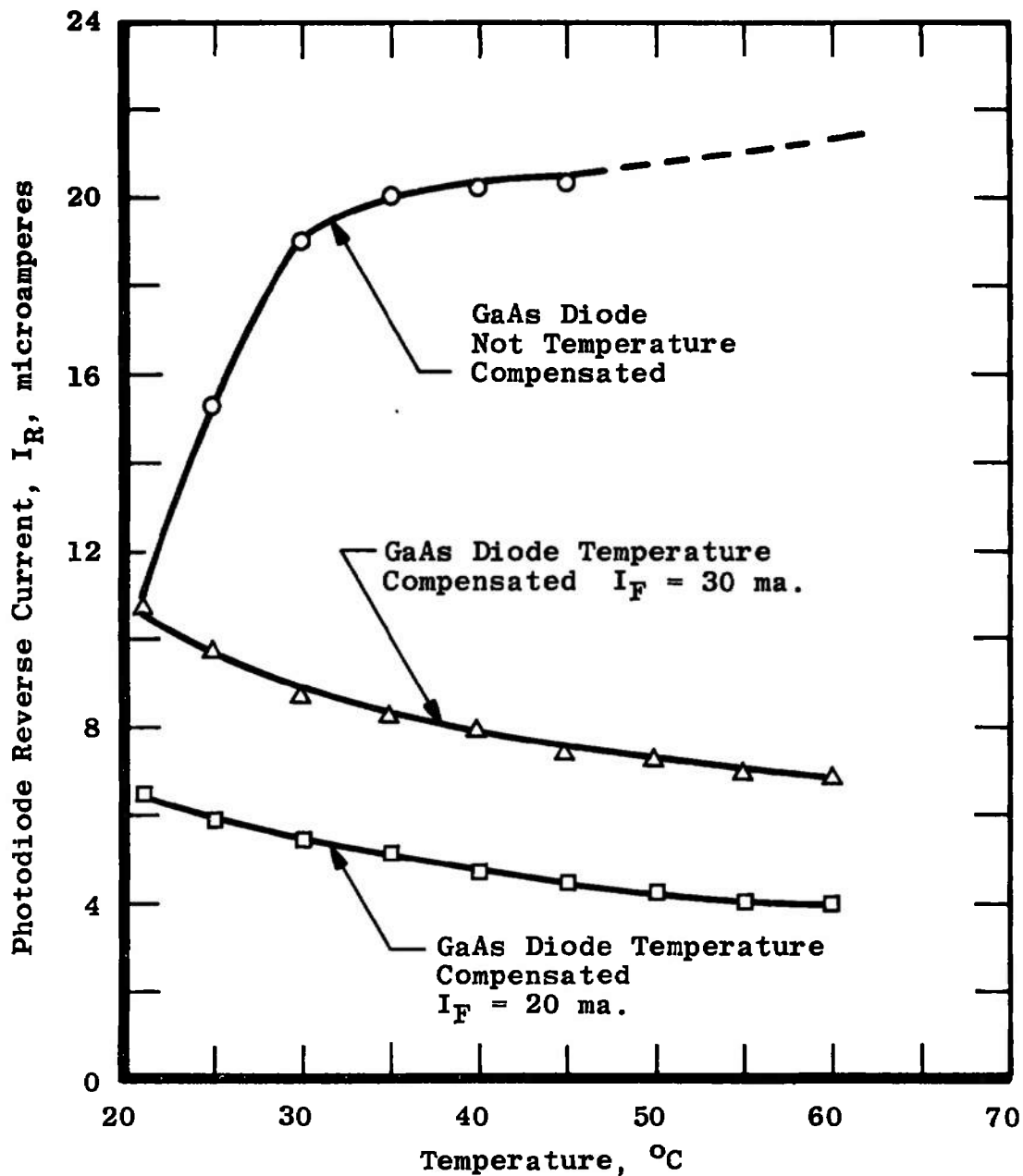
Figure 20. Photodiode reverse current versus temperature for compensated and uncompensated input.
