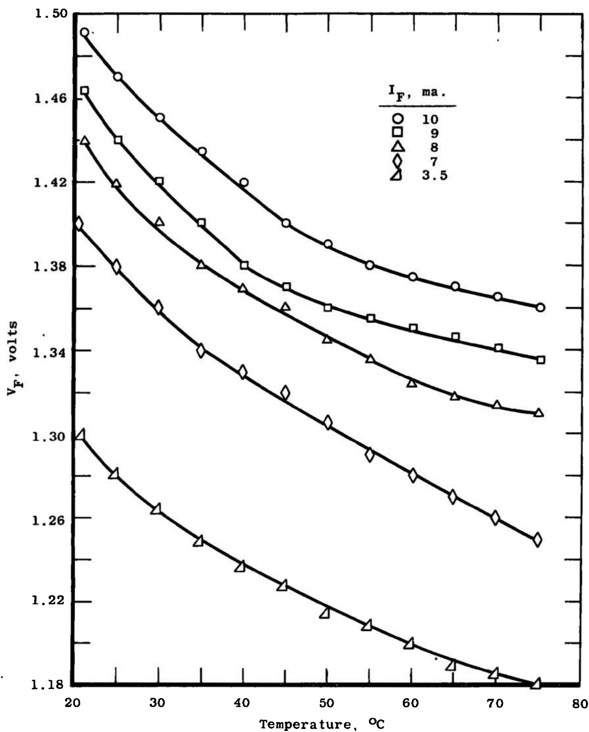
Figure 14. 1N661 forward voltage versus temperature change for constant forward current.
