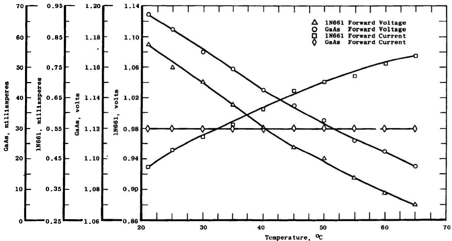
Figure 16. Current and voltage variations with temperature for a GaAs diode biased with a 1N661 diode.
