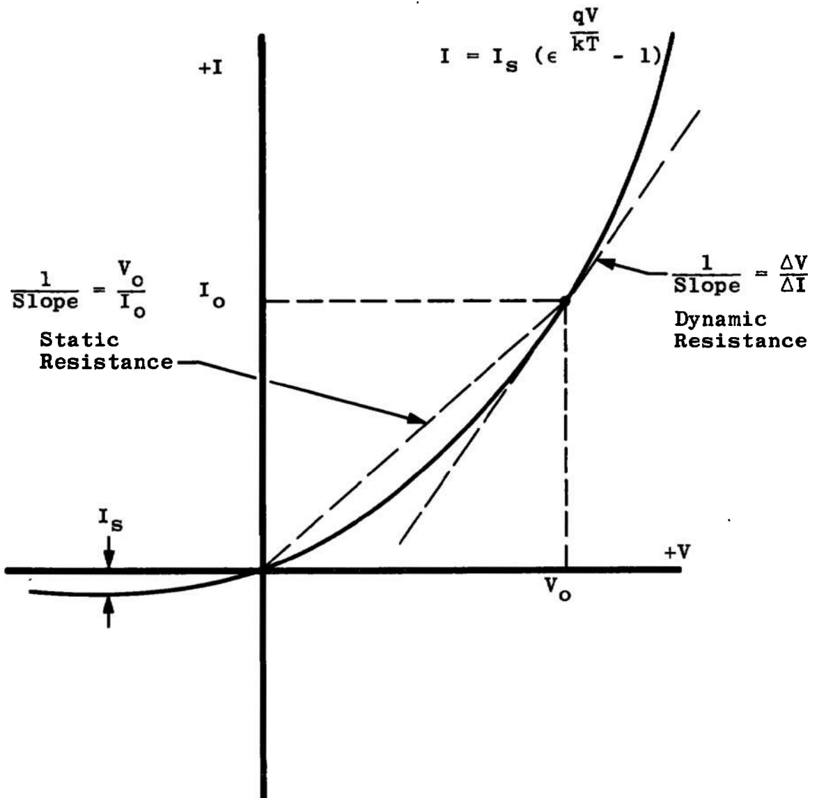
Figure 2. Graphical method for determining static and dynamic resistance of a diode.
