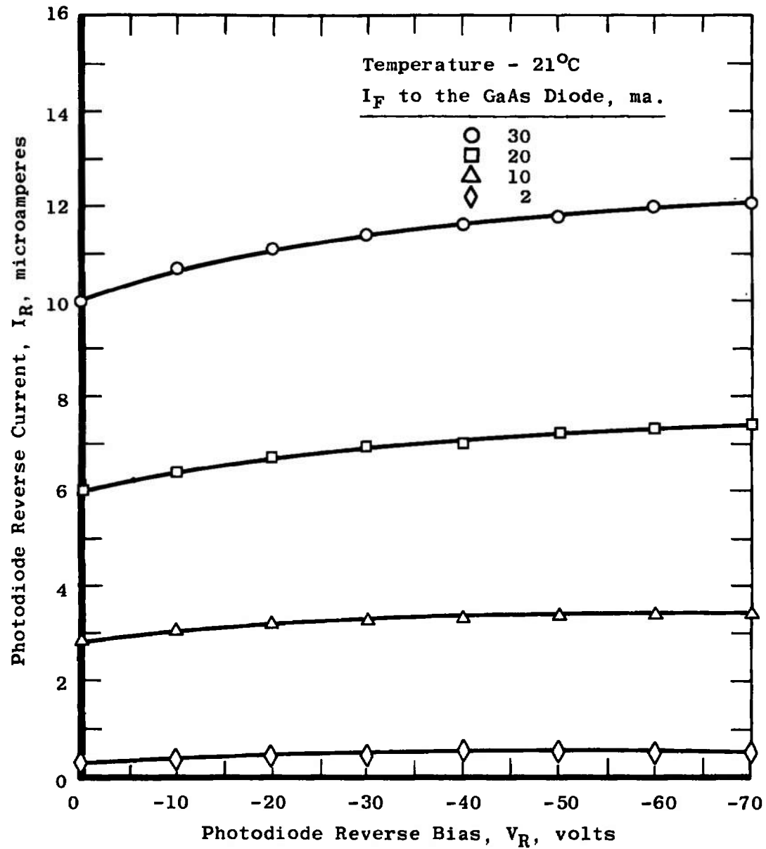
Figure 18. Photodiode reverse current versus reverse voltage for constant GaAs input current.
