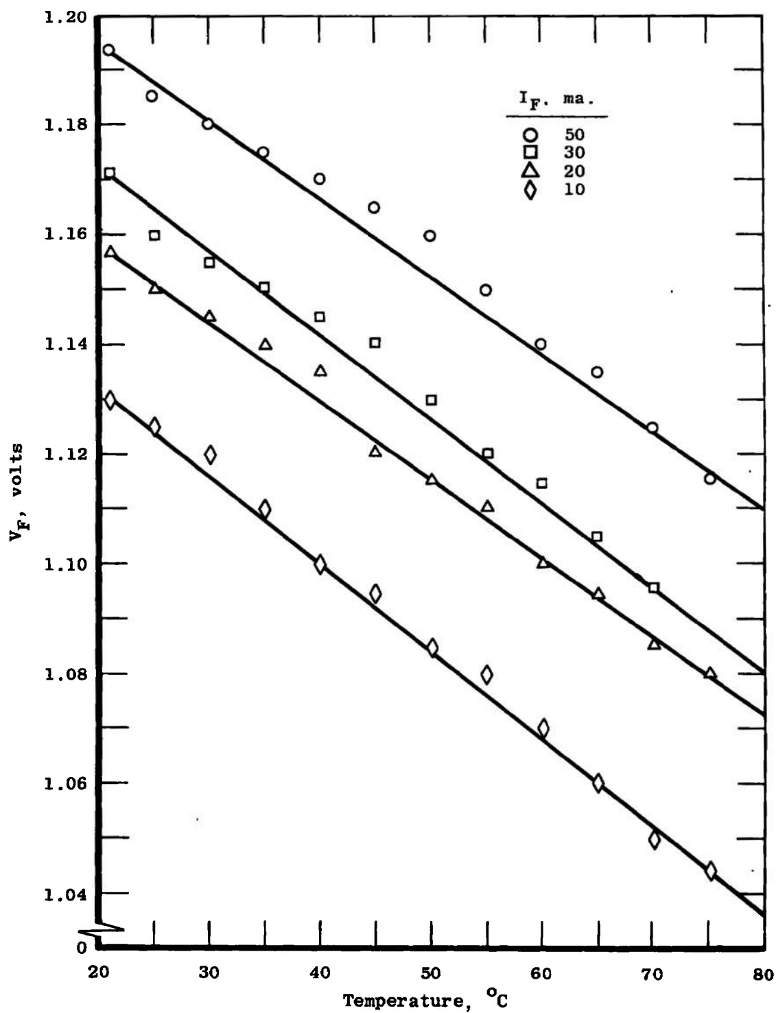
Figure 12. GaAs forward voltage versus temperature change for constant forward current.
