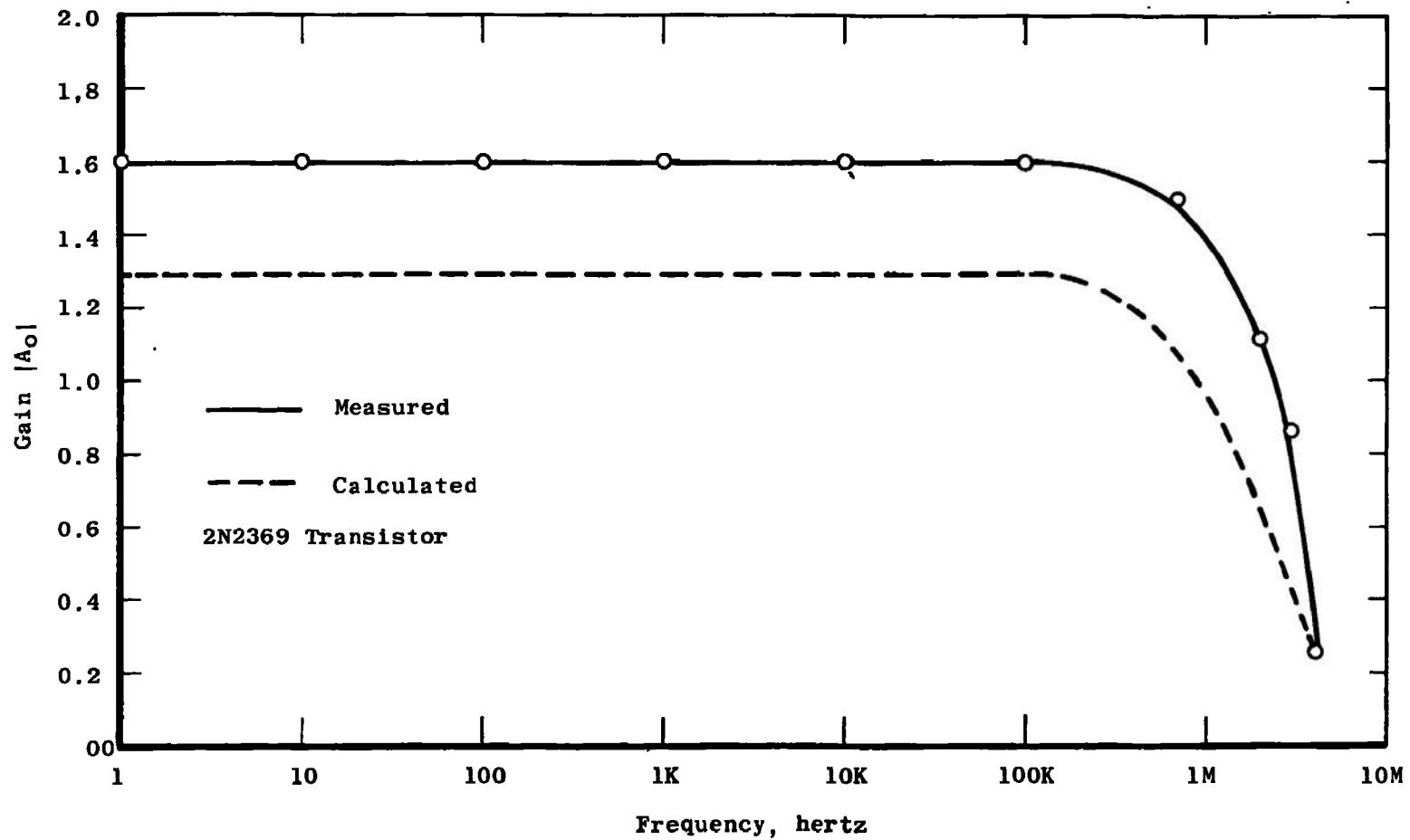
Figure 9. Frequency response of the isolator-preamplifier.
