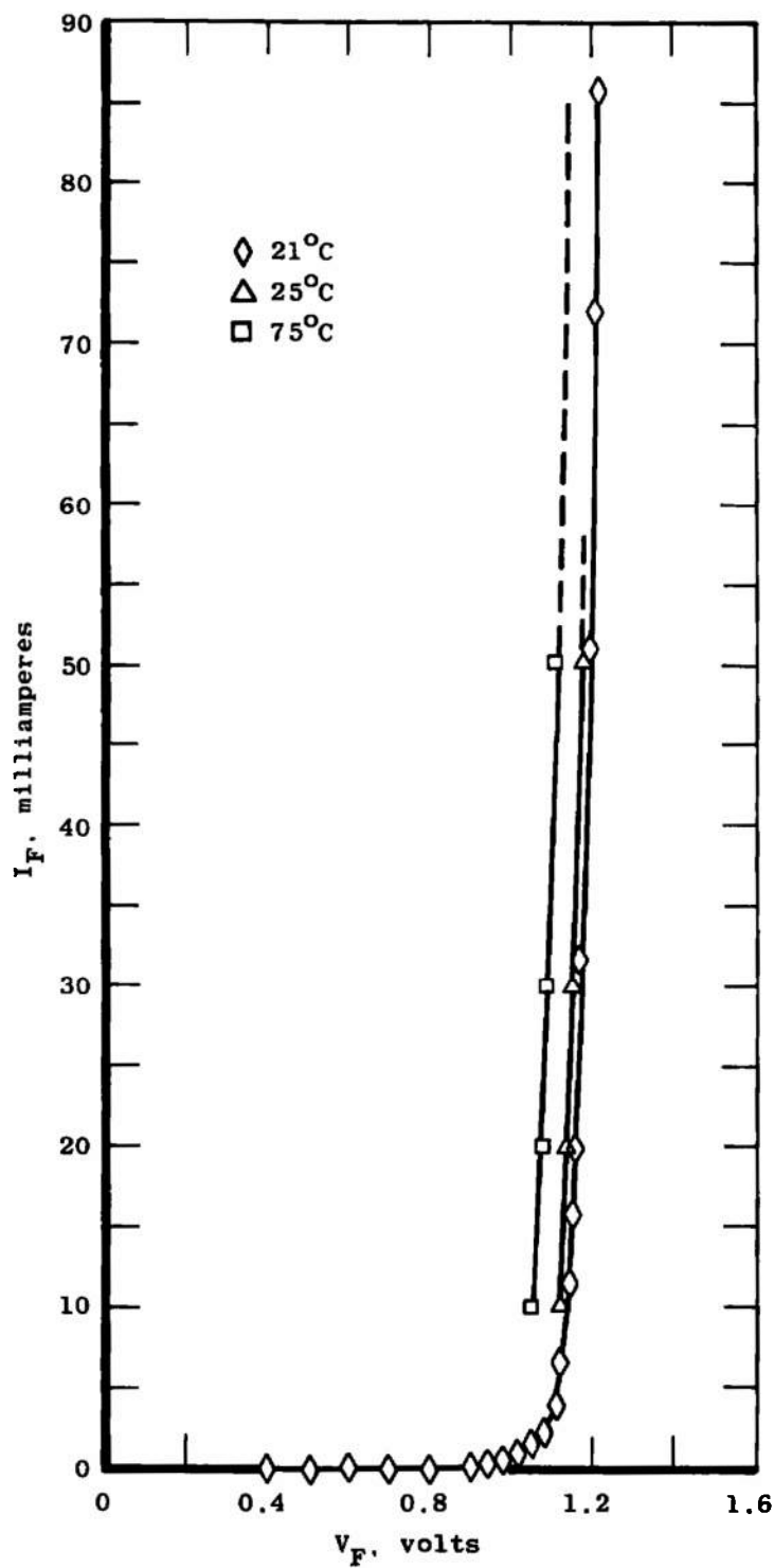
Figure 11. GaAs forward current versus forward voltage for varying temperature.
