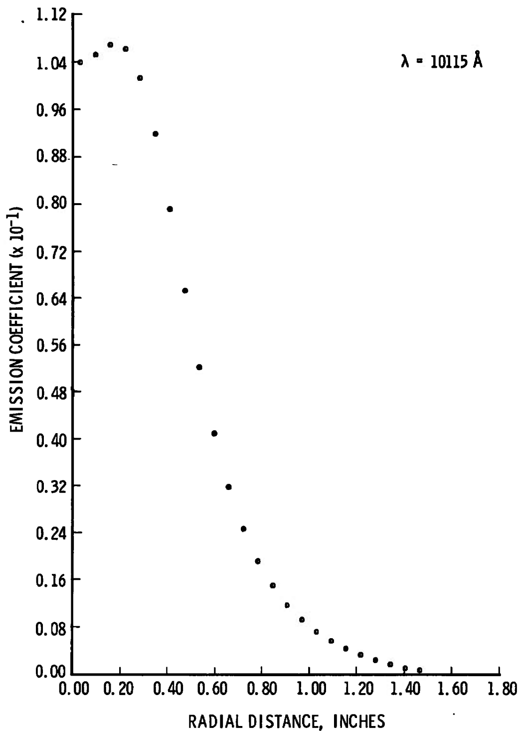
Fig. 17 Emission Coefficient Profile for the 10,115-Å Line
