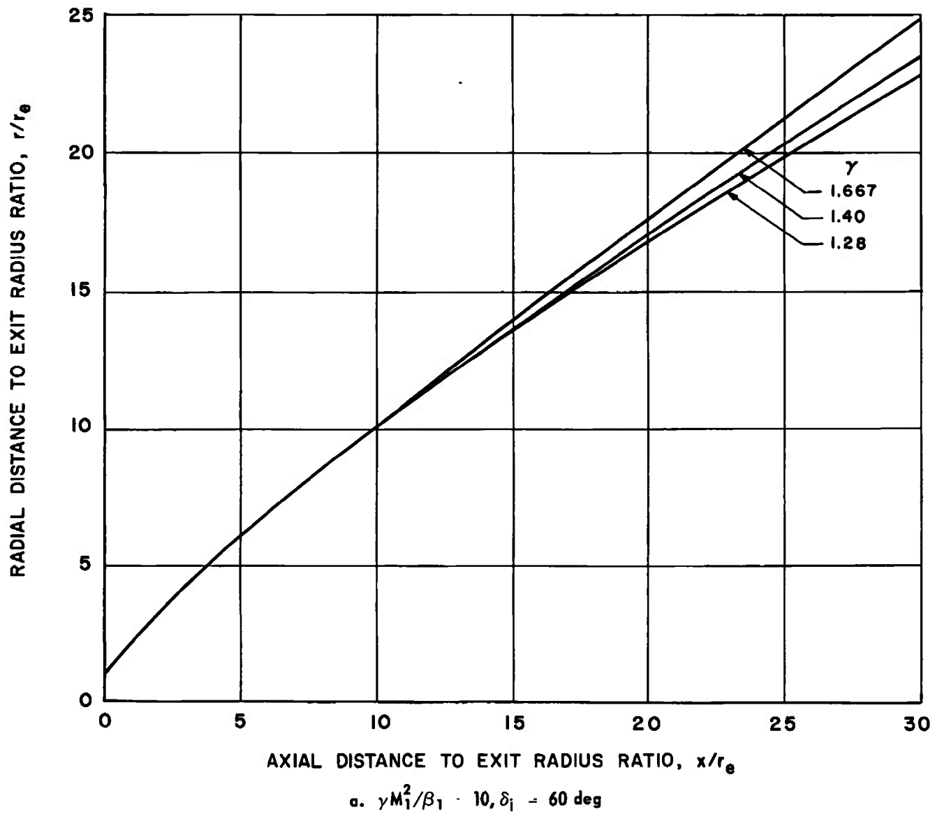
Fig. 8 Comparison of Jet Boundaries as Determined by the Latvala Approximation
