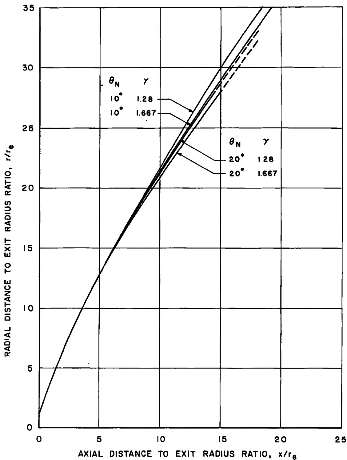
Fig. 18 Comparison of Jet Boundaries as Determined by a Method-of-Characteristics Solution for \delta_i = 75^\circ
