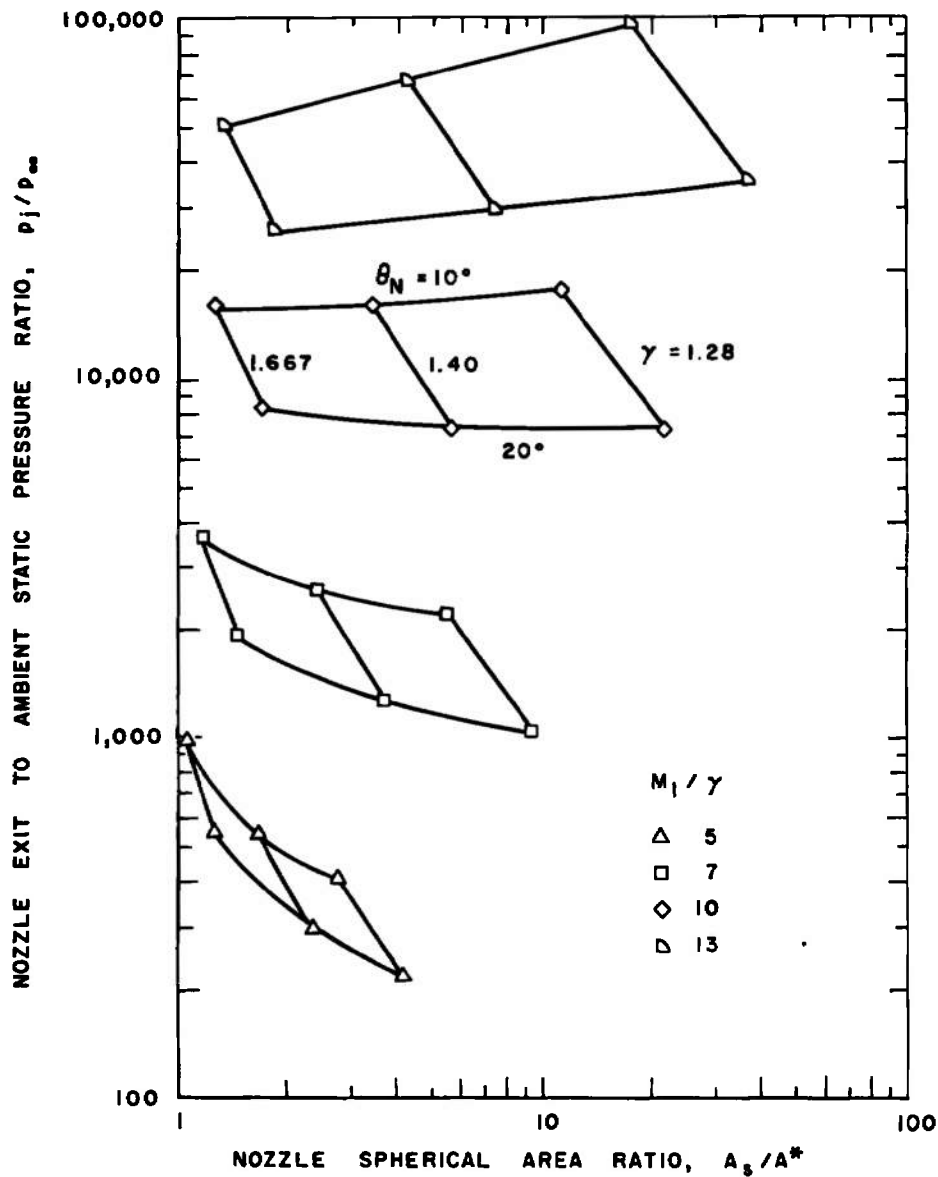
Fig. 17 Range of Nozzle Area Ratio and Exit Pressure Ratio for Jets with Constant Values of M_1/\gamma
