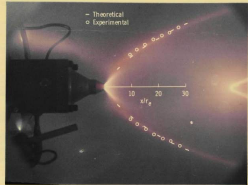
b. \text{N}_2 , \delta_1 = 60 \text{ deg} , \theta_N = 10 \text{ deg}
