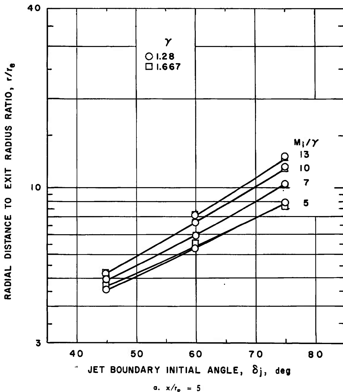
Fig. 21 Effect of the Boundary Initial Angle on the Jet Radius at a Given Axial Distance for Nozzles with \theta_N = 10 deg
