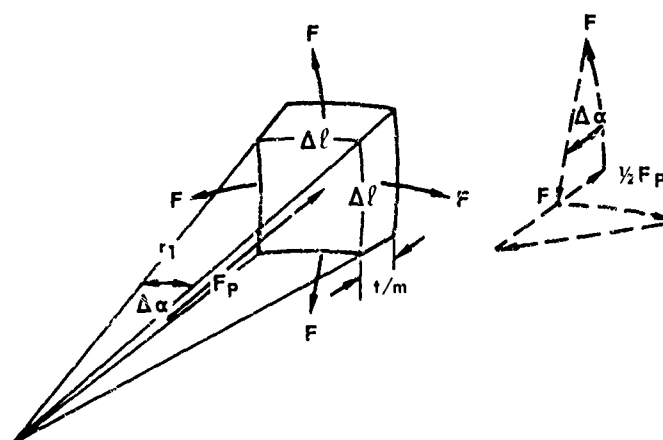
Fig. 2 STRAINED DIAPHRAGM
