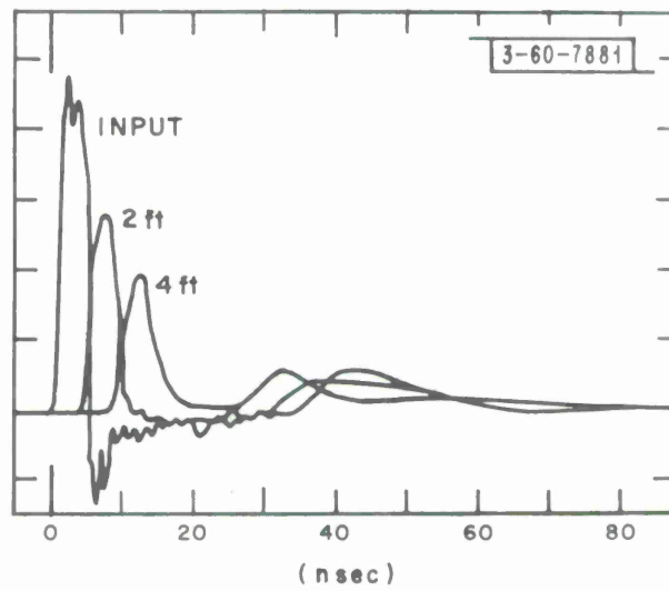
Fig. 2. Oscilloscope displays obtained with a 5-nsec pulse propagating through illite of 5% water content.
