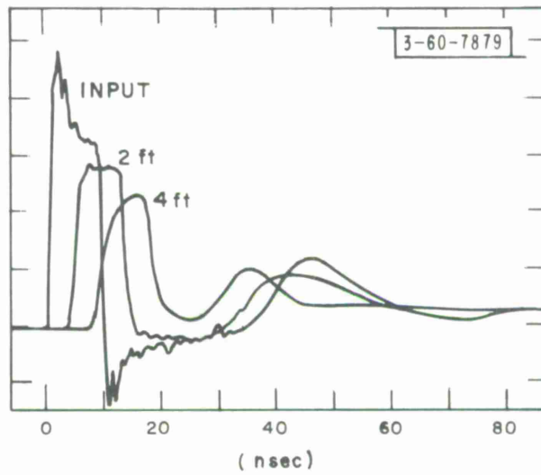
Fig. 1. Oscilloscope displays obtained with a 10-nsec pulse propagating through illite of 5% water content.
