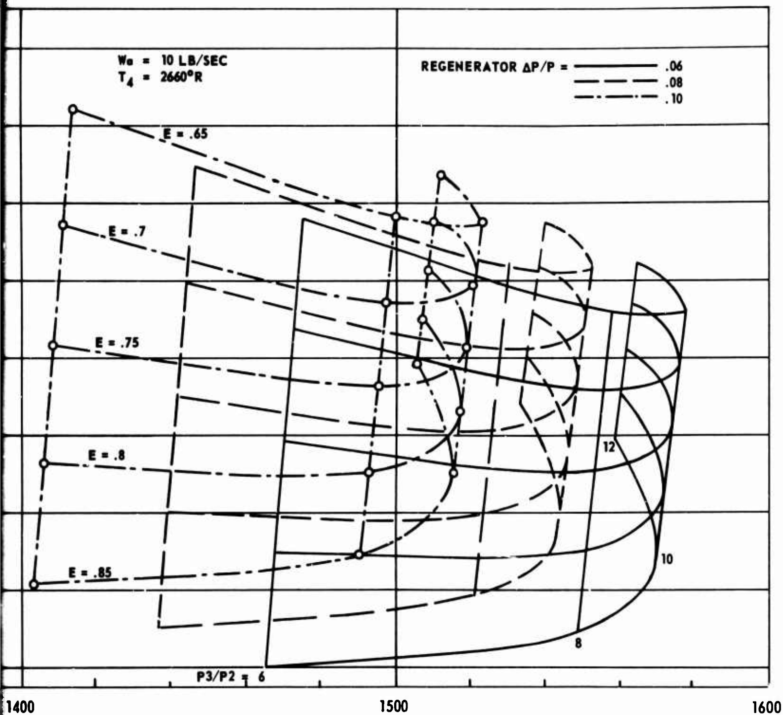
7. The effect of P_3/P_2 , regenerator \Delta P/P & regenerator effectiveness on regenerative engine SHP & BSFC, 6000 feet static, T_{\text{ambient}} = 95^\circ\text{F} .
