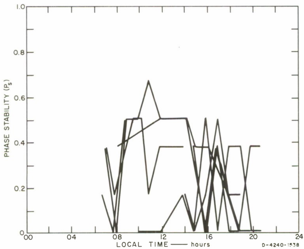
FIG. 148 DIURNAL VARIATION OF PULSE STABILITY, 5.1-MHz ORDINARY WAVE VIA F LAYER
