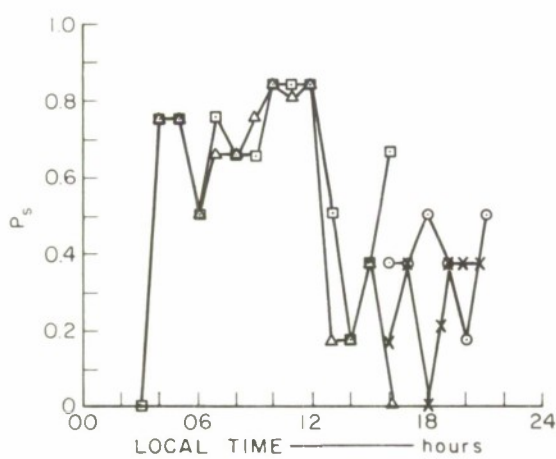
FIG. 119 3.4-MHz PULSE DATA, CHOLBURI/SATTAHIP CIRCUIT: N-S TRANSMITTING, 83 km
