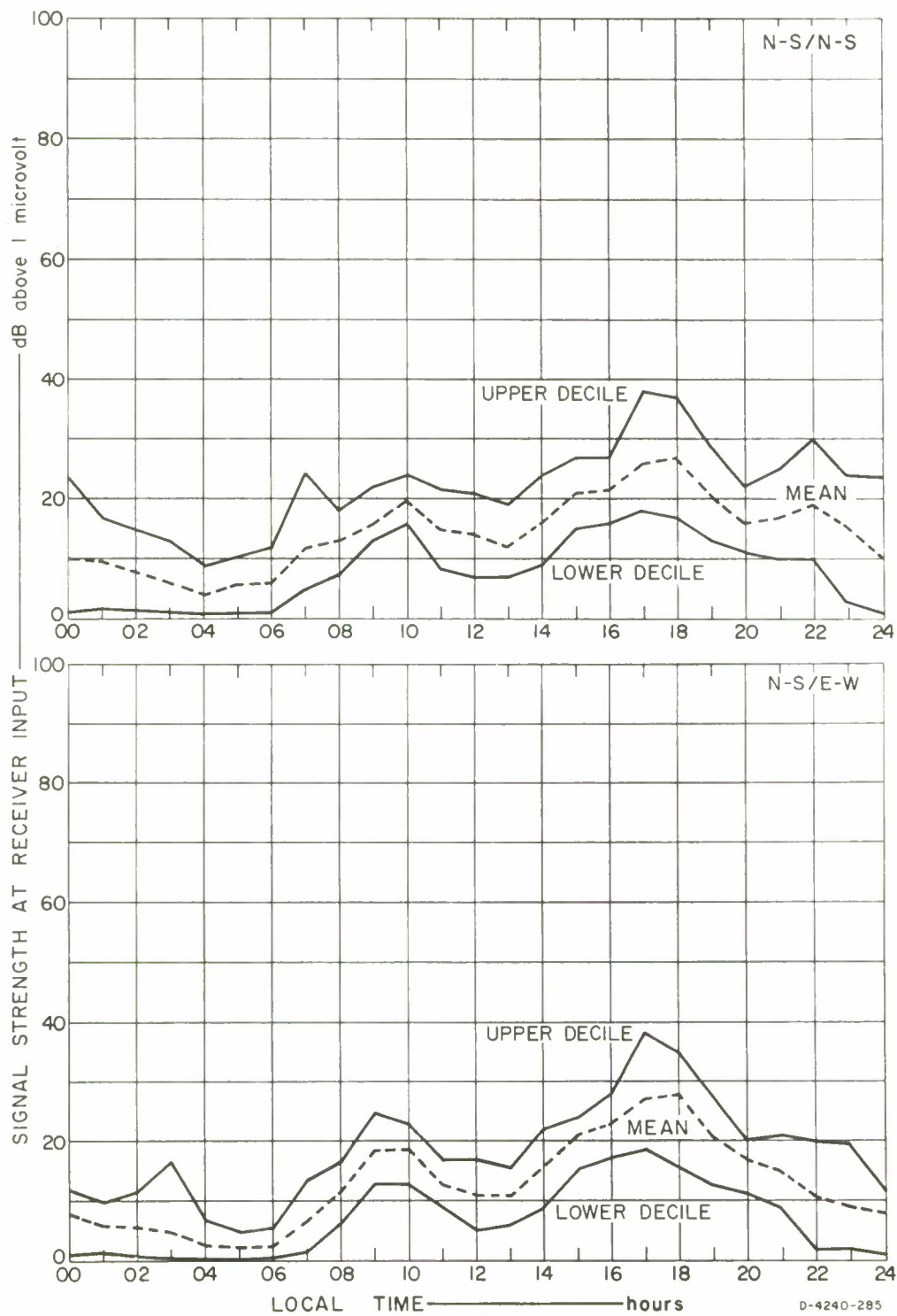
FIG. 42 NAKORNPATHEM: 10 MHz CW, N-S TRANSMITTING
