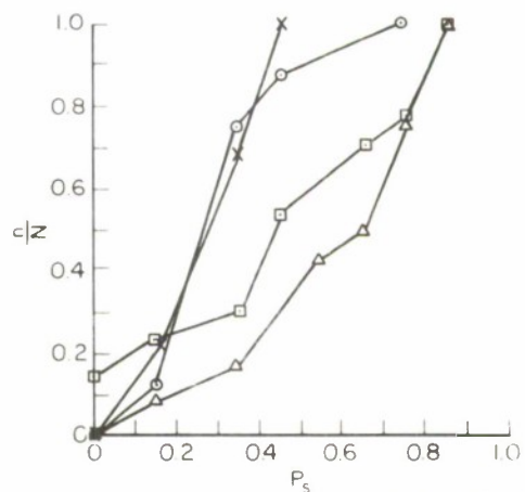
FIG. 121 3.4-MHz PULSE DATA, CHOLBURI/SATTAHIP CIRCUIT: NE-SW TRANSMITTING, 83 km
