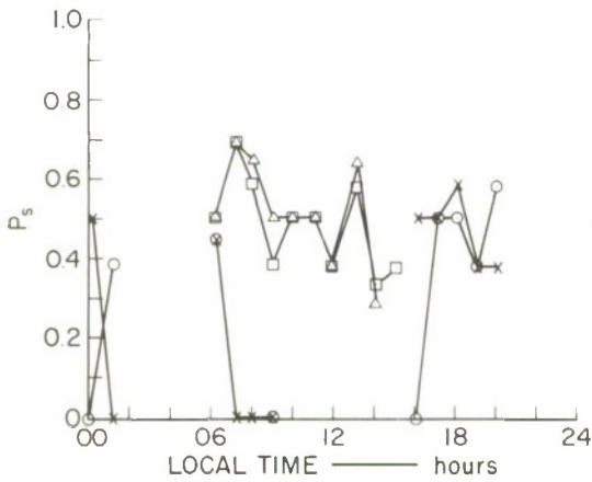
FIG. 138 3.4-MHz PULSE DATA, KAO PONGRANG/KRABINBURI CIRCUIT: NE-SW TRANSMITTING, 109 km
