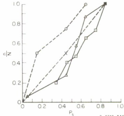
FIG. 113 3.4-MHz PULSE DATA, CHOLBURI/SATTAHIP CIRCUIT: N-S TRANSMITTING, 43 km
