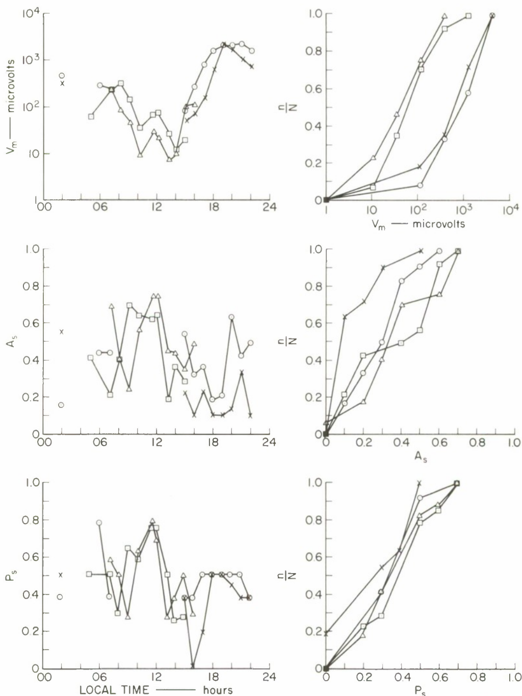
FIG. 130 3.4-MHz PULSE DATA, KAO PONGRANG/KRABINBURI CIRCUIT: N-S TRANSMITTING, 59 km
