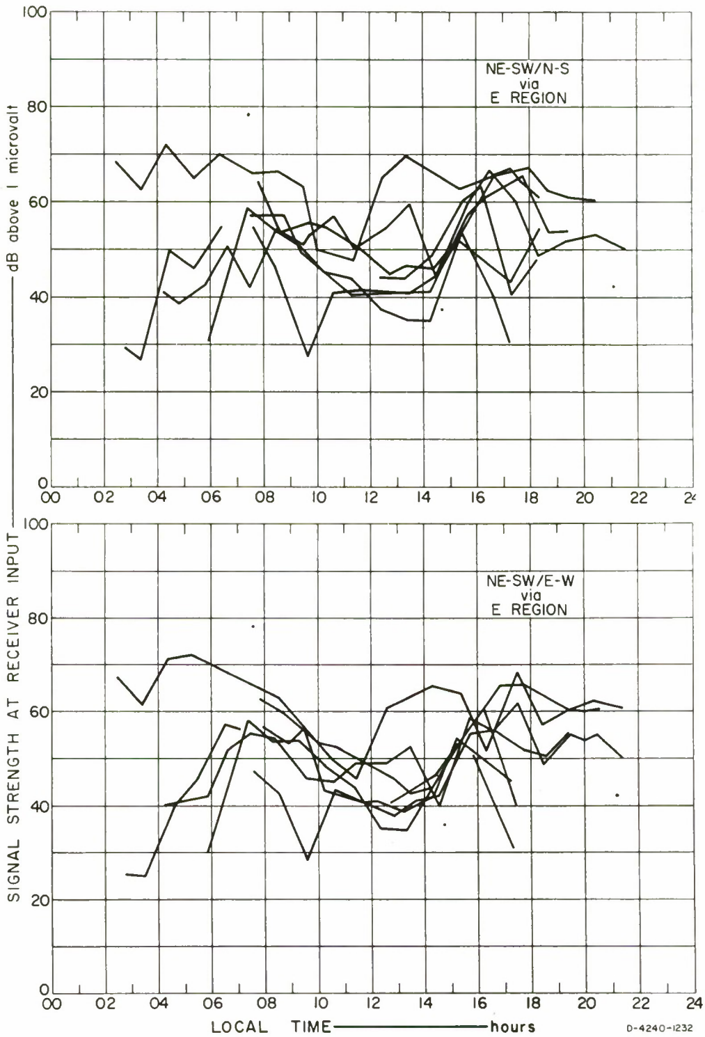
FIG. 106 DIRUNAL VARIATION OF V_m : SATTAHIP, NE-SW TRANSMITTING AT 3.4 MHz
