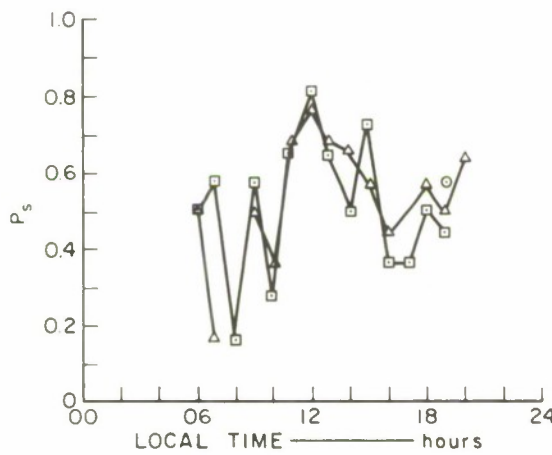
FIG. 96 3.4-MHz PULSE DATA, SATTAHIP/CHOLBURI CIRCUIT: NE-SW TRANSMITTING, 49 km
