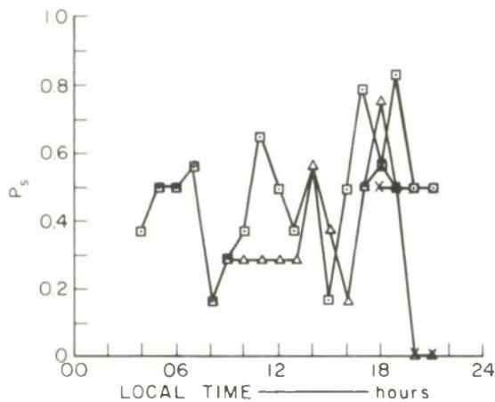
FIG. 82 3.4-MHz PULSE DATA, SATTAHIP/CHOLBURI CIRCUIT: N-S TRANSMITTING, 15 km
