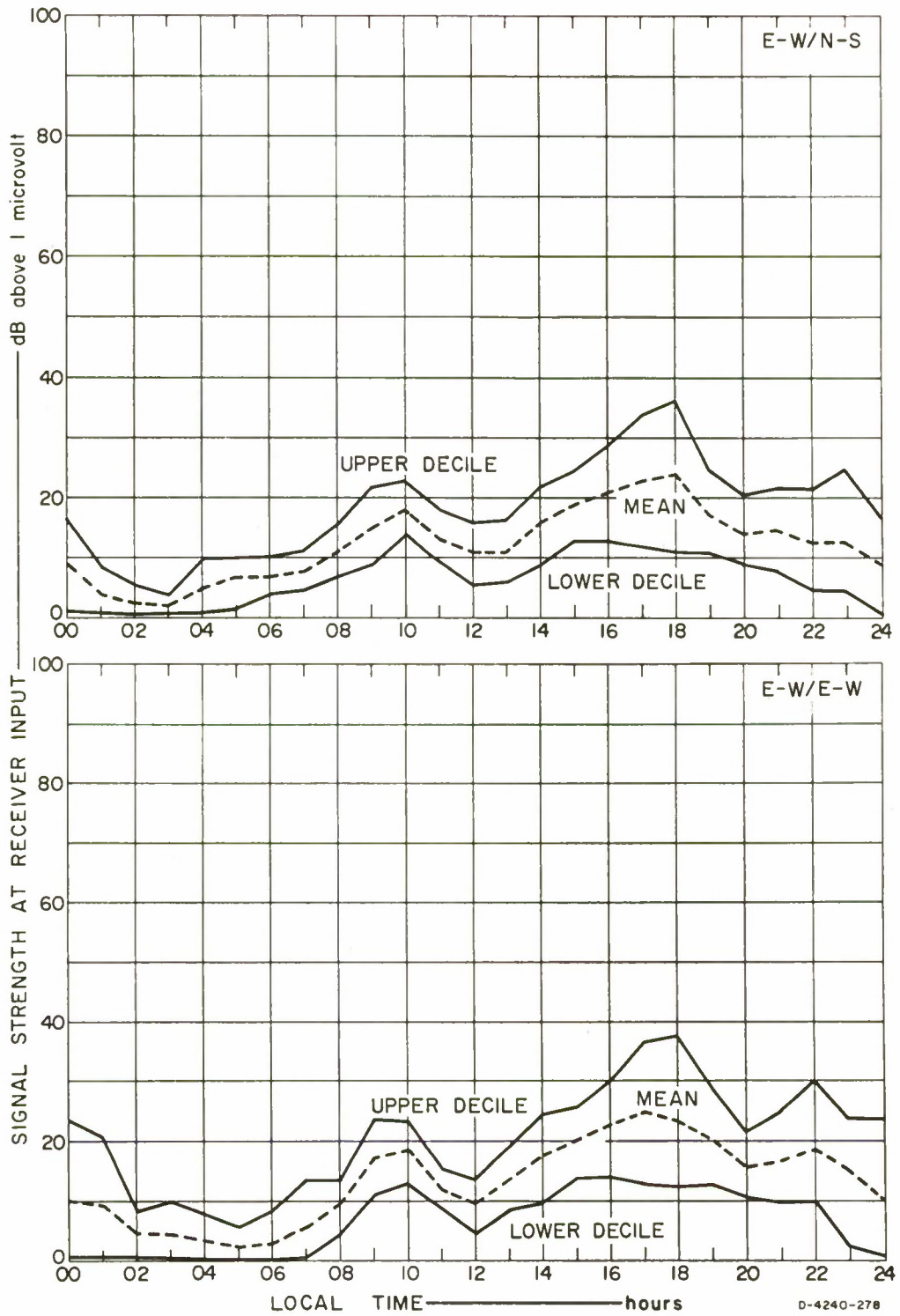
FIG. 35 AYUDHAYA: 10 MHz CW, E-W TRANSMITTING
