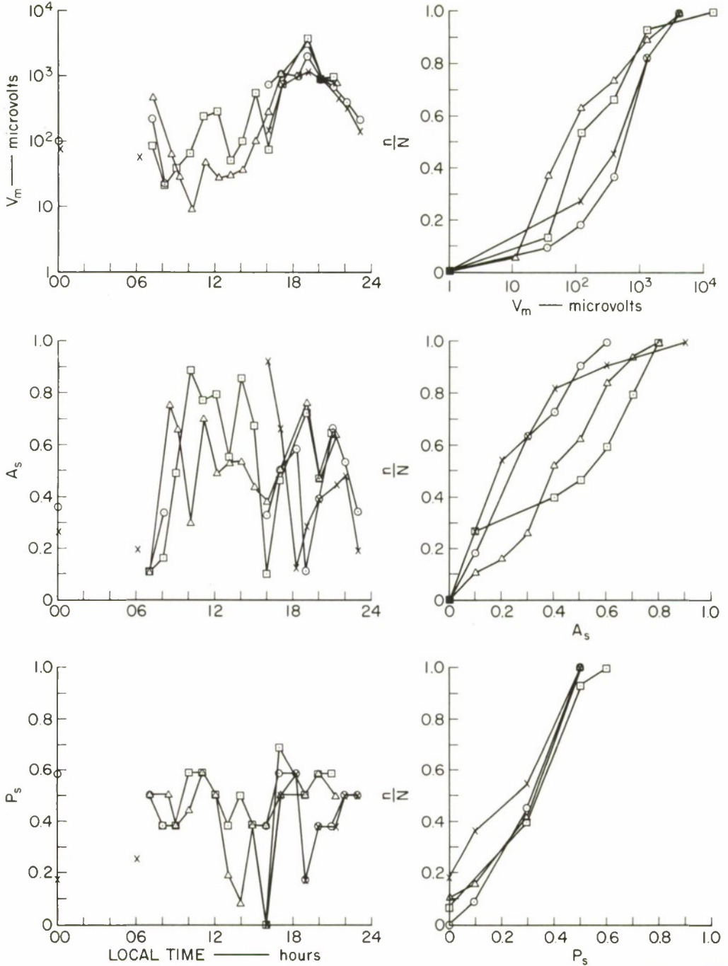
FIG. 127 3.4-MHz PULSE DATA, KAO PONGRANG/KRABINBURI CIRCUIT: N-S TRANSMITTING, 45 km
