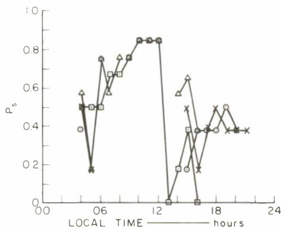
FIG. 121 3.4-MHz PULSE DATA, CHOLBURI/SATTAHIP CIRCUIT: NE-SW TRANSMITTING, 83 km
