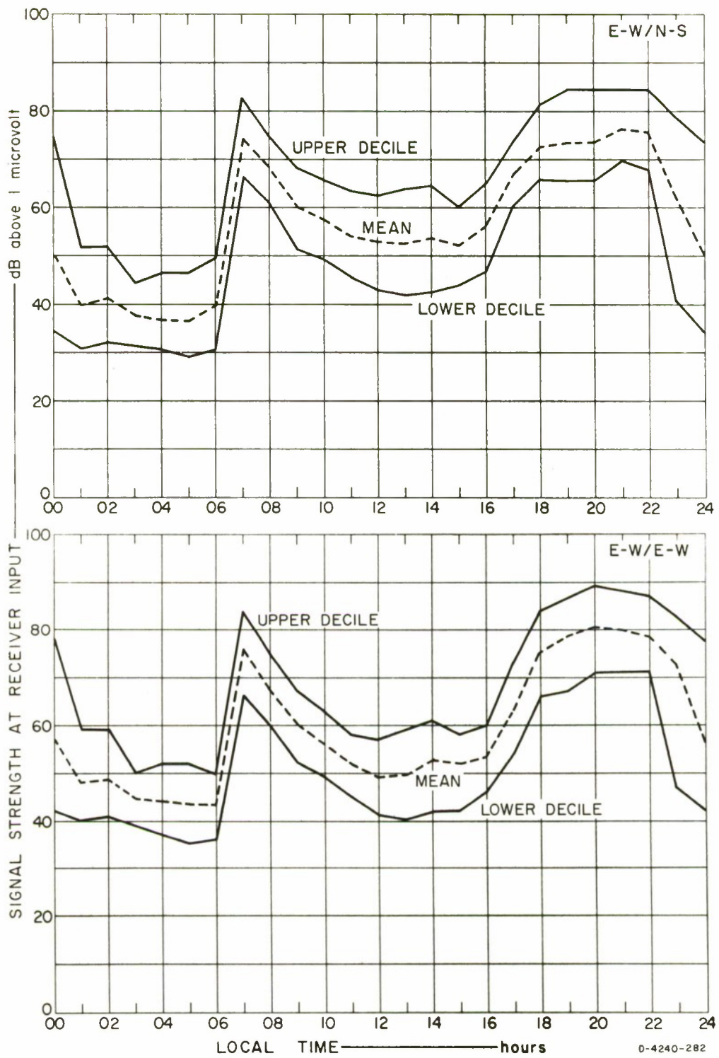
FIG. 39 NAKORNPATOM: 3 MHz CW, E-W TRANSMITTING
