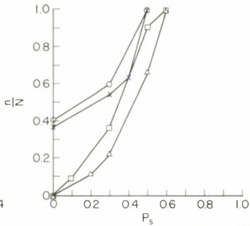
FIG. 138 3.4-MHz PULSE DATA, KAO PONGRANG/KRABINBURI CIRCUIT: NE-SW TRANSMITTING, 109 km
