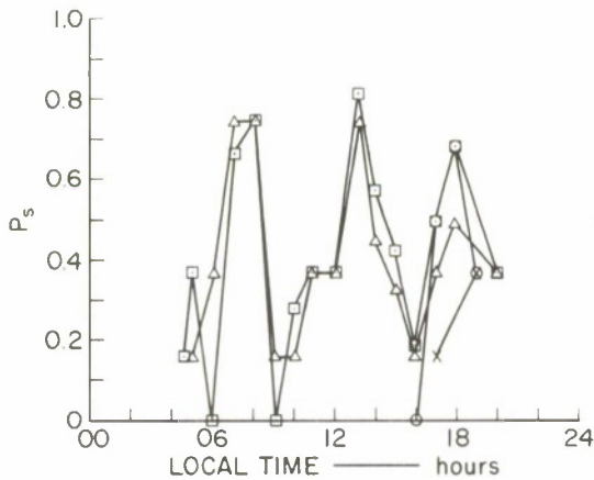
FIG. 124 3.4-MHz PULSE DATA, KAO PONGRANG/KRABINBURI CIRCUIT: N-S TRANSMITTING, 26 km
