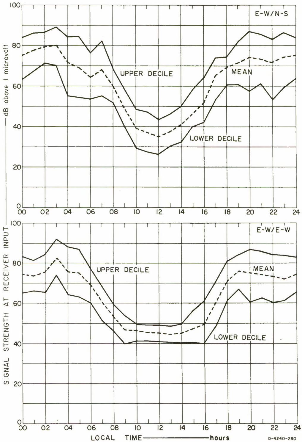
FIG. 37 NAKORNPATTHOM: 1.7 MHz CW, E-W TRANSMITTING
