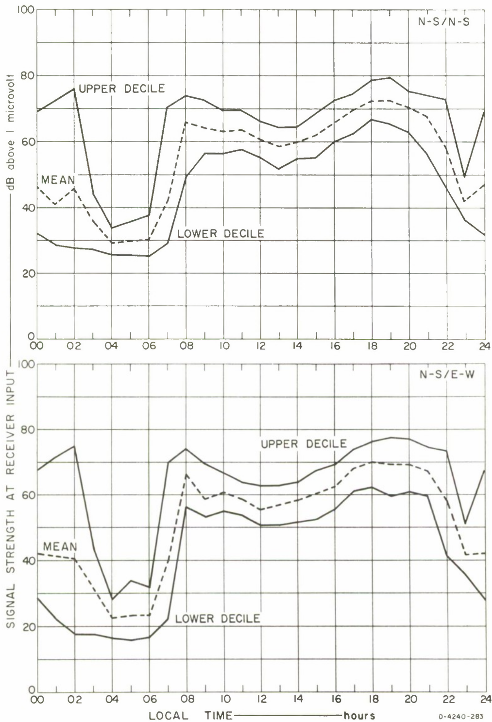
FIG. 40 NAKORNPATHEM: 5 MHz CW, N-S TRANSMITTING
