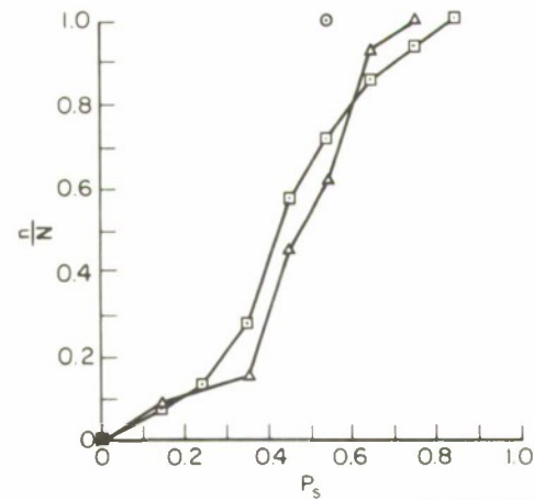
FIG. 96 3.4-MHz PULSE DATA, SATTAHIP/CHOLBURI CIRCUIT: NE-SW TRANSMITTING, 49 km
