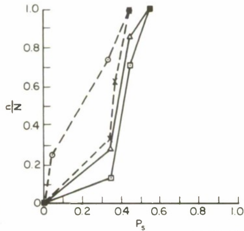
FIG. 100 3.4-MHz PULSE DATA, SATTAHIP/CHOLBURI CIRCUIT: N-S TRANSMITTING, 83 km
