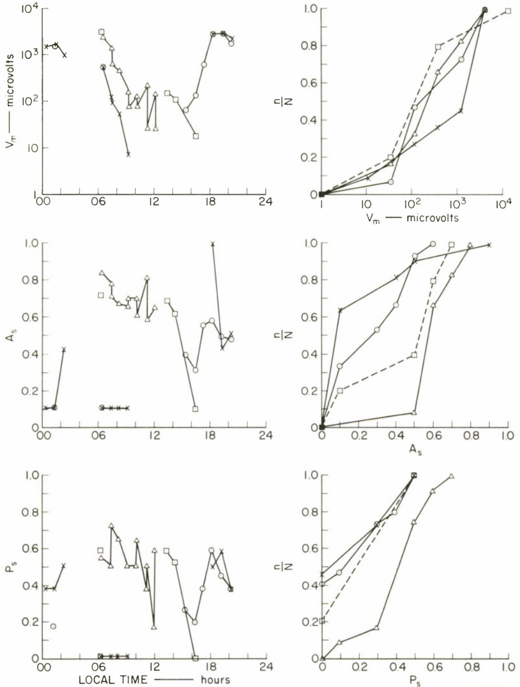
FIG. 137 3.4-MHz PULSE DATA, KAO PONGRANG/KRABINBURI CIRCUIT: E-W TRANSMITTING, 109 km
