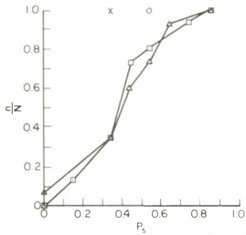
FIG. 94 3.4-MHz PULSE DATA, SATTAHIP/CHOLBURI CIRCUIT: N-S TRANSMITTING, 49 km
