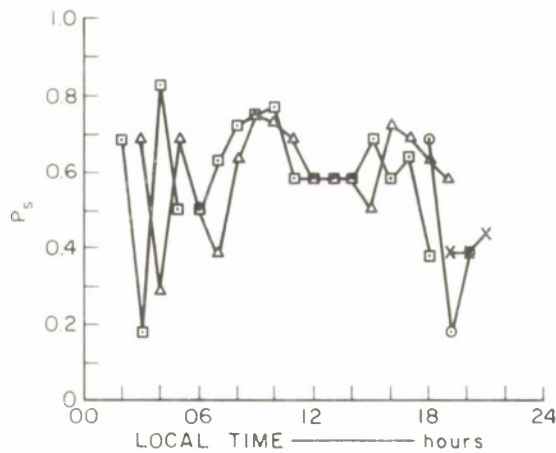
FIG. 92 3.4-MHz PULSE DATA, SATTAHIP/CHOLBURI CIRCUIT: E-W TRANSMITTING, 40 km
