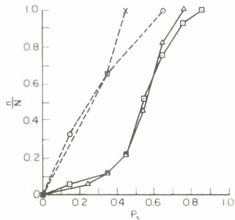
FIG. 92 3.4-MHz PULSE DATA, SATTAHIP/CHOLBURI CIRCUIT: E-W TRANSMITTING, 40 km
