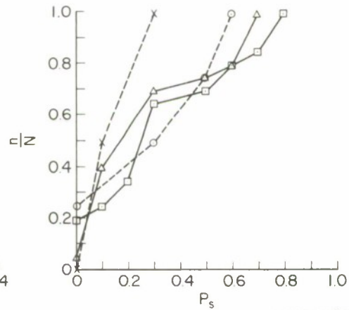
FIG. 124 3.4-MHz PULSE DATA, KAO PONGRANG/KRABINBURI CIRCUIT: N-S TRANSMITTING, 26 km
