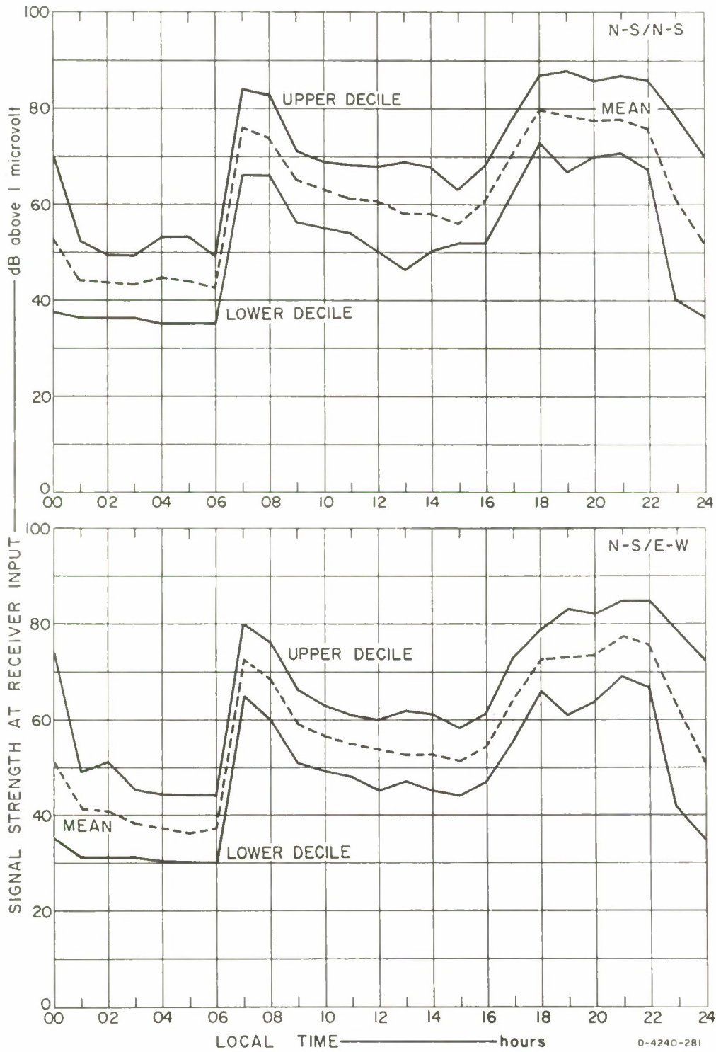
FIG. 38 NAKORNPATTHOM: 3 MHz CW, N-S TRANSMITTING
