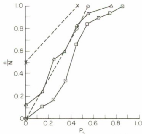
FIG. 82 3.4-MHz PULSE DATA, SATTAHIP/CHOLBURI CIRCUIT: N-S TRANSMITTING, 15 km
