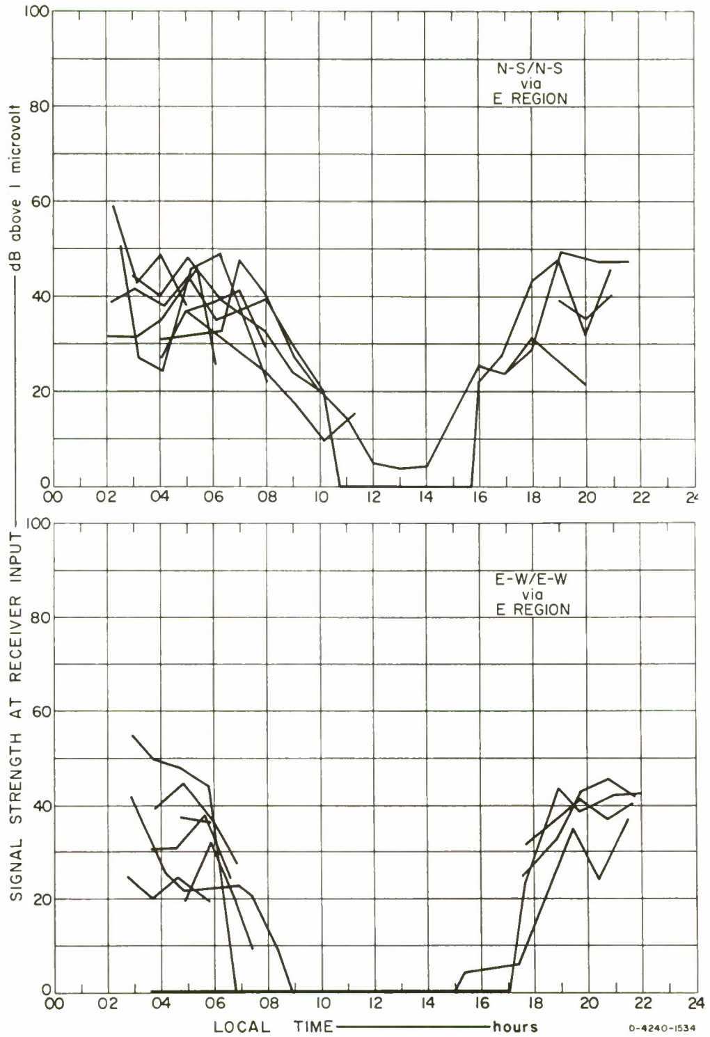
FIG. 144 DIRURNAL VARIATION OF V_m : SATTAHIP, N-S AND E-W TRANSMITTING AT 1.7 MHz
