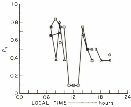
FIG. 97 3.4-MHz PULSE DATA, SATTAHIP/CHOLBURI CIRCUIT: N-S TRANSMITTING, 59 km
