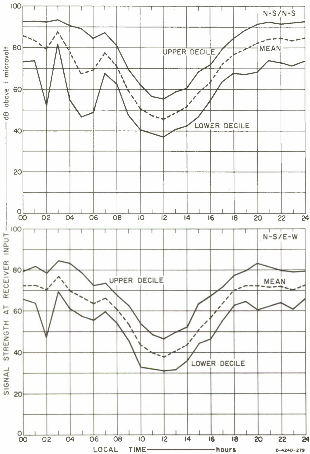
FIG. 36 NAKORNPATHOM: 1.7 MHz CW, N-S TRANSMITTING
