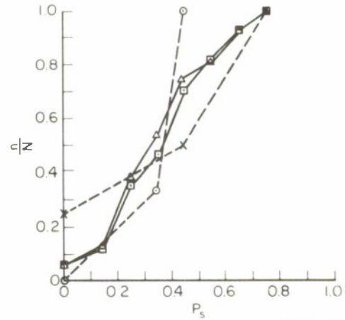
FIG. 84 3.4-MHz PULSE DATA, SATTAHIP/CHOLBURI CIRCUIT: NE-SW TRANSMITTING, 15 km
