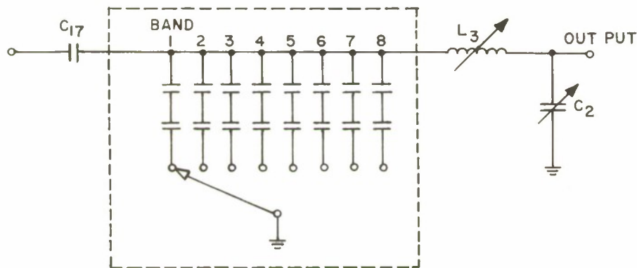
C_{1\pi} SWITCHING ARRANGEMENT
