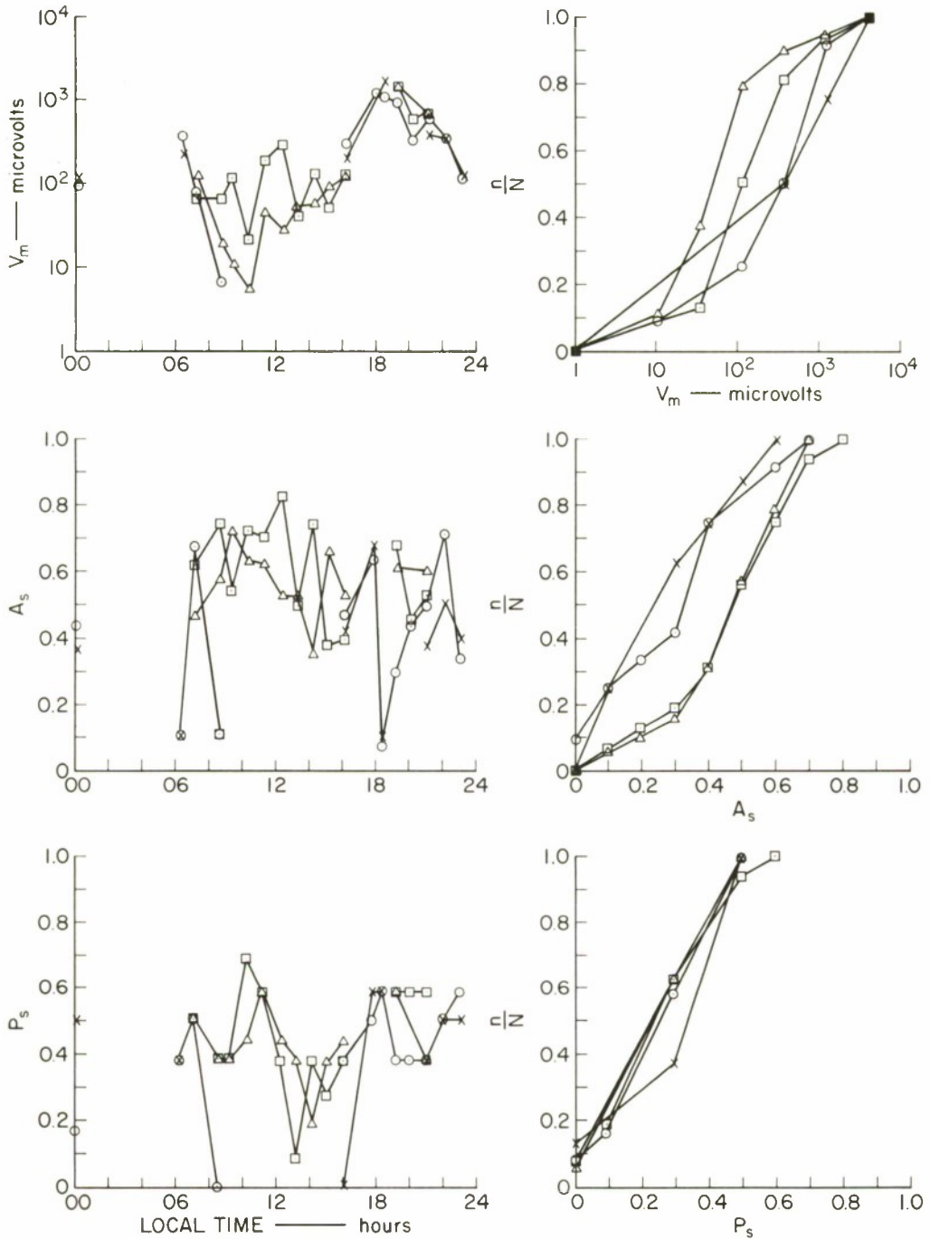
FIG. 129 3.4-MHz PULSE DATA, KAO PONGRANG/KRABINBURI CIRCUIT: NE-SW TRANSMITTING, 45 km
