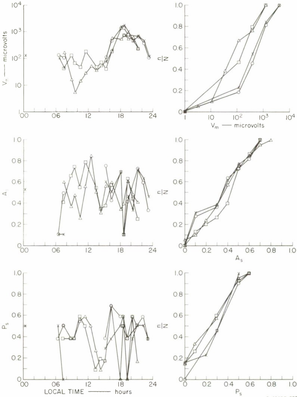
FIG. 128 3.4-MHz PULSE DATA, KAO PONGRANG/KRABINBURI CIRCUIT: E-W TRANSMITTING, 45 km
