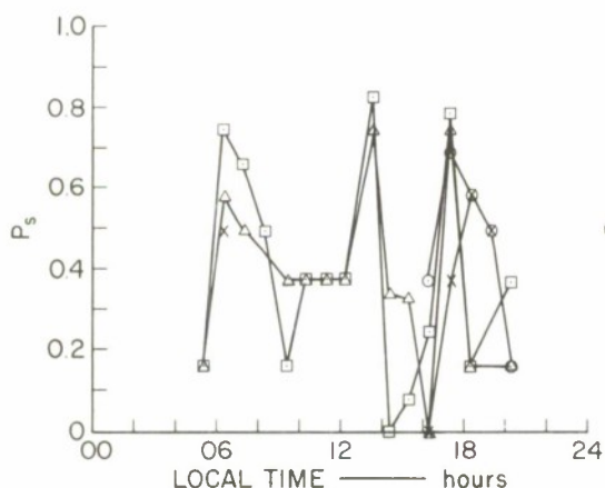
FIG. 126 3.4-MHz PULSE DATA, KAO PONGRANG/KRABINBURI CIRCUIT: NE-SW TRANSMITTING, 26 km
