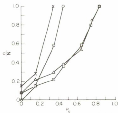
FIG. 119 3.4-MHz PULSE DATA, CHOLBURI/SATTAHIP CIRCUIT: N-S TRANSMITTING, 83 km
