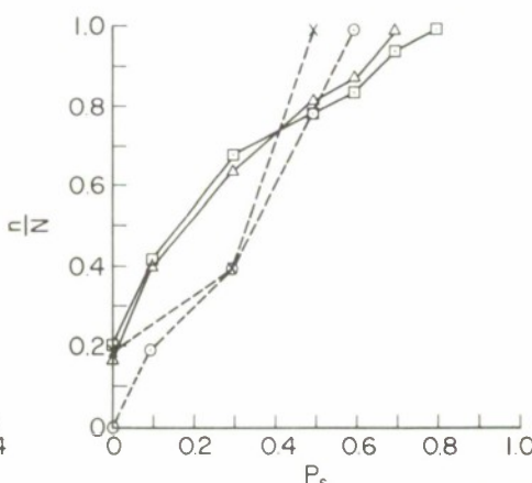
FIG. 126 3.4-MHz PULSE DATA, KAO PONGRANG/KRABINBURI CIRCUIT: NE-SW TRANSMITTING, 26 km
