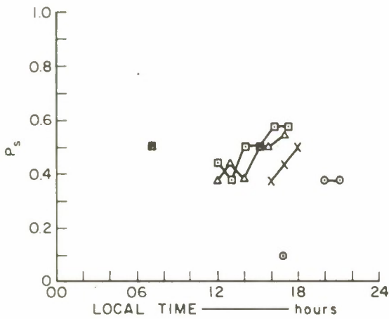
FIG. 100 3.4-MHz PULSE DATA, SATTAHIP/CHOLBURI CIRCUIT: N-S TRANSMITTING, 83 km
