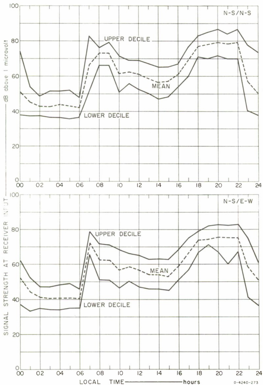
FIG. 30 AYUDHAYA: 3 MHz CW, N-S TRANSMITTING
