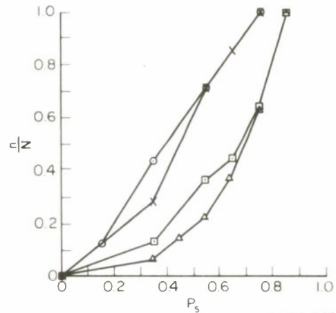
FIG. 90 3.4-MHz PULSE DATA, SATTAHIP/CHOLBURI CIRCUIT: NE-SW TRANSMITTING, 30 km
