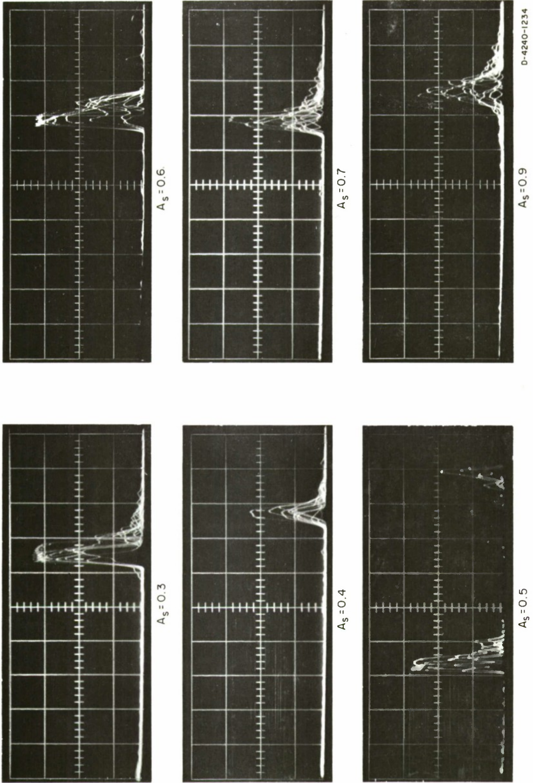
FIG. 103 AMPLITUDE STABILITY VALUES, A_s , OF PULSES
