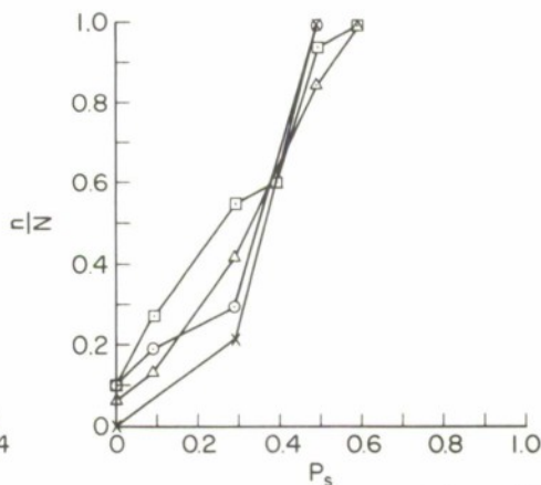
FIG. 134 3.4-MHz PULSE DATA, KAO PONGRANG/KRABINBURI CIRCUIT: E-W TRANSMITTING, 76 km
