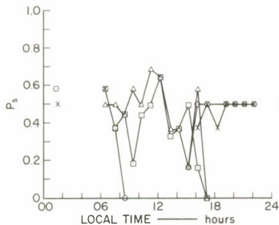
FIG. 134 3.4-MHz PULSE DATA, KAO PONGRANG/KRABINBURI CIRCUIT: E-W TRANSMITTING, 76 km
