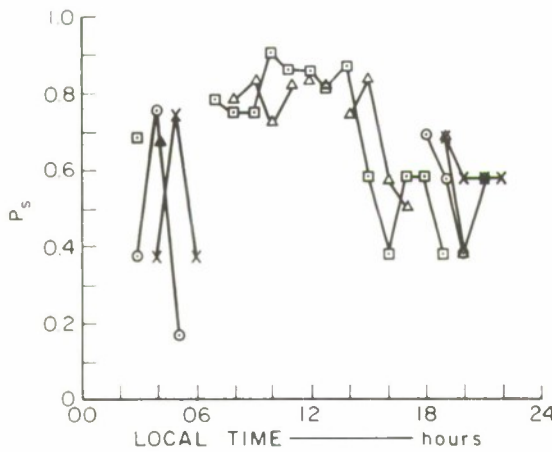
FIG. 90 3.4-MHz PULSE DATA, SATTAHIP/CHOLBURI CIRCUIT: NE-SW TRANSMITTING, 30 km
