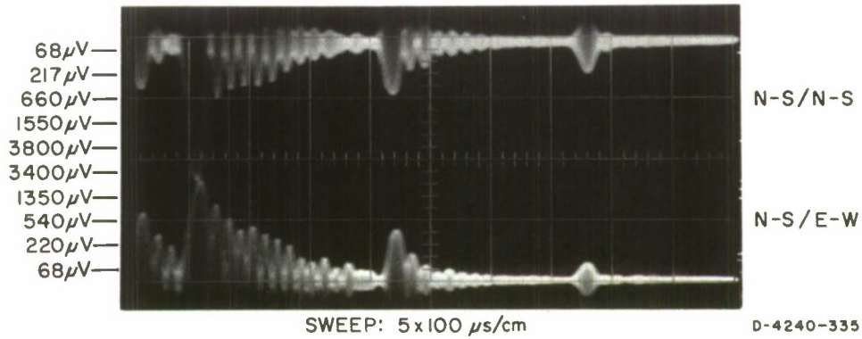
FIG. 73 PHOTOGRAPH OF RINGING OF SECOND IF 50\text{-}\mu\text{s} PULSE OUTPUT
