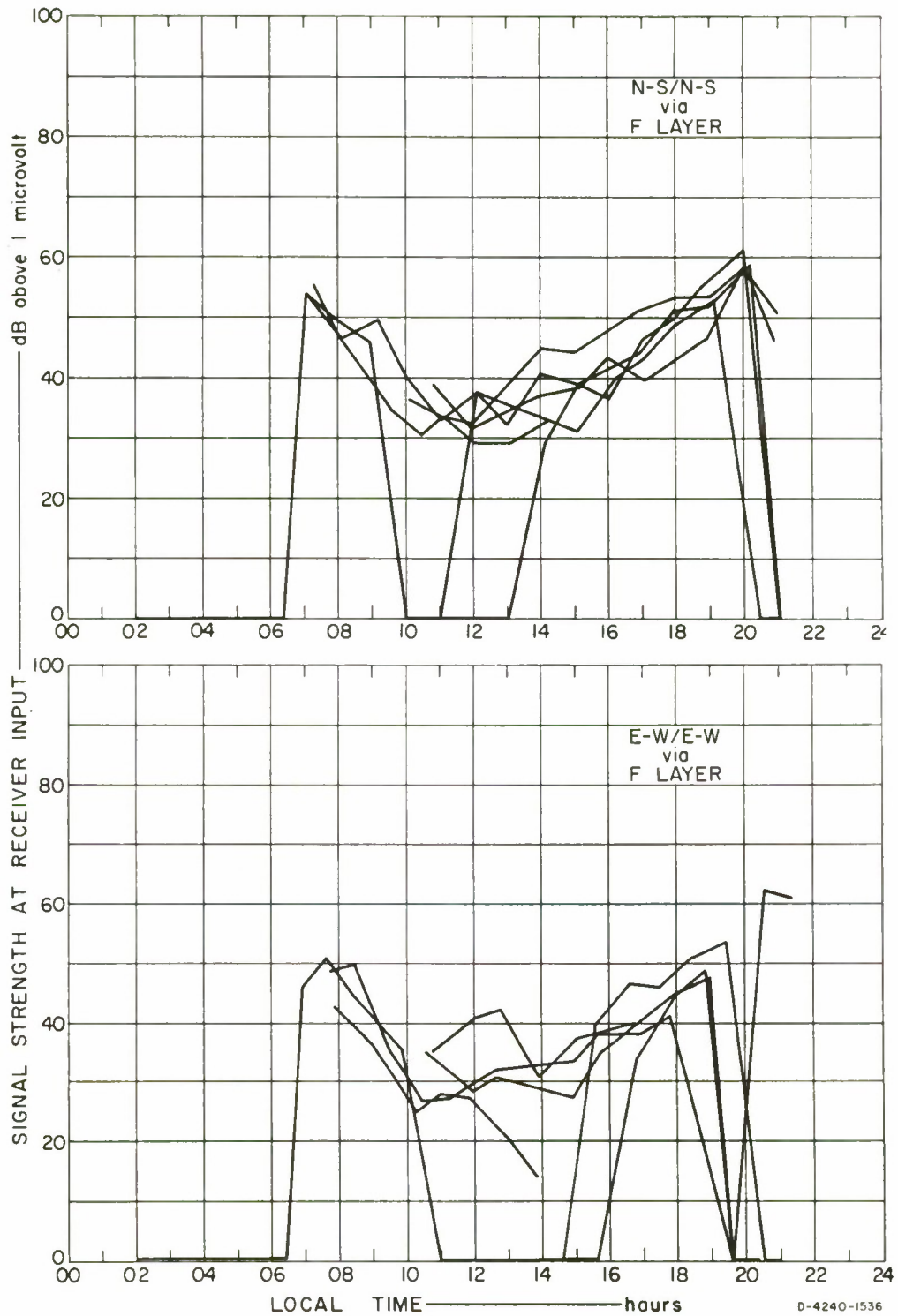
FIG. 146 DIRUNAL VARIATION OF V_m : SATTAHIP, N-S AND E-W TRANSMITTING AT 5.1 MHz
