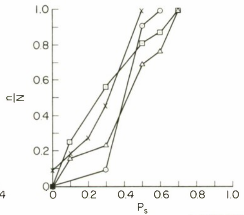
FIG. 131 3.4-MHz PULSE DATA, KAO PONGRANG/KRABINBURI CIRCUIT: E-W TRANSMITTING, 59 km
