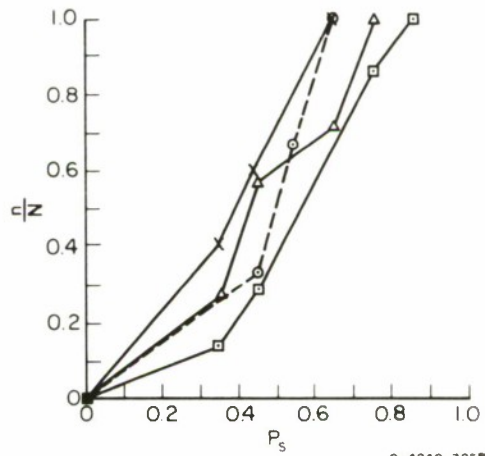
FIG. 97 3.4-MHz PULSE DATA, SATTAHIP/CHOLBURI CIRCUIT: N-S TRANSMITTING, 59 km
