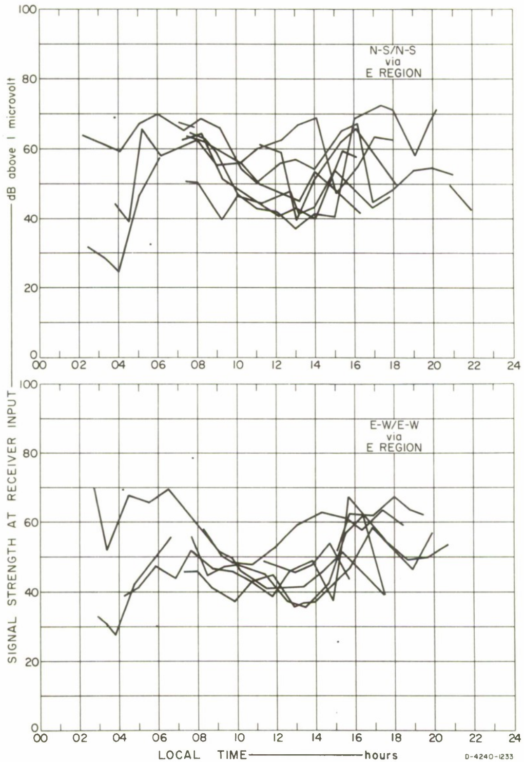
FIG. 105 DIURNAL VARIATION OF V_m : SATTAHIP, N-S AND E-W TRANSMITTING AT 3.4-MHz
