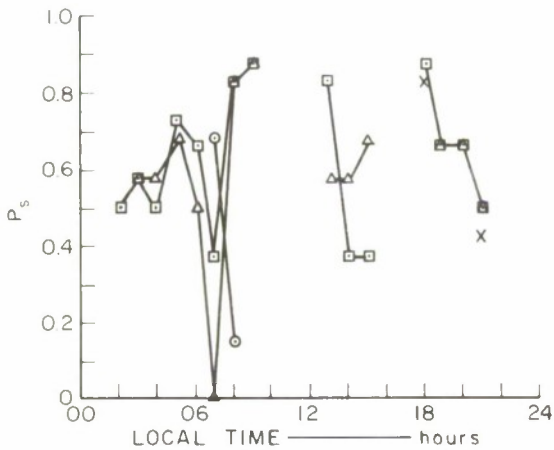
FIG. 113 3.4-MHz PULSE DATA, CHOLBURI/SATTAHIP CIRCUIT: N-S TRANSMITTING, 43 km
