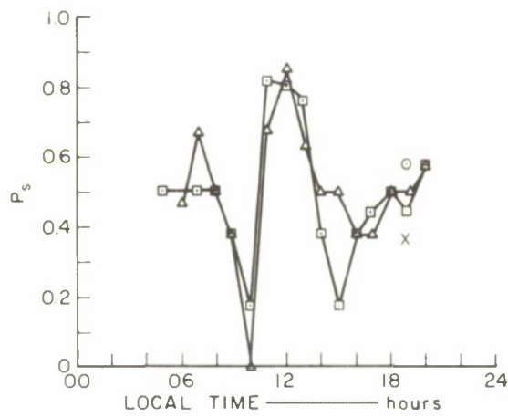
FIG. 94 3.4-MHz PULSE DATA, SATTAHIP/CHOLBURI CIRCUIT: N-S TRANSMITTING, 49 km
