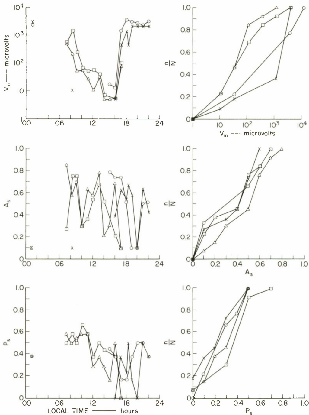
FIG. 133 3.4-MHz PULSE DATA, KAO PONGRANG/KRABINBURI CIRCUIT: N-S TRANSMITTING, 76 km
