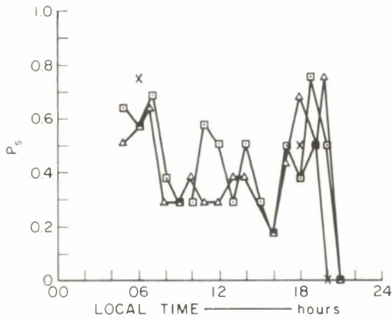
FIG. 84 3.4-MHz PULSE DATA, SATTAHIP/CHOLBURI CIRCUIT: NE-SW TRANSMITTING, 15 km
