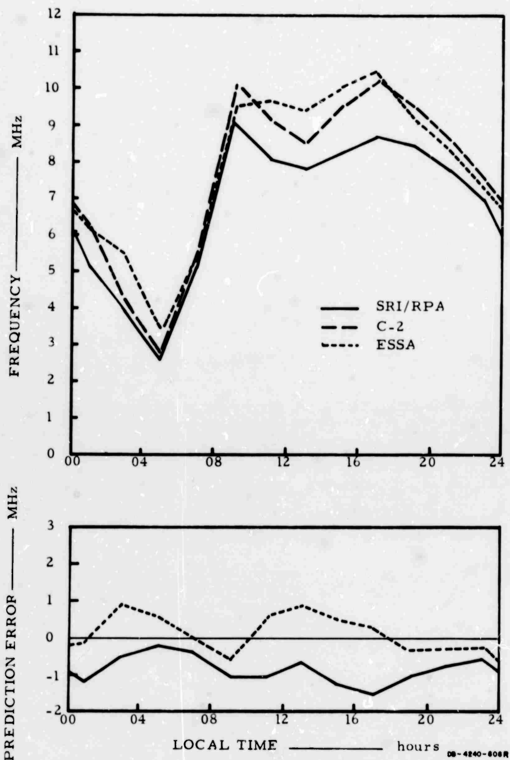
FIG. 1 COMPARISON OF OBSERVED AND PREDICTED MONTHLY MEDIAN f_0F_2 AND ERROR FUNCTION FOR JANUARY 1967
