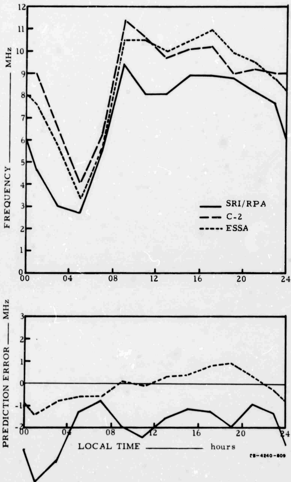
FIG. 2 COMPARISON OF OBSERVED AND PREDICTED MONTHLY MEDIAN f_oF_2 AND ERROR FUNCTION FOR FEBRUARY 1967
