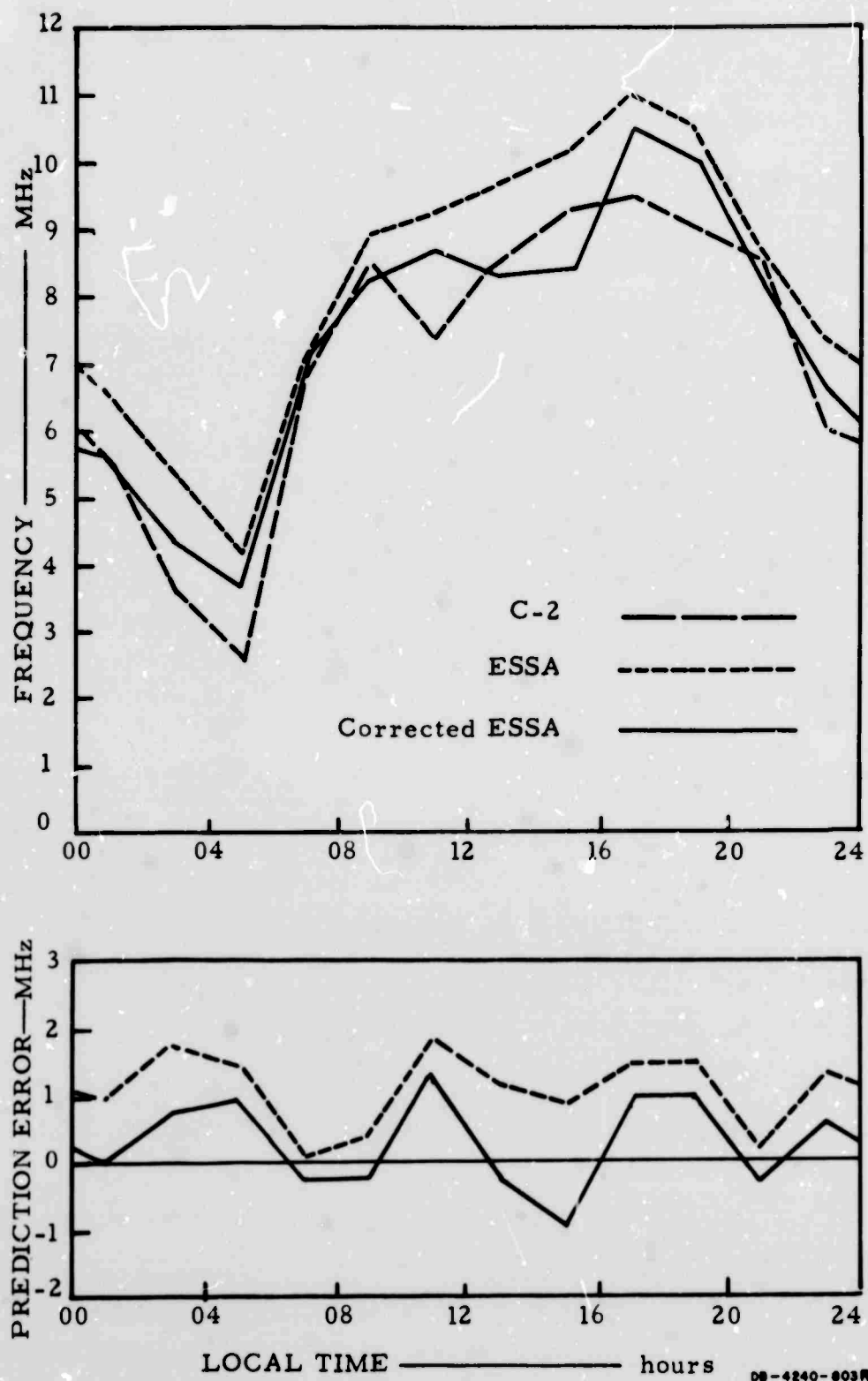
FIG. B-8 COMPARISON OF OBSERVED AND ESSA-PREDICTED MONTHLY MEDIAN f_oF_2 FOR AUGUST 1966
