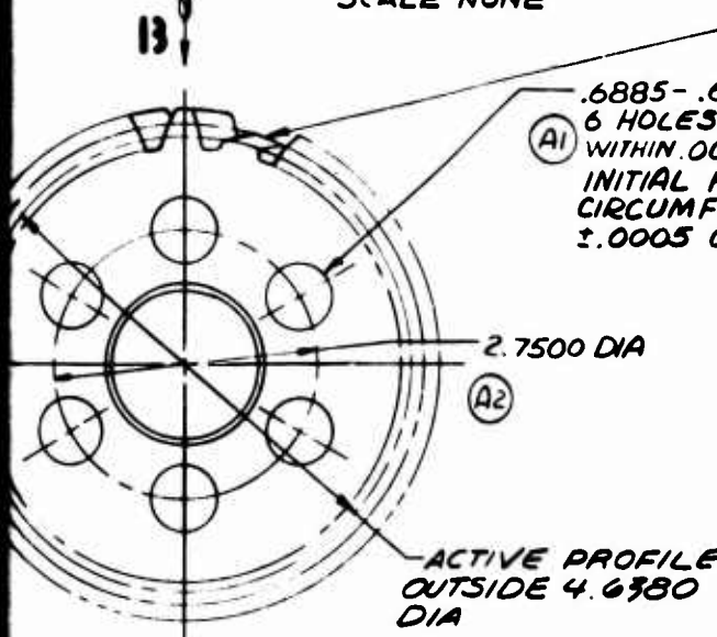
ENLARGED VIEW OF GEAR PROFILE SCALE NONE
