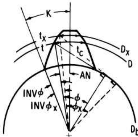
Figure 98. Arc and Chordal Tooth Thickness.
