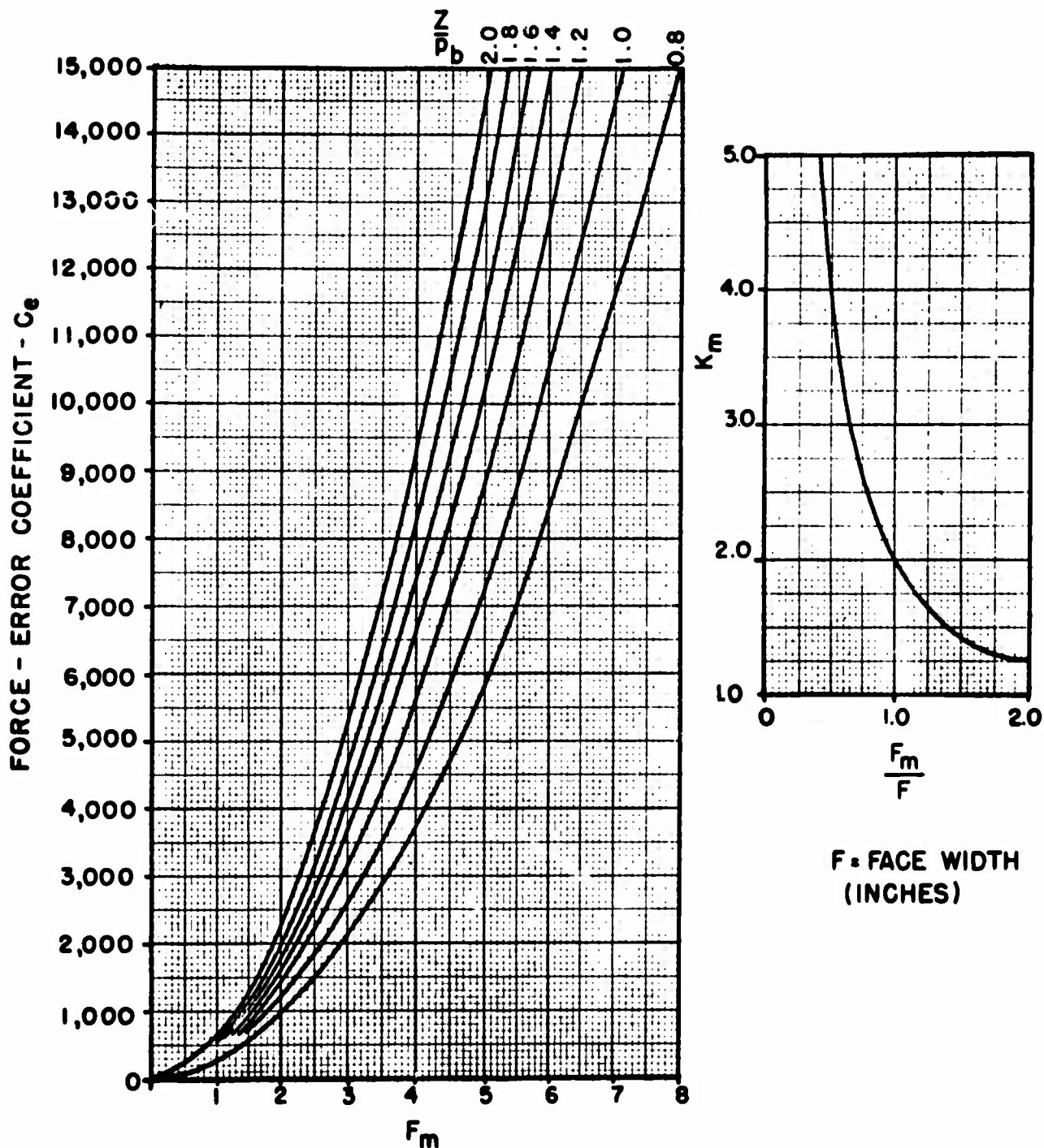
FIG. 5 HELICAL GEAR LOAD DISTRIBUTION FACTOR - K_m
