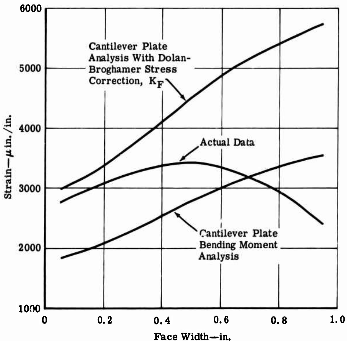
Figure 67. Strain Versus Face Width—EX-84119.
