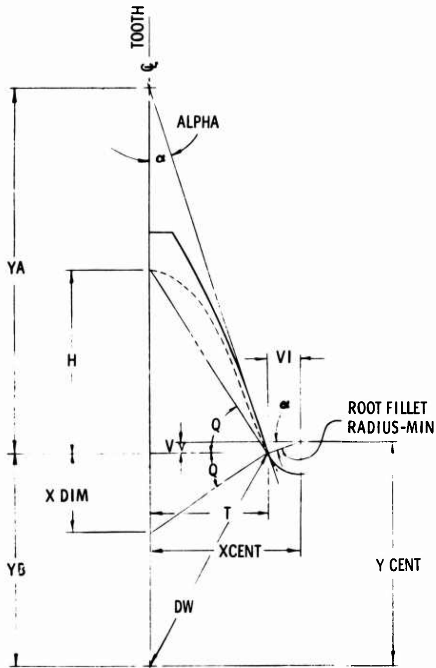
Figure 108. True Fillet Radius Inscribed Lewis Parabola.
