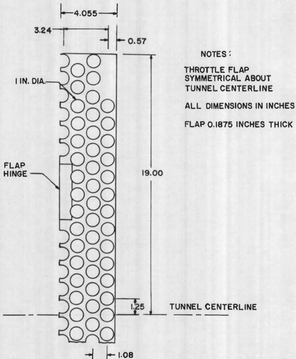
Fig. 4 Throttle Flaps
