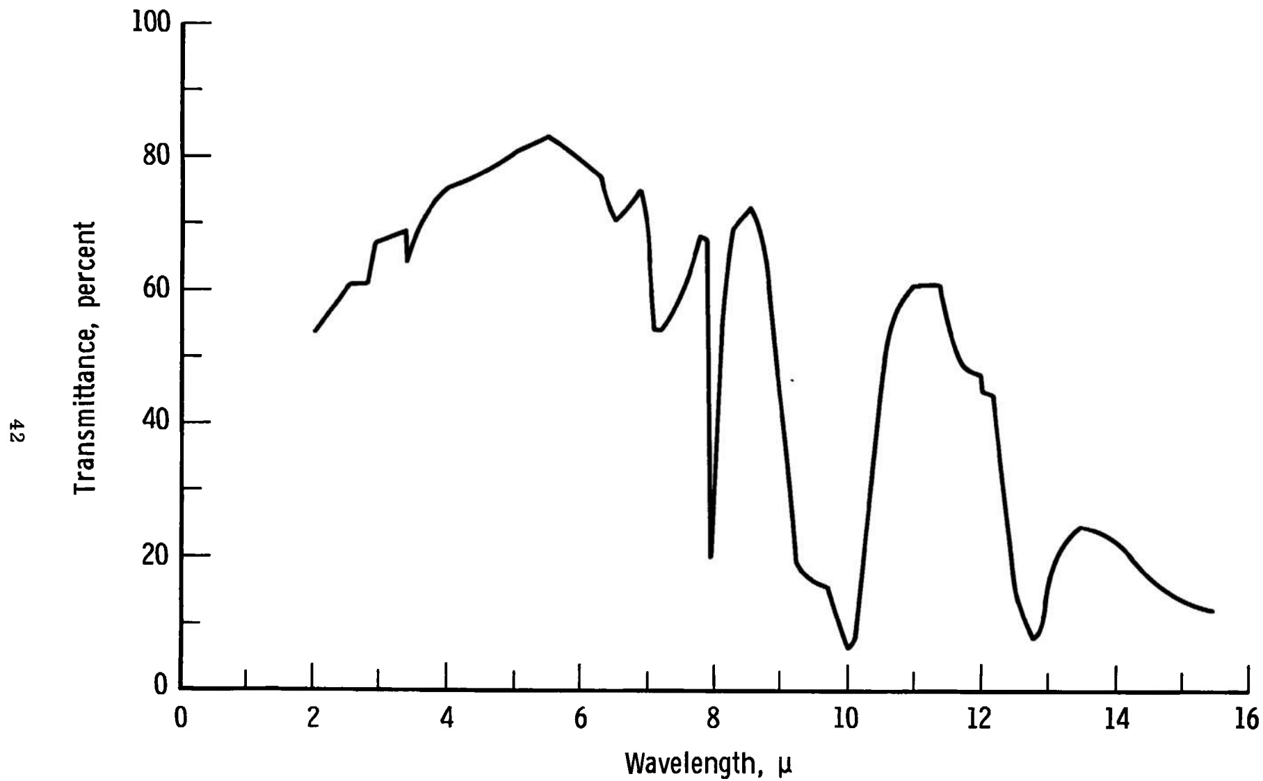
Fig. 17 Infrared Spectra of Electron Irradiated (Low Rate) Sample
