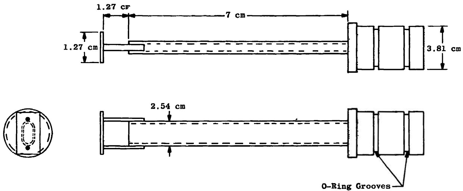
Fig. 3 Viewing Tube
