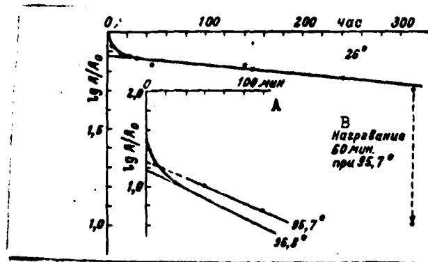
Fig. 2 Kinetics of inactivation of trypsin irradiated with ultraviolet light. c equals 1.0 mg/ml in 10^{-3} n.H 2 SO 4 . Residual activity after irradiation 35%. Line obtained at 96.8° corresponds to the inactivation of trypsin immediately following irradiation. Points at 95.7° correspond to enzyme inactivation after 314 hours of incubation of the irradiated solution at 26°. Key: A - minutes B - heating 60 minutes at 95.7°
