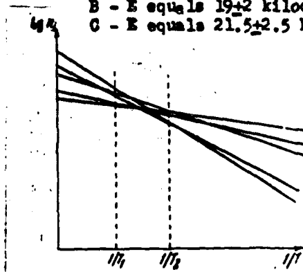
Fig. 4 Schematic diagram of the logarithm of the constant of the monomolecular reaction in enzyme inactivation as a function of 1/T .
