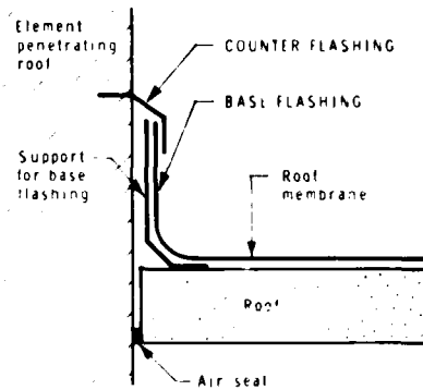
Figure 1 Basic flashings
