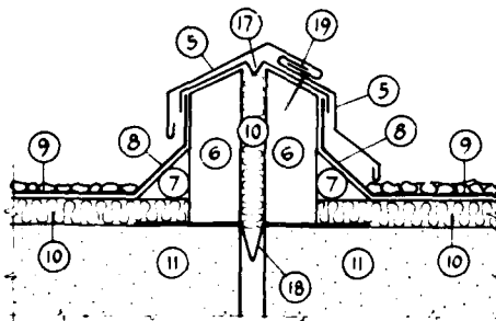
Figure 5 Movement joint
