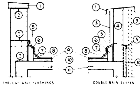
Figure 3 Parapet walls
