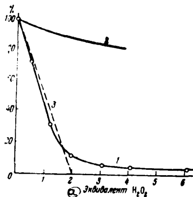
Figure 2. Action of H_2O_2 on semiquinone obtained from one equivalent of methylnaphthoquinone. 1 -- curve for experiment; 2 -- function computed on assumption of displacement of equilibrium III; 3 -- function computed according to scheme II. Ordinate axis -- quantity of free radicals as % of original amount. LEGEND: a) equivalents of H_2O_2 .
