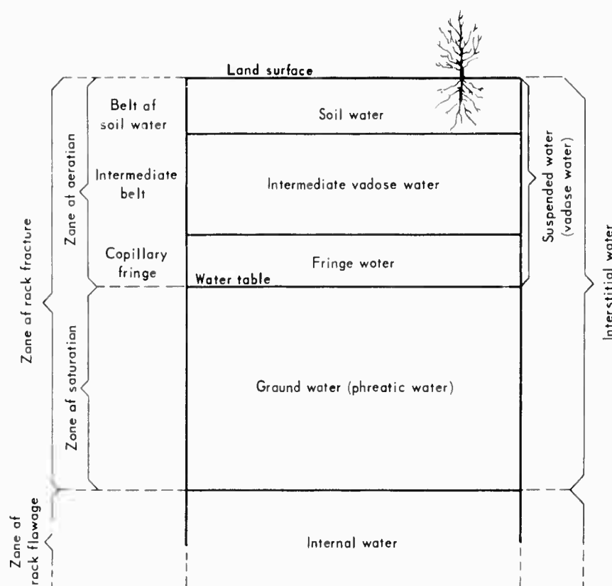
Fig. B8—Classic Divisions of Subsurface Water
