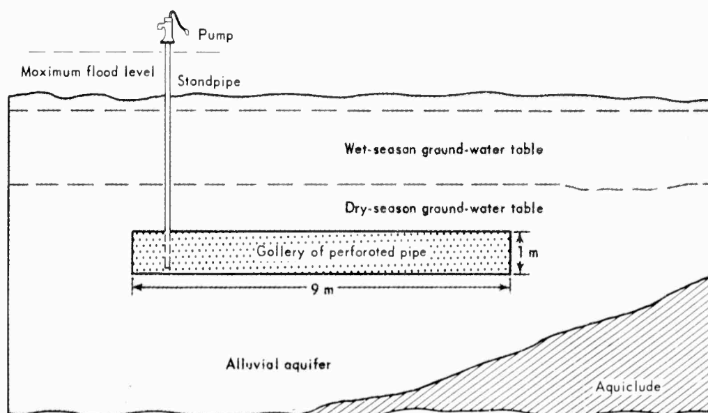
Fig. B9—Horizontal Infiltration Gallery
