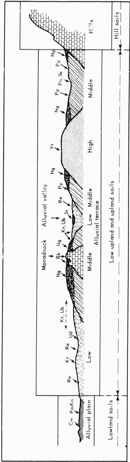
Fig. A10—Schematic Cross Section Indicating the Physiographic Position of the Principal Soil Series in Northeast Thailand
