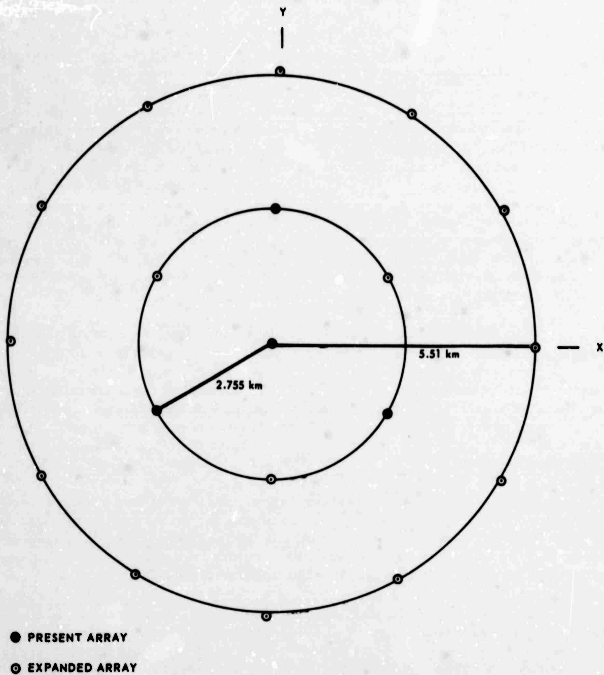
Figure 31 Expanded array at Station Inga Lehmann, Greenland
