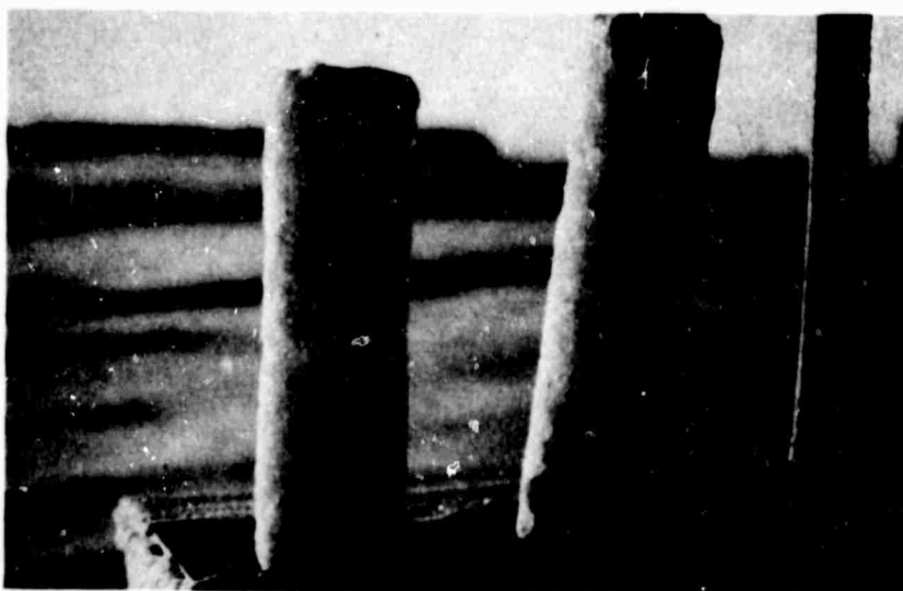
Sample of ice cores taken from one of the shallow holes
