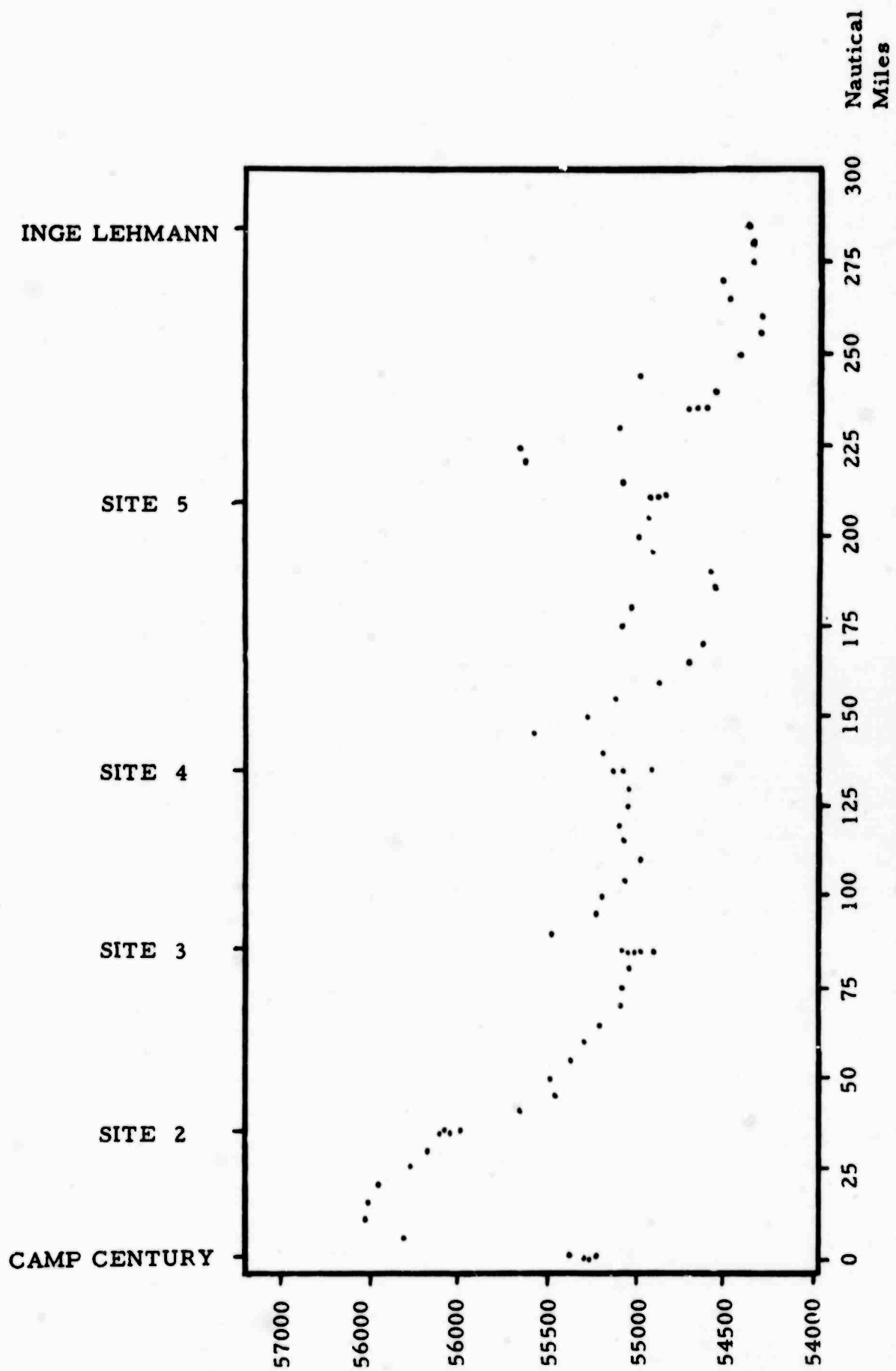
Fig. 51 Vertical Component of the Magnetic Field between Camp Century and Inge Lehmann
