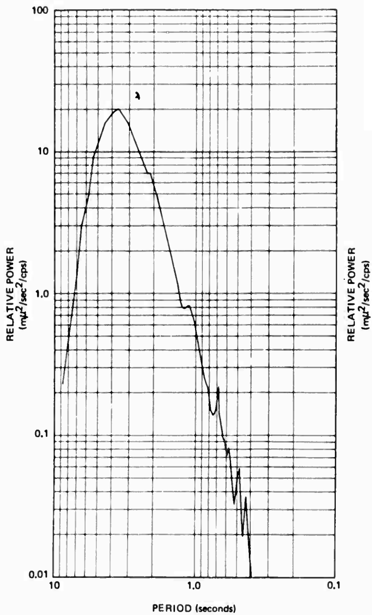
Figure 45 Project BLUE TREK site 4 power spectrum 17 August 1967
