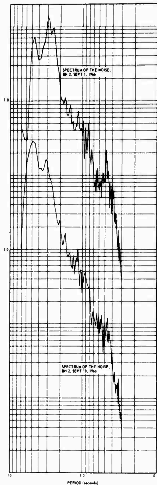
Figure 10 Nested spectra of the short-period noise recorded at Station Inge Lehmann, Greenland
