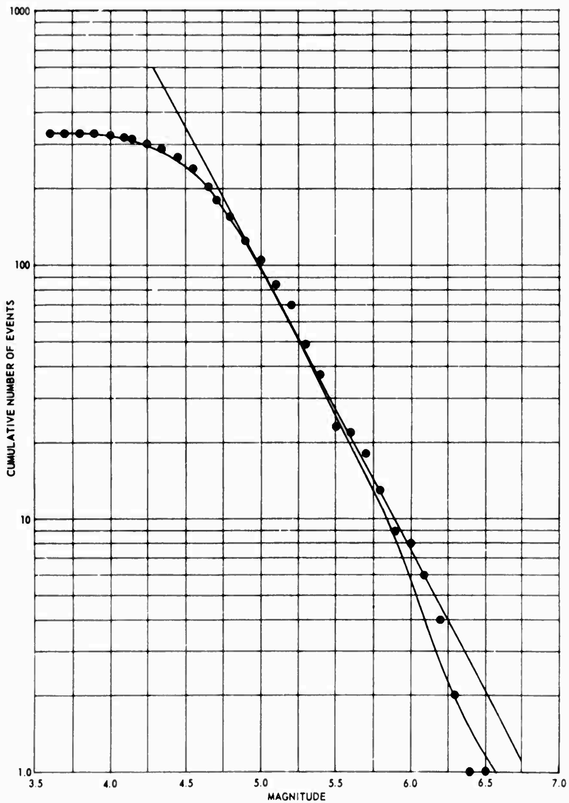
Figure 22 Cumulative probability of detection curve for Station Inge Lehmann, Greenland
