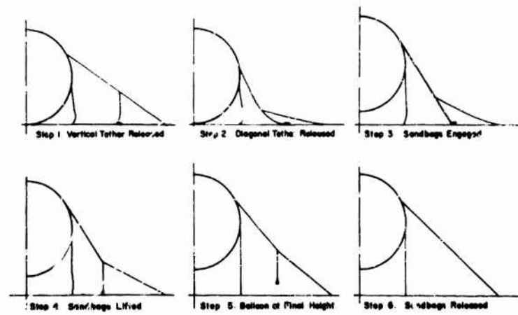
Figure 9. 110-ft Balloon Deployment Sequence
