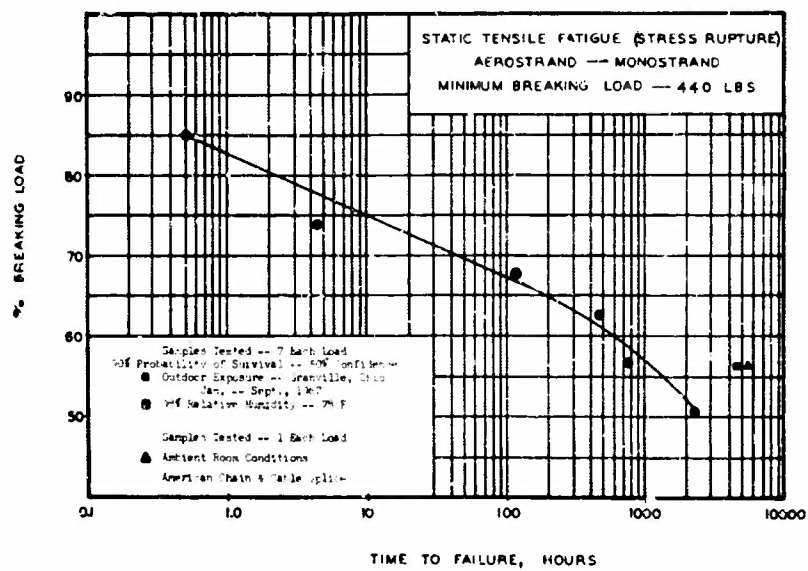
Figure 4. Static Tensile Fatigue (Stress Rupture) Aerostrand-Monostand
