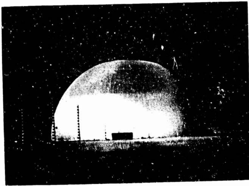
Figure 1. 125-ft Diameter Hemisphere During Filling Operation
