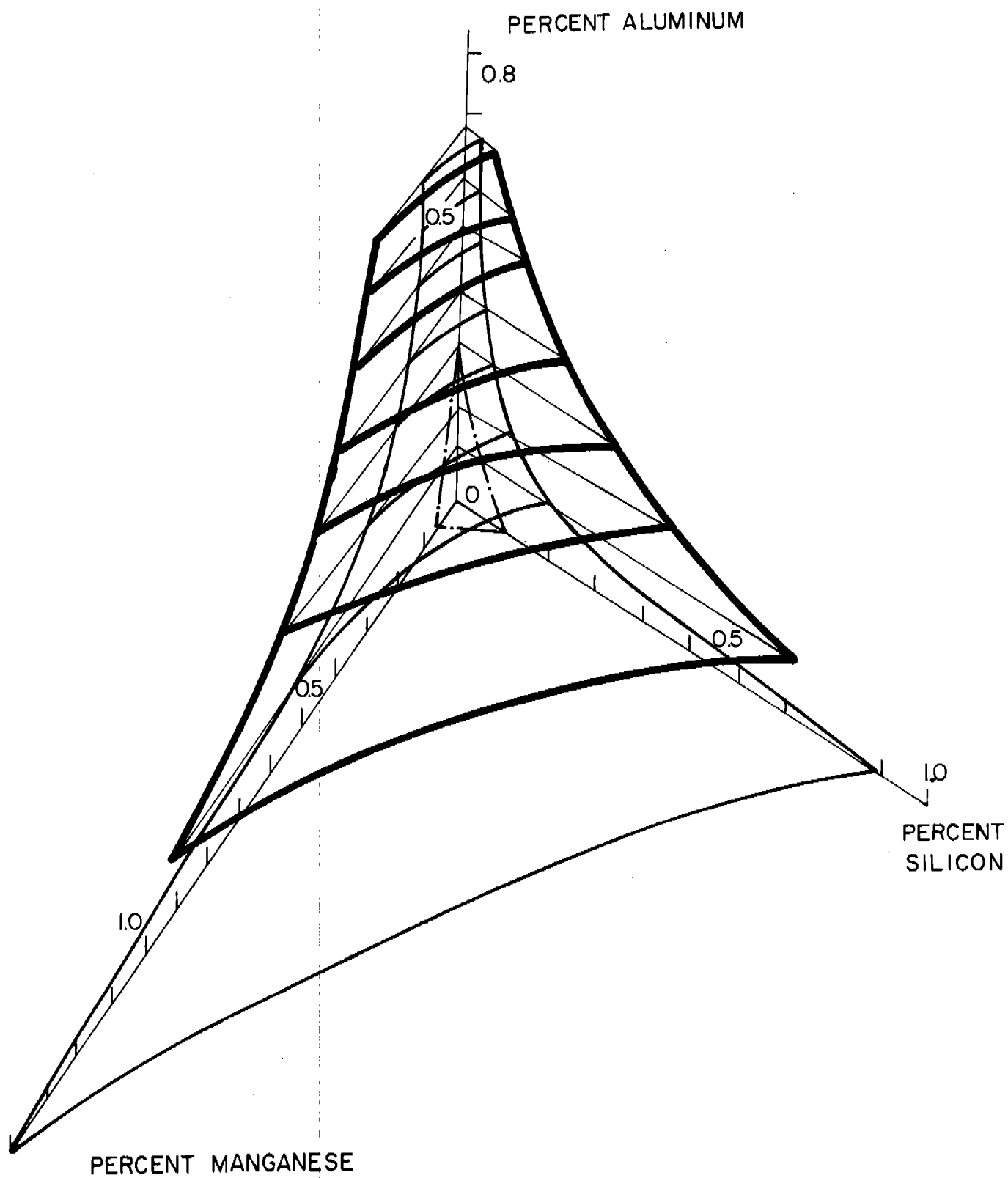
Figure 17: Type of sulfide inclusions versus Al,Mn,and Si additions. AISI 4330 - 0.1% S specimens solidified at 40°C/min.
