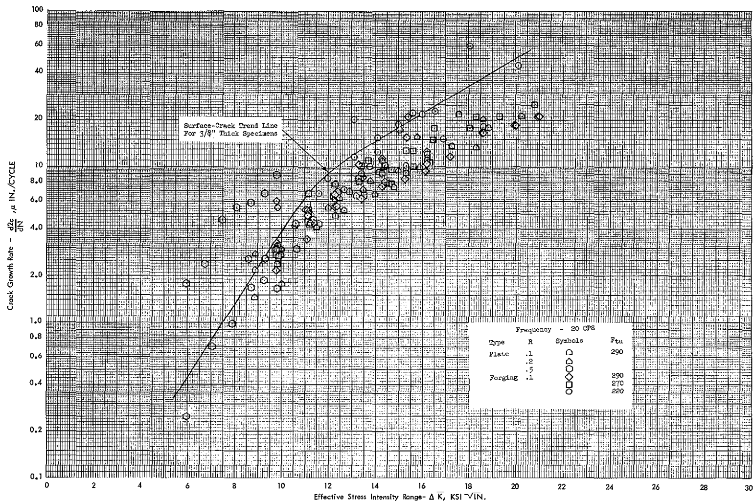
Figure 92 Cyclic Cracking Rate vs Effective Stress Intensity Range for 3/4" Thick 300 M Steel Plate (F tu 290 KSI) and Forging (F tu 290, 270, 220 KSI) Surface-Crack Specimens in Moist Air Environment.
