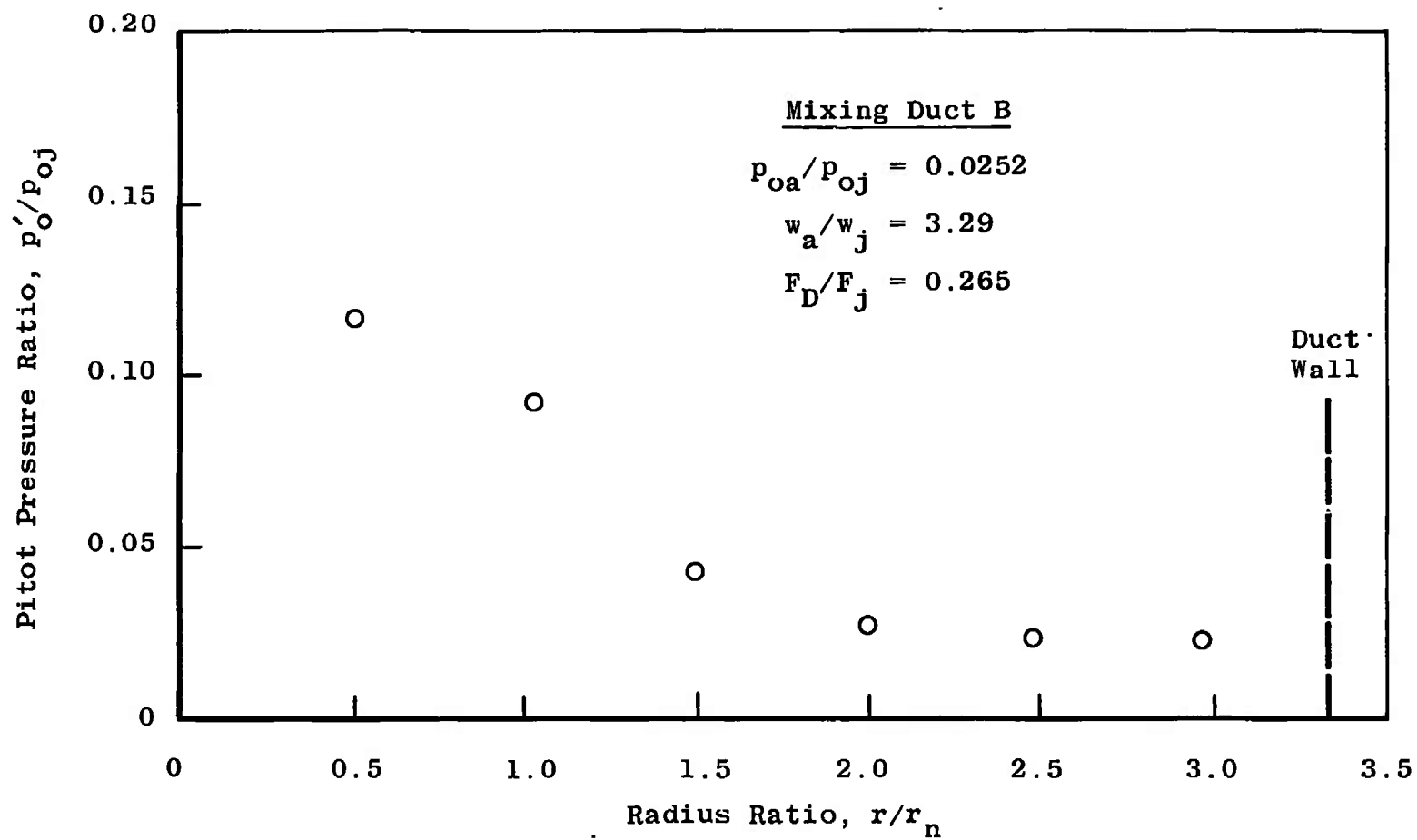
e. Test Condition 6 Fig. 10 Concluded
