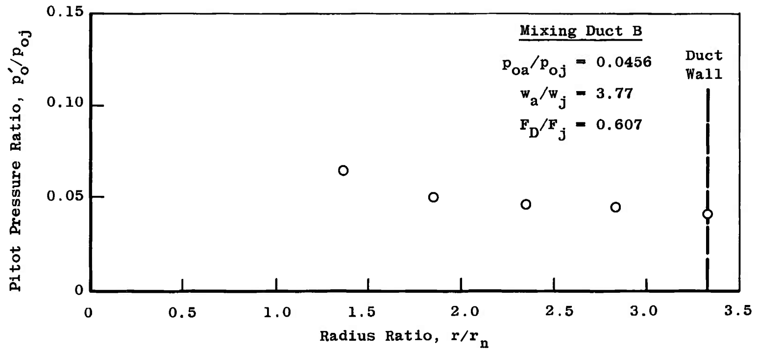
c. Test Condition 10 Fig. 13 Continued
