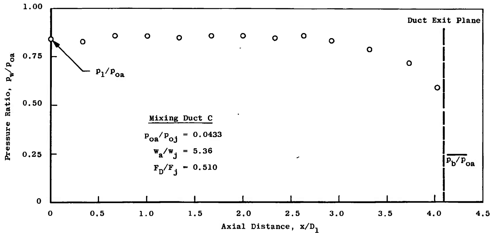
a. Test Condition 1 Fig. 9 Duct-Wall Pressure, Downstream Choking Mode
