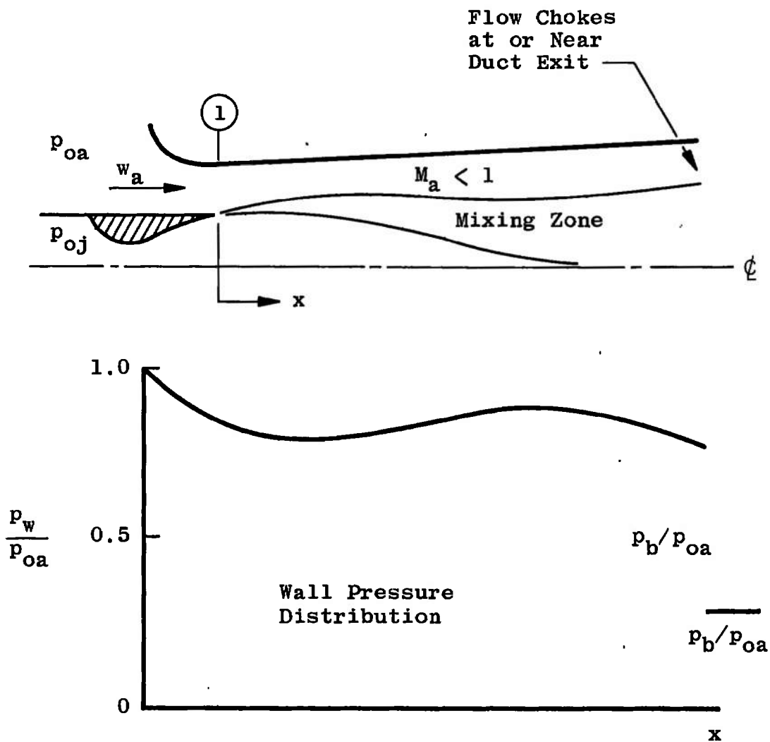
c. Downstream Choking Mode Fig. 2 Concluded
