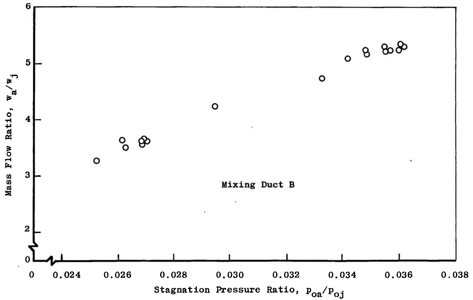
Fig. 7 Mass Flow Ratio, Downstream Choking Mode
