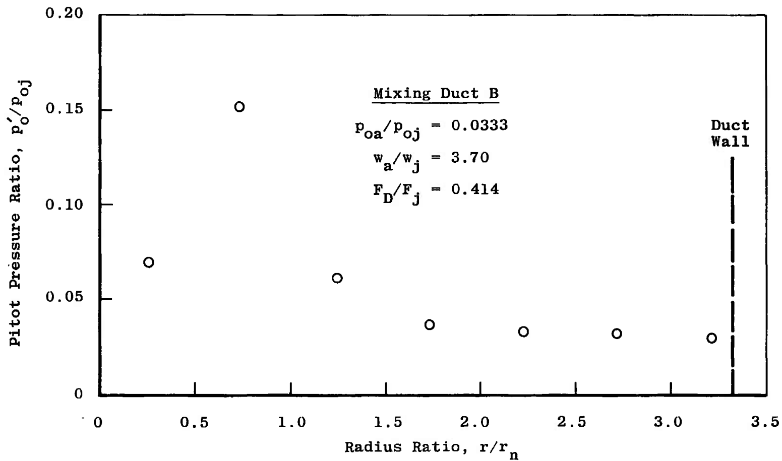
e. Test Condition 13 Fig. 13 Concluded
