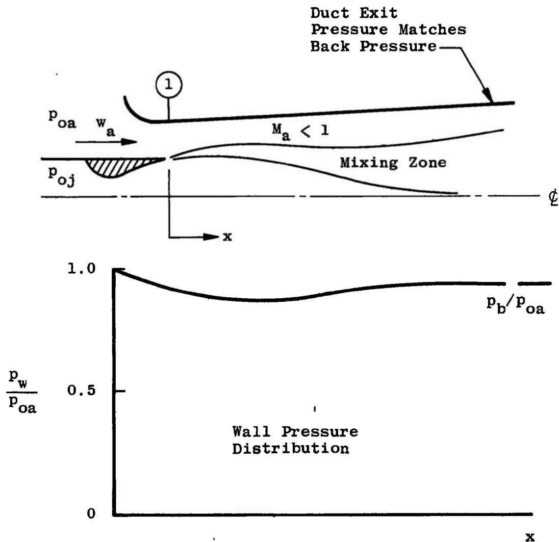
b. Back Pressure Dependent Mode Fig. 2 Continued
