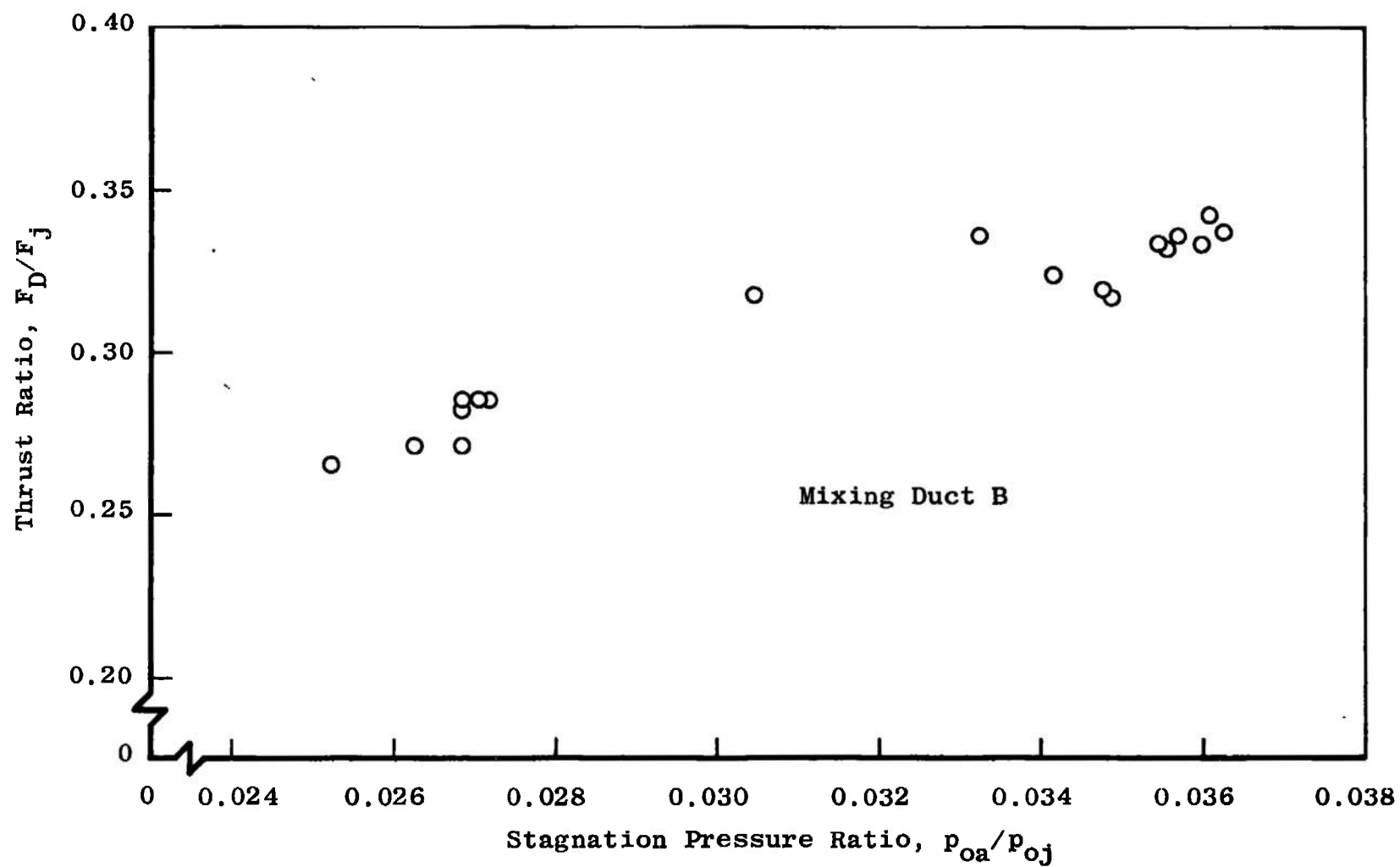
Fig. 8 Mixing Duct Thrust, Downstream Choking Mode
