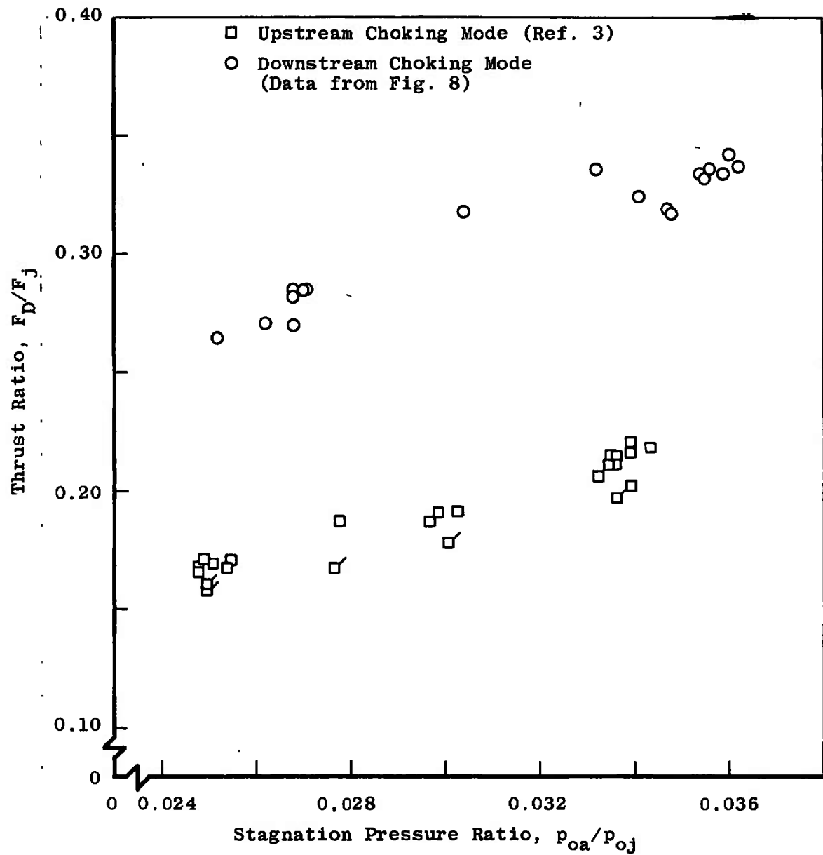
b. Thrust Ratio Fig. 15 Concluded
