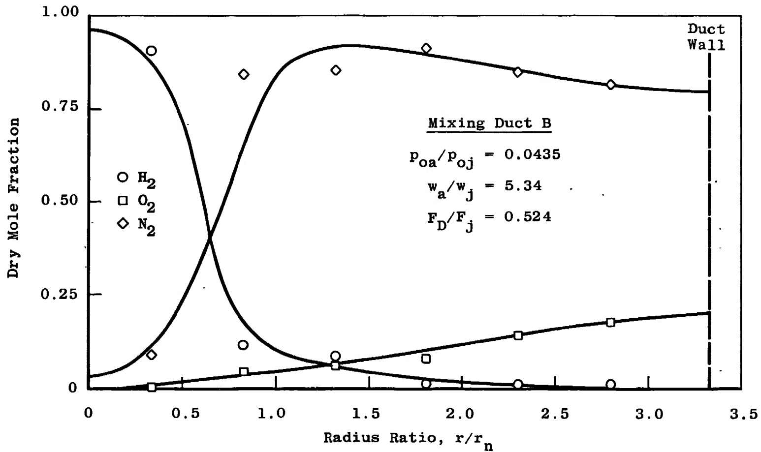
b. Test Condition 9 Fig. 14 Continued
