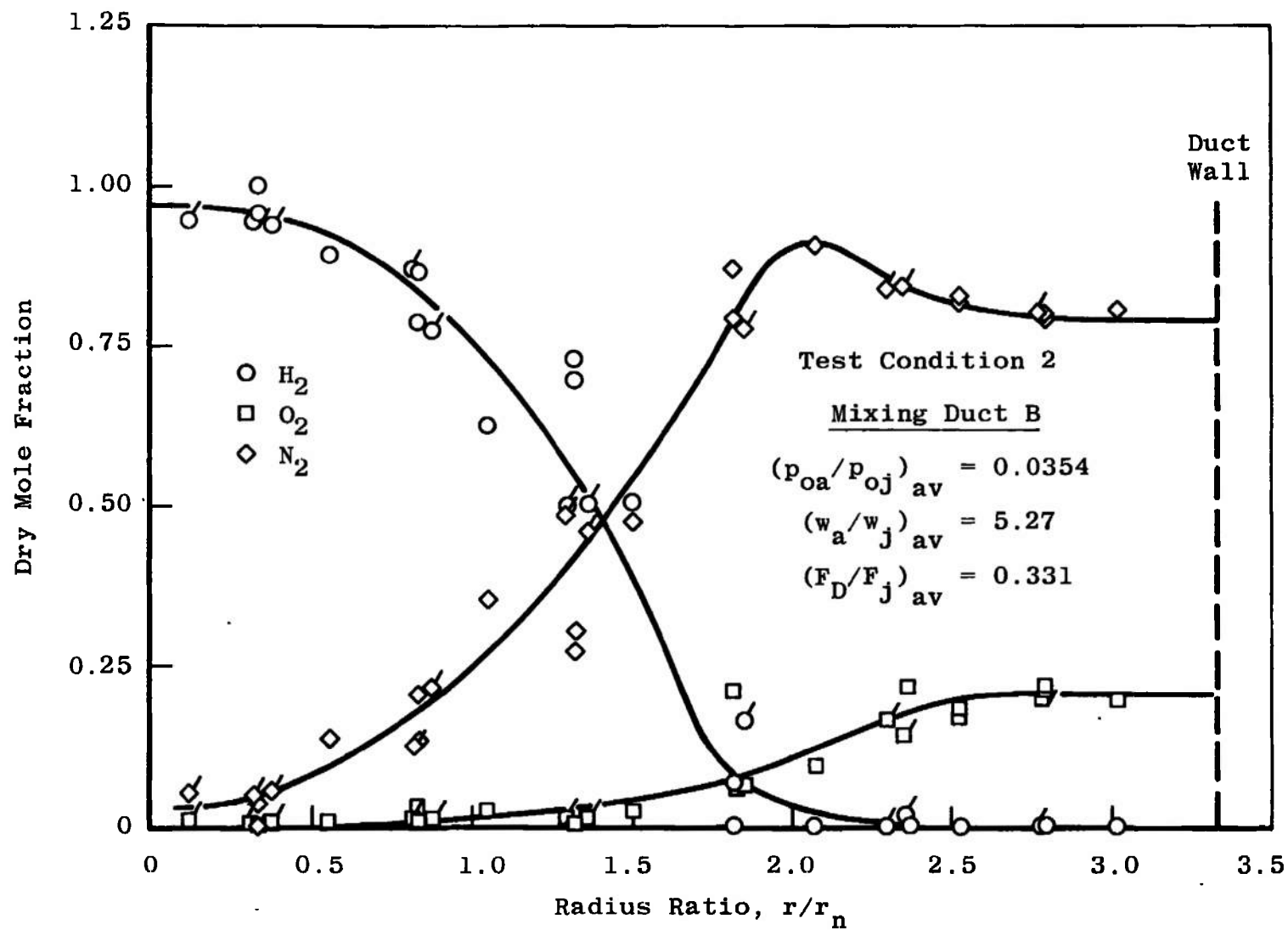
Fig. 11 Composition at Duct Exit, Downstream Choking Mode
