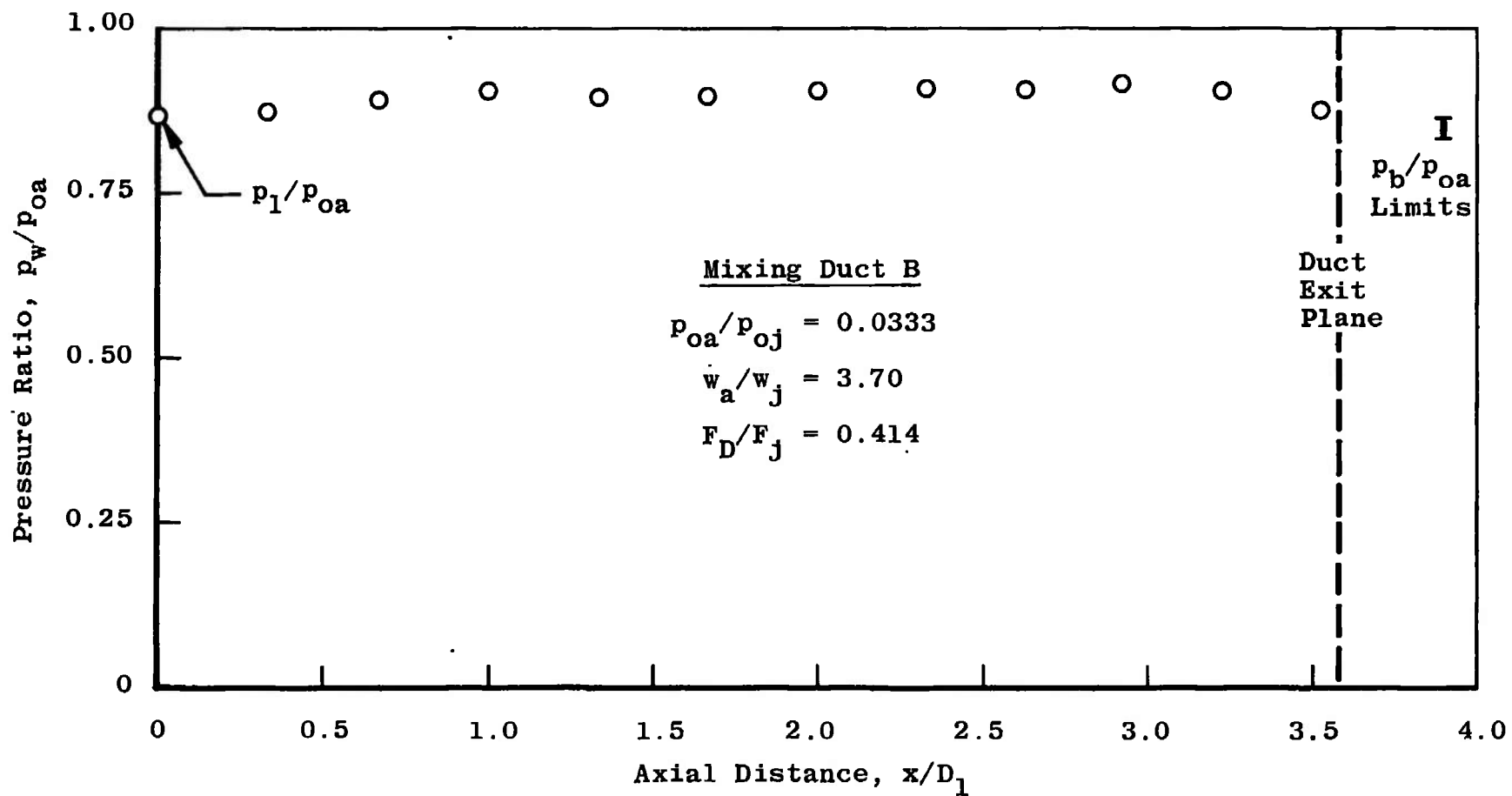
g. Test Condition 13 Fig. 12 Concluded
