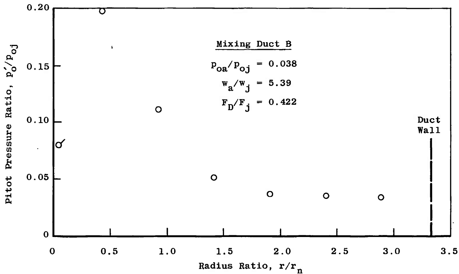
Fig. 13 Pitot Pressure at Duct Exit, Back Pressure Dependent Mode
