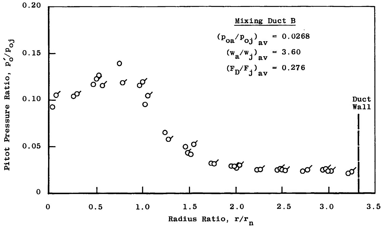
b. Test Condition 3 Fig. 10 Continued
