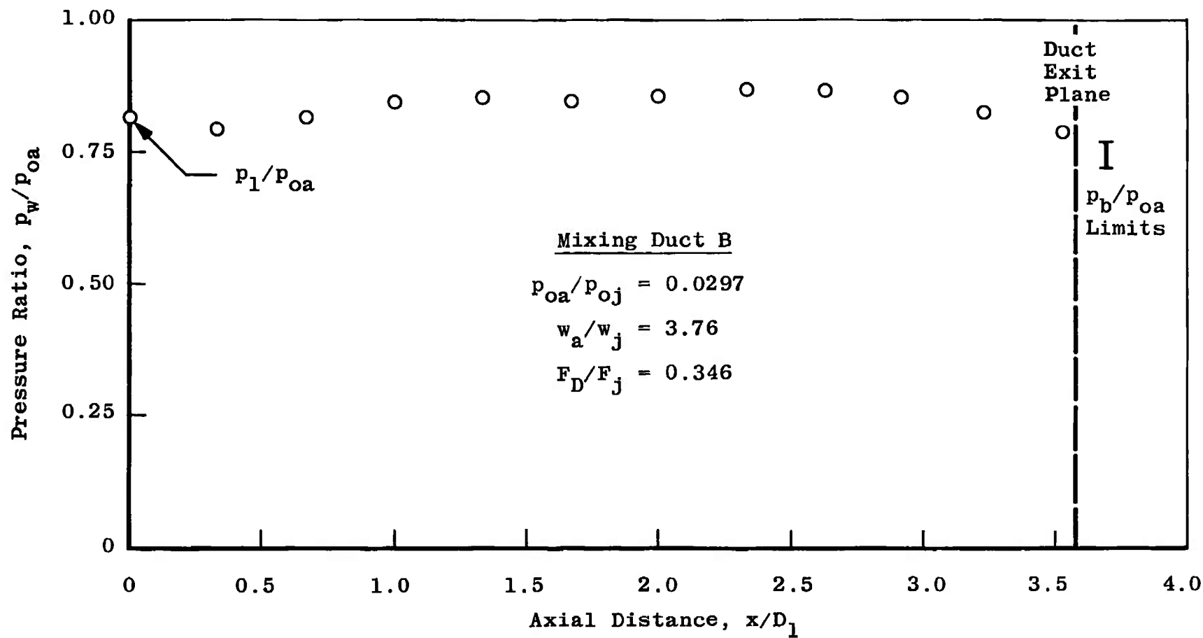
f. Test Condition 12 Fig. 12 Continued
