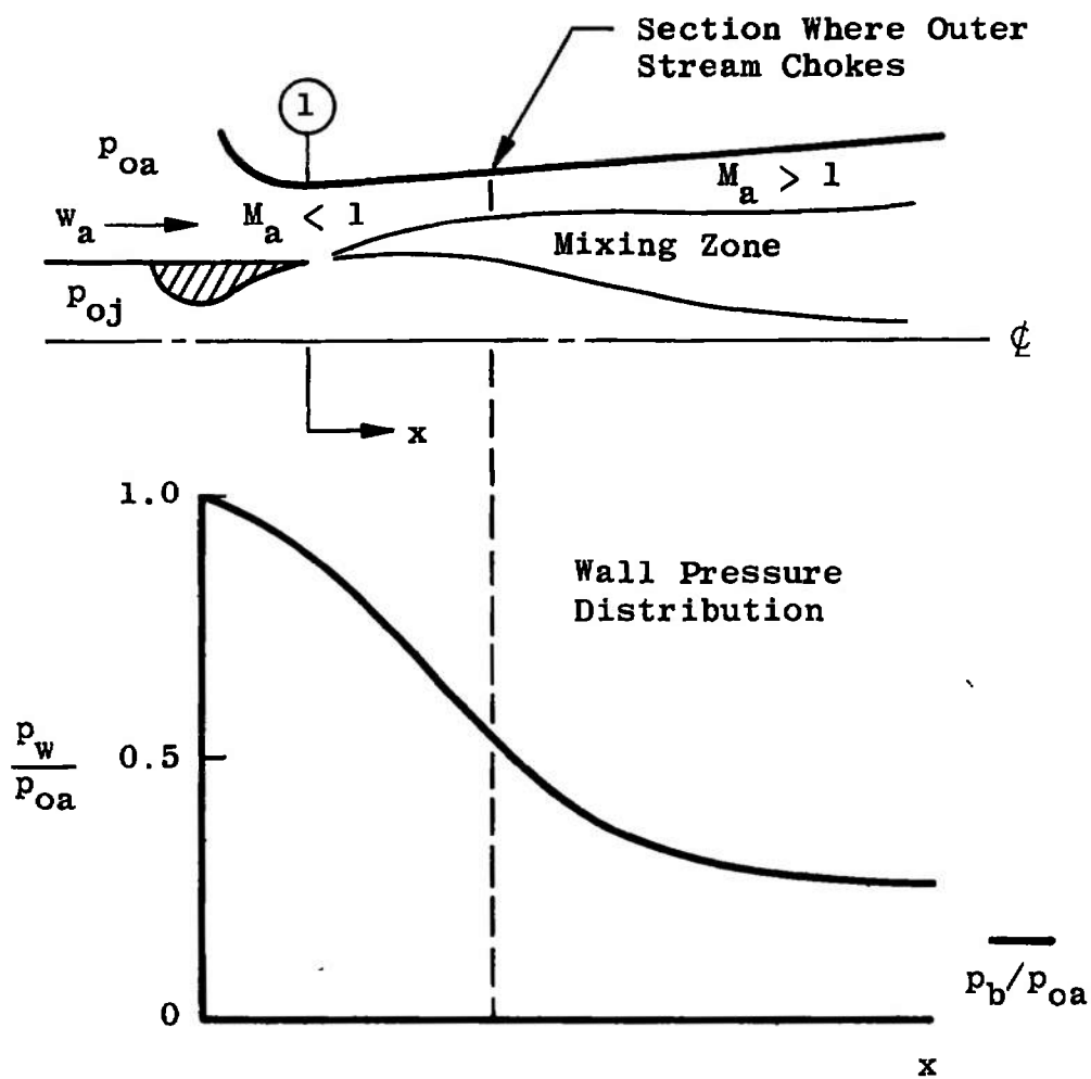
Fig. 2 Operational Modes of a Ducted Mixing System
