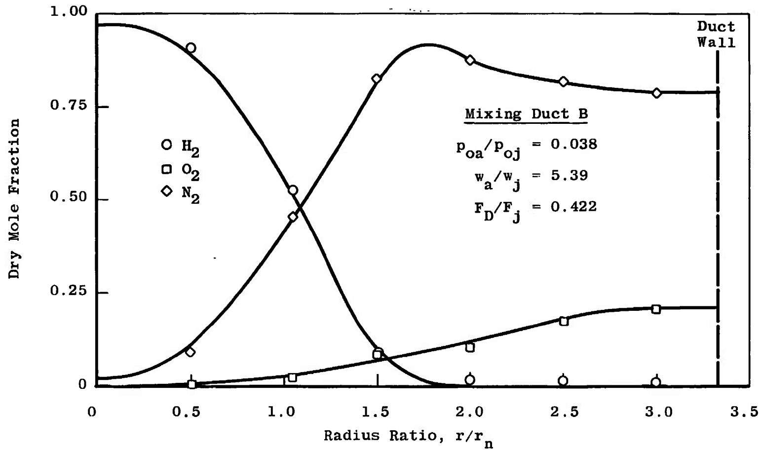
Fig. 14 Composition at Duct Exit, Downstream Choking Mode
