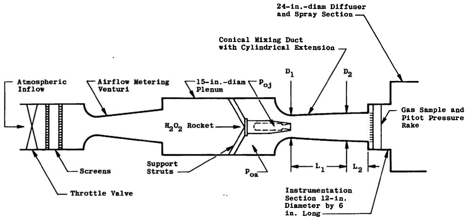
Fig. 3 Schematic of Propulsion Research Cell (R-1B)
