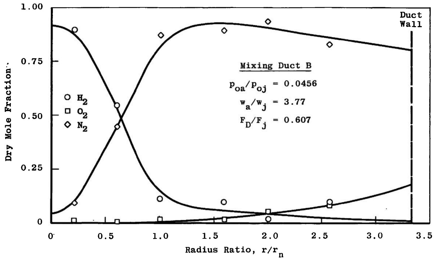
c. Test Condition 10 Fig. 14 Concluded
