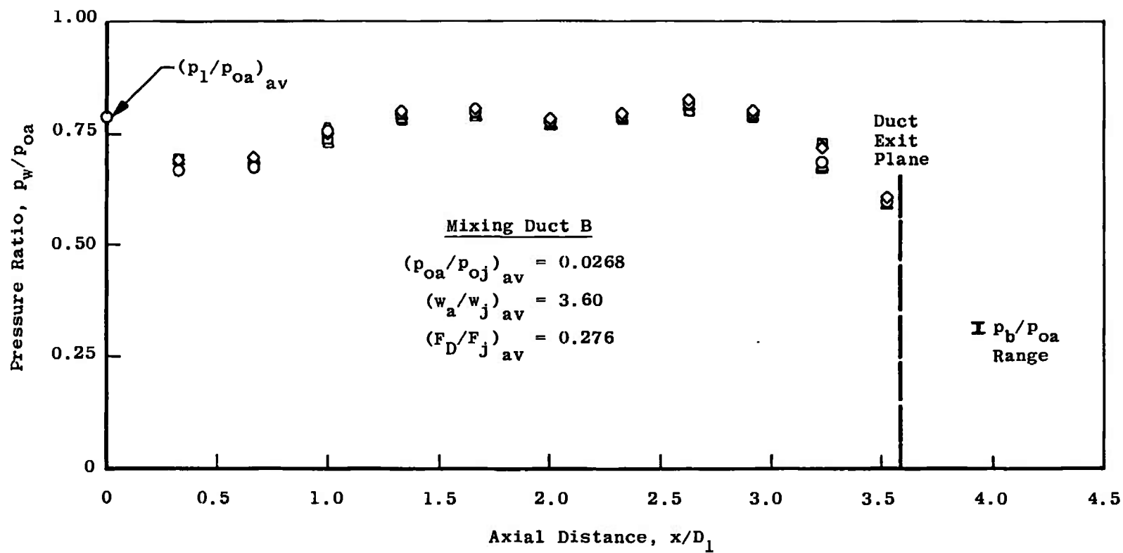
c. Test Condition 3 Fig. 9 Continued
