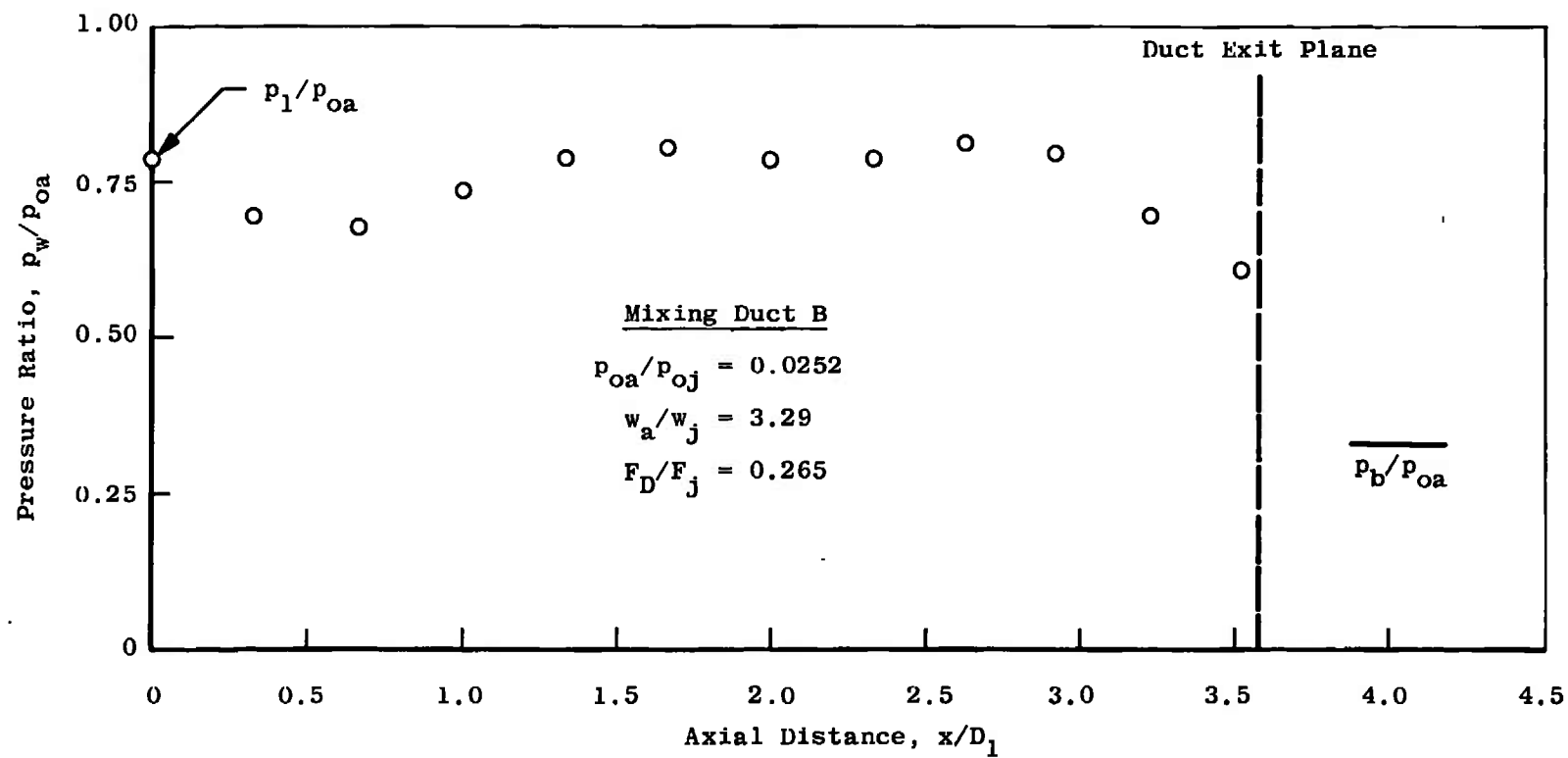
f. Test Condition 6 Fig. 9 Concluded
