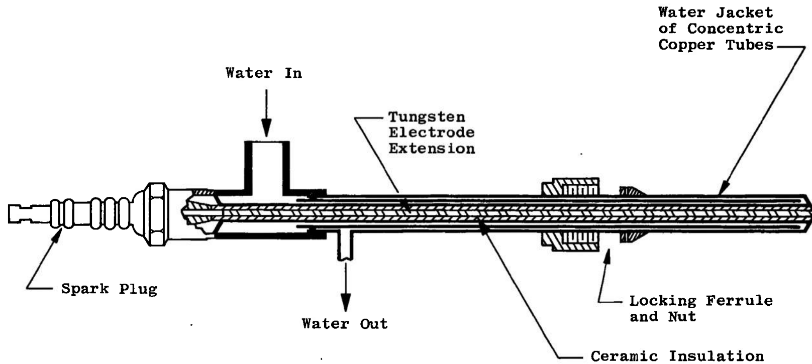
Fig. 5 Details of Water-Cooled Spark Plug
