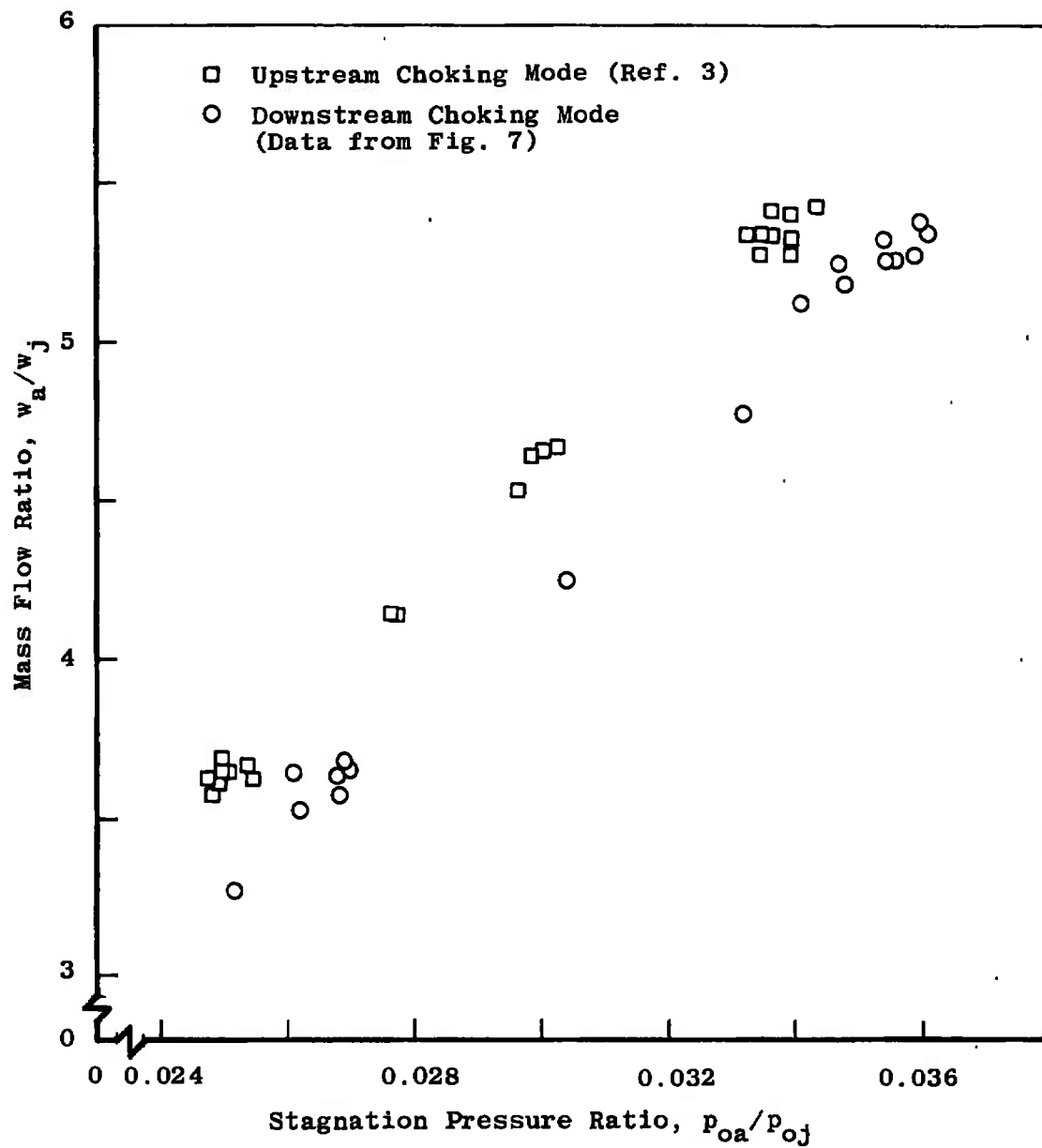
Fig. 15 Comparison of Upstream Choking and Downstream Choking Modes
