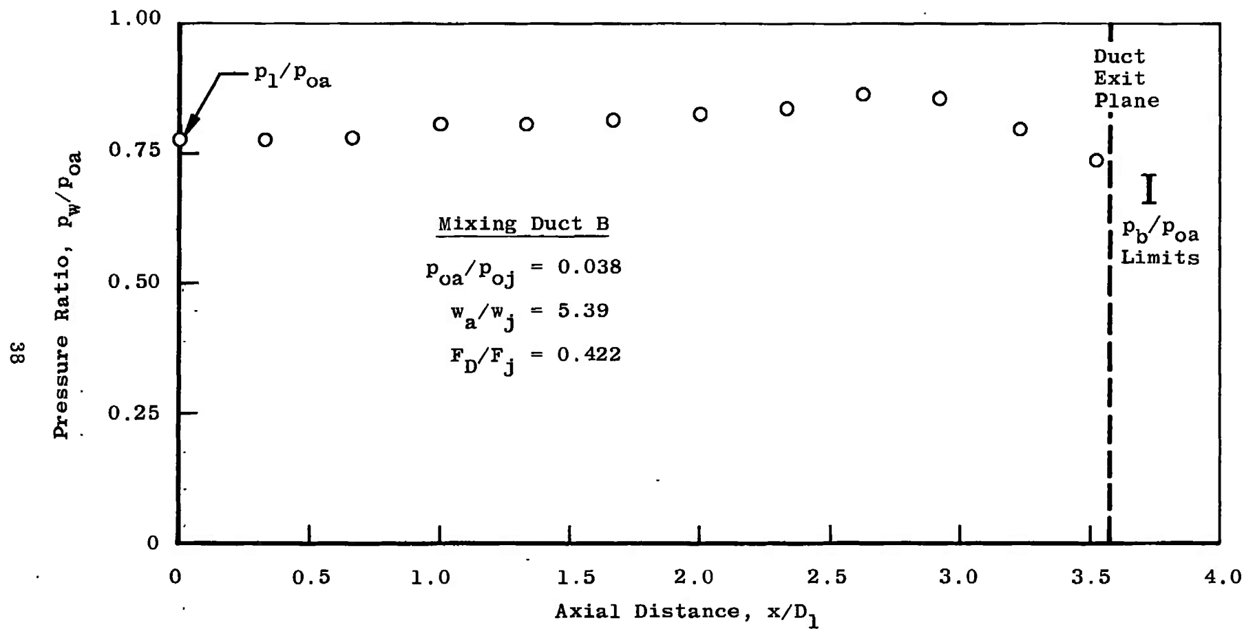
b. Test Condition 8 Fig. 12 Continued
