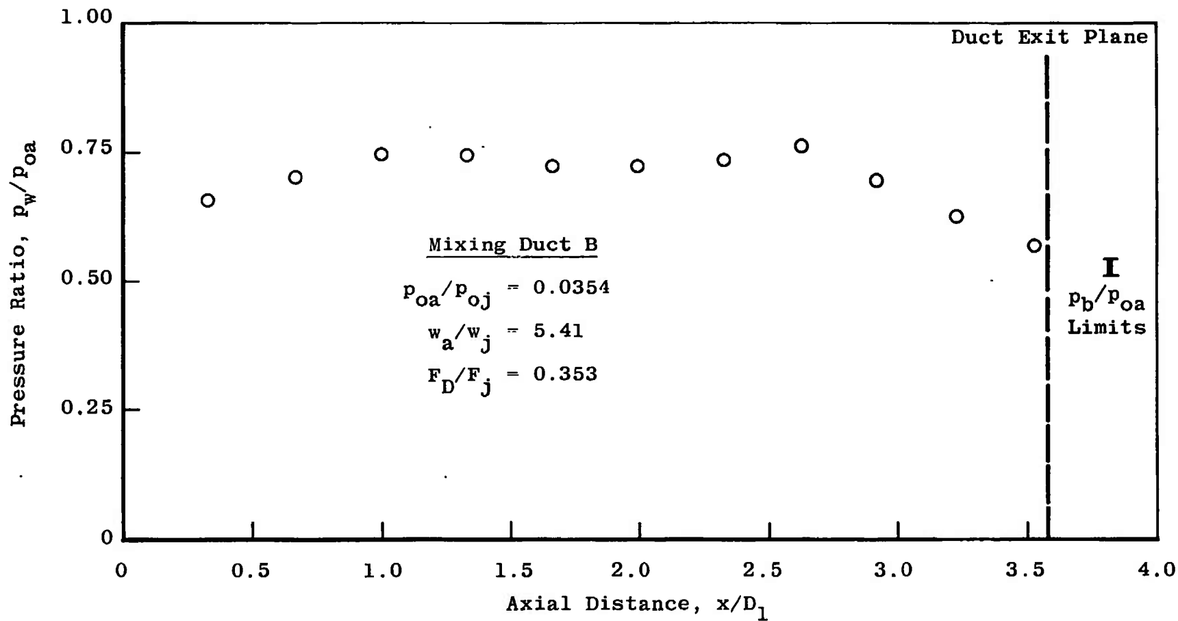
a. Test Condition 7 Fig. 12 Duct Wall Pressure, Back Pressure Dependent Mode
