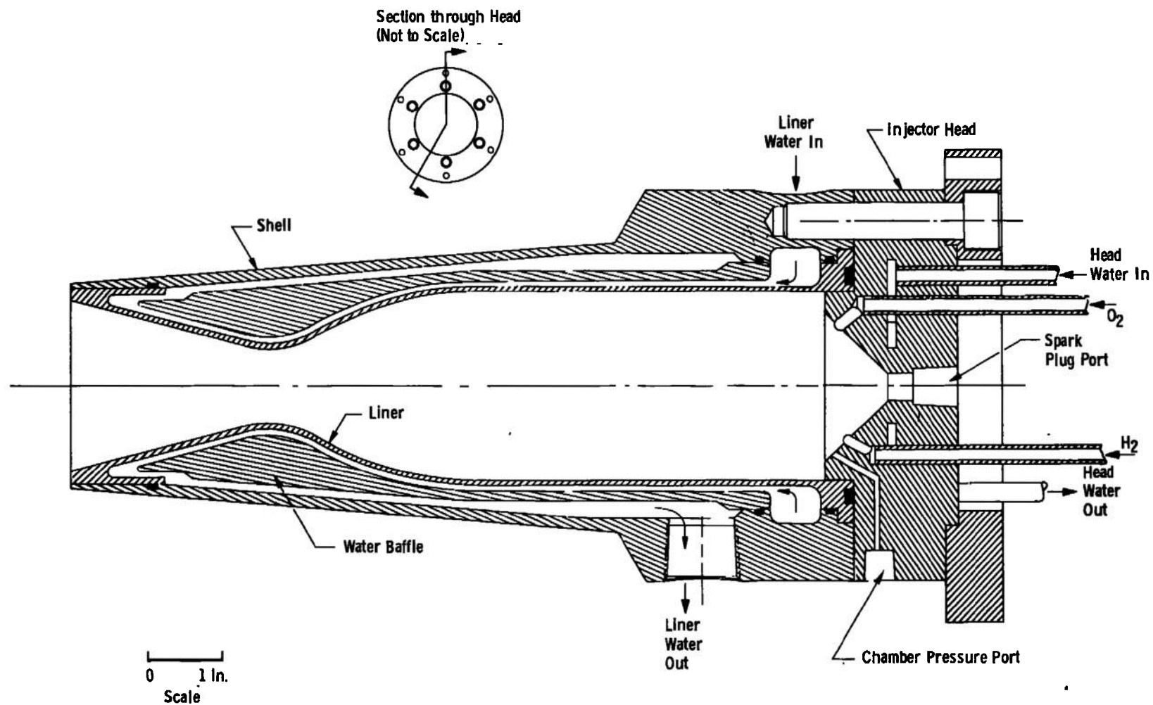
Fig. 4 Rocket Engine
