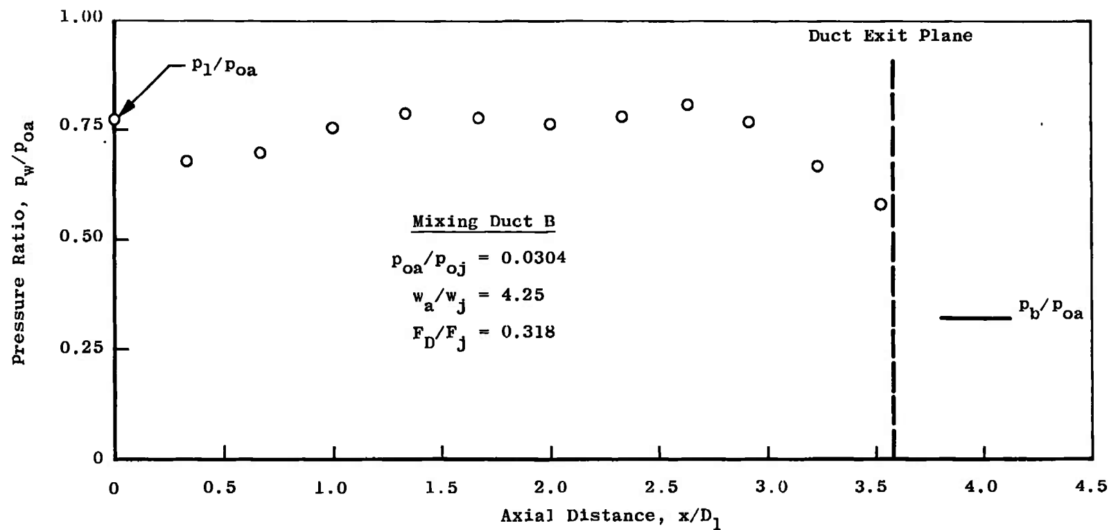
d. Test Condition 4 Fig. 9 Continued
