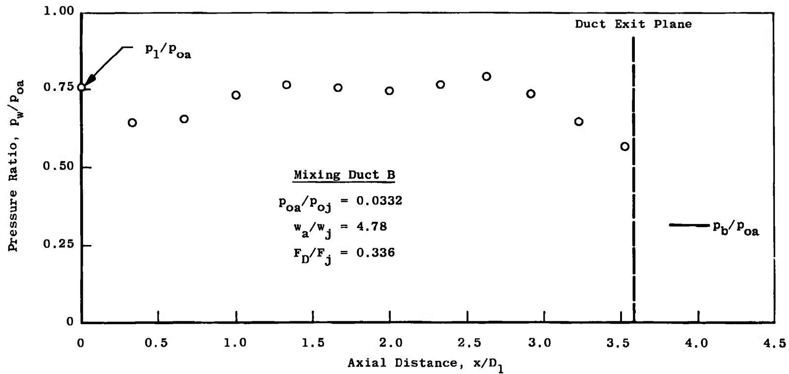
e. Test Condition 5 Fig. 9 Continued
