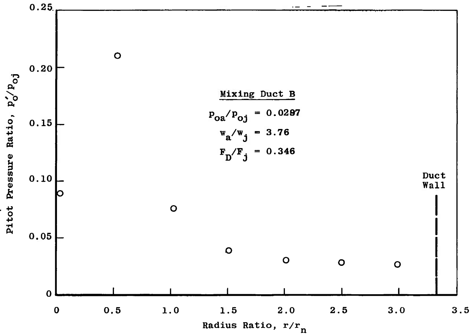
d. Test Condition 12 Fig. 13 Continued
