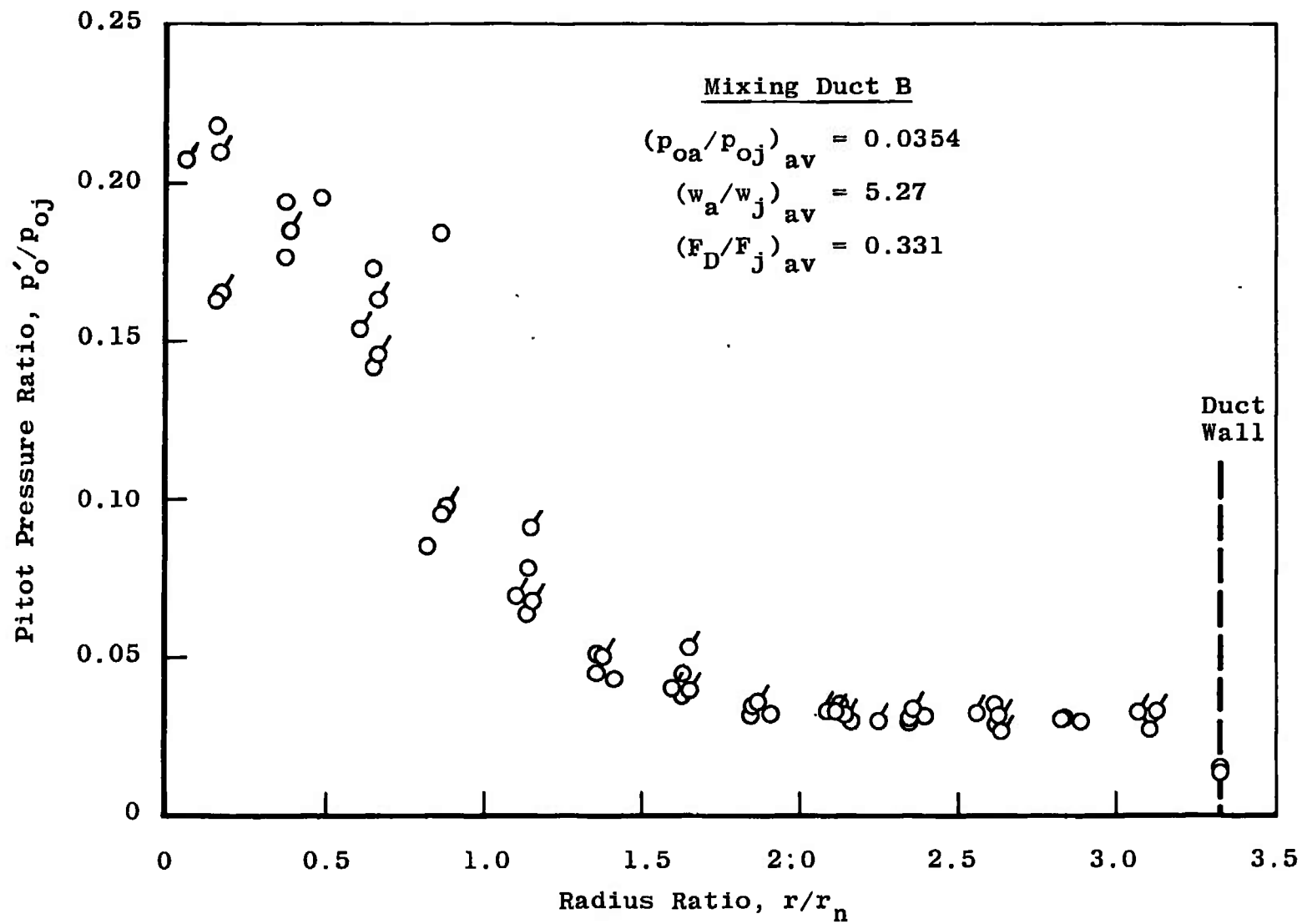
Fig. 10 Pitot Pressure at Duct Exit, Downstream Choking Mode
