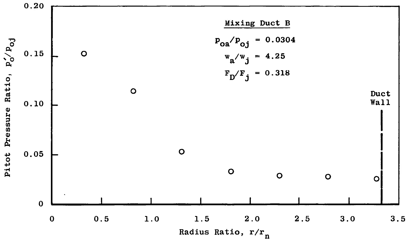
c. Test Condition 4 Fig. 10 Continued
