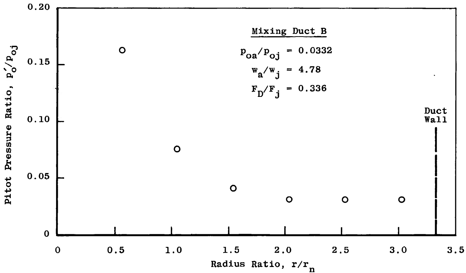
d. Test Condition 5 Fig. 10 Continued
