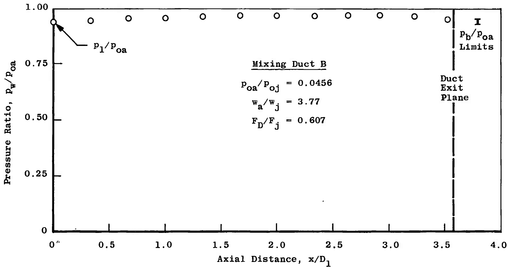
d. Test Condition 10 Fig. 12 Continued
