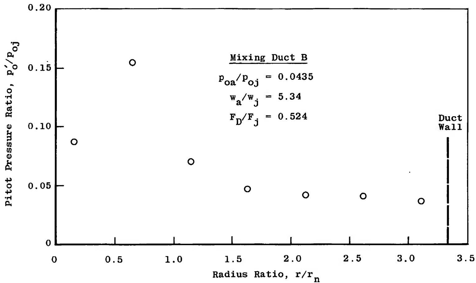
b. Test Condition 9 Fig. 13 Continued
