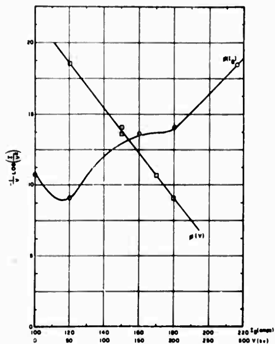
Figure 9-7. 1/V \log I/V^2 as a Function of V and Magnetizing Current (2 cm Gap, Test No. 3) (290 amp \approx 250 Gauss)
