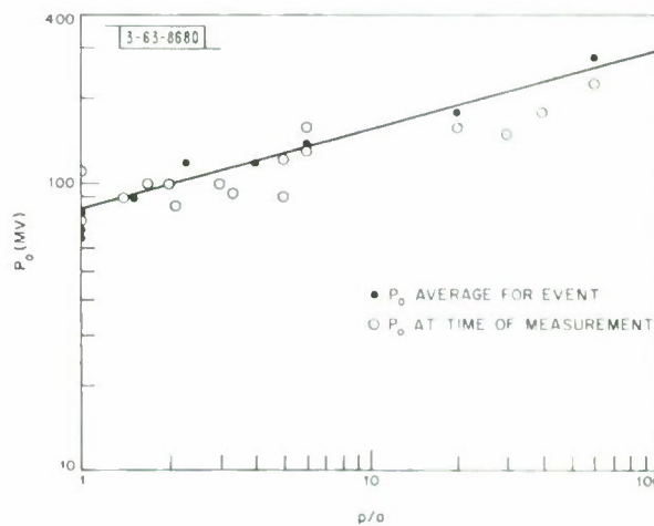
Fig. 17. Proton-to-alpha-particle ratio as a function of characteristic rigidity P_0 (taken from W. R. Webber, Ref. 65, Fig. 3).
