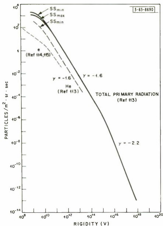
Fig. 27. Integral spectrum of galactic cosmic rays (total primary radiation and helium nuclei from W.R. Webber, Ref. 113, electrons from C.J. Waddington, Ref. 114 and P. Meyer, Ref. 115).
